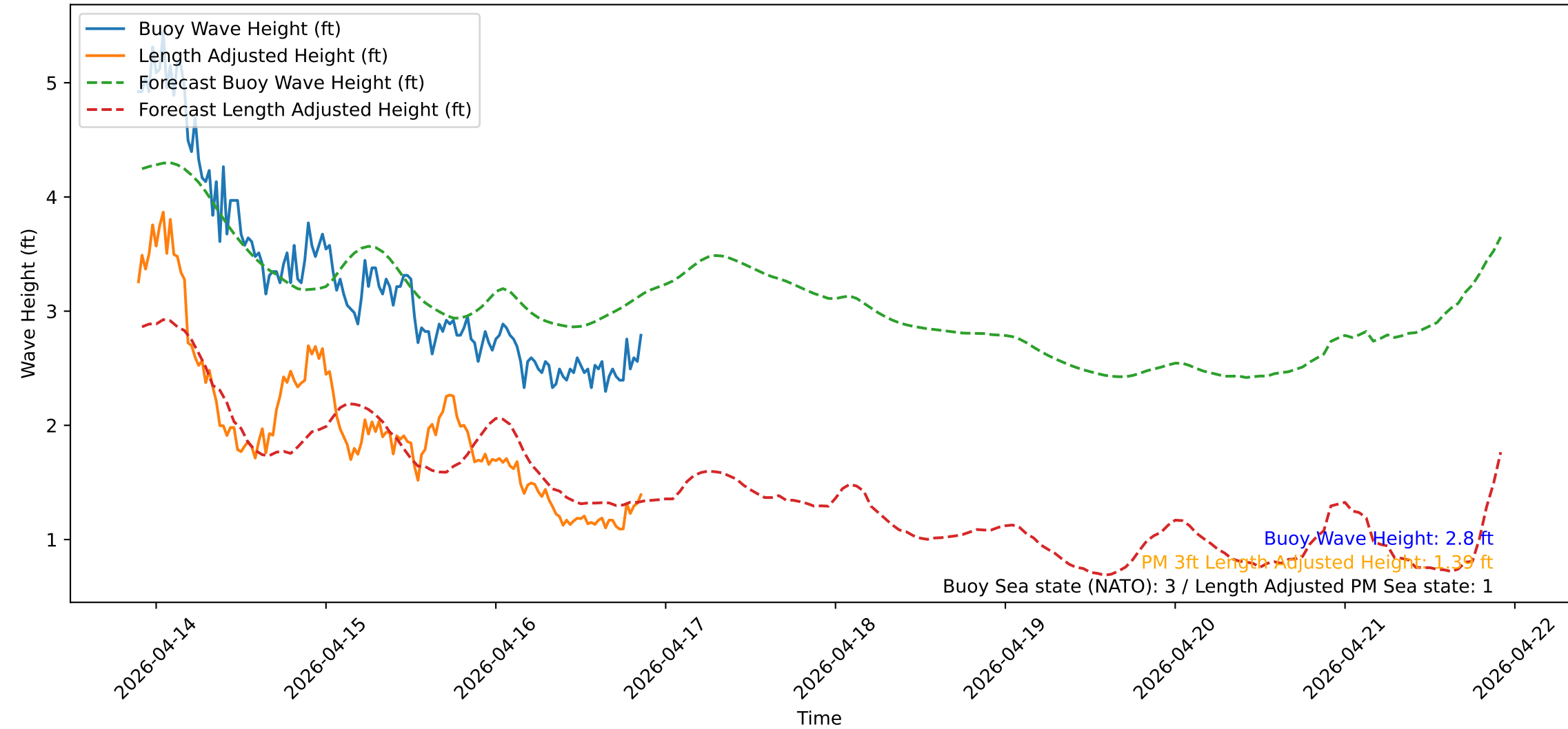
Wave Heights over Time for Oceanside Harbor at 2026-04-16 21:30:31
