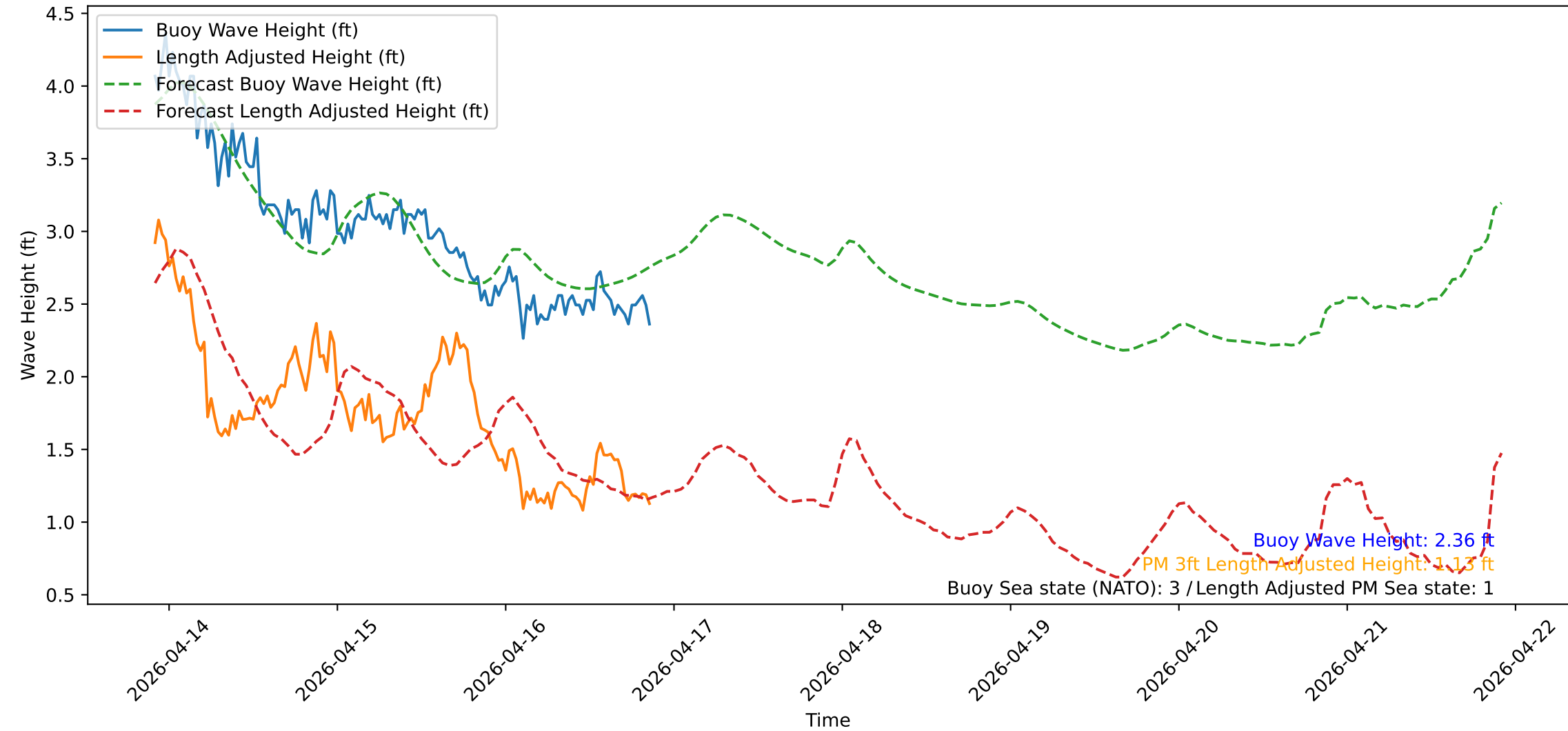
Wave Heights over Time for Red Beach at 2026-04-16 21:30:50
