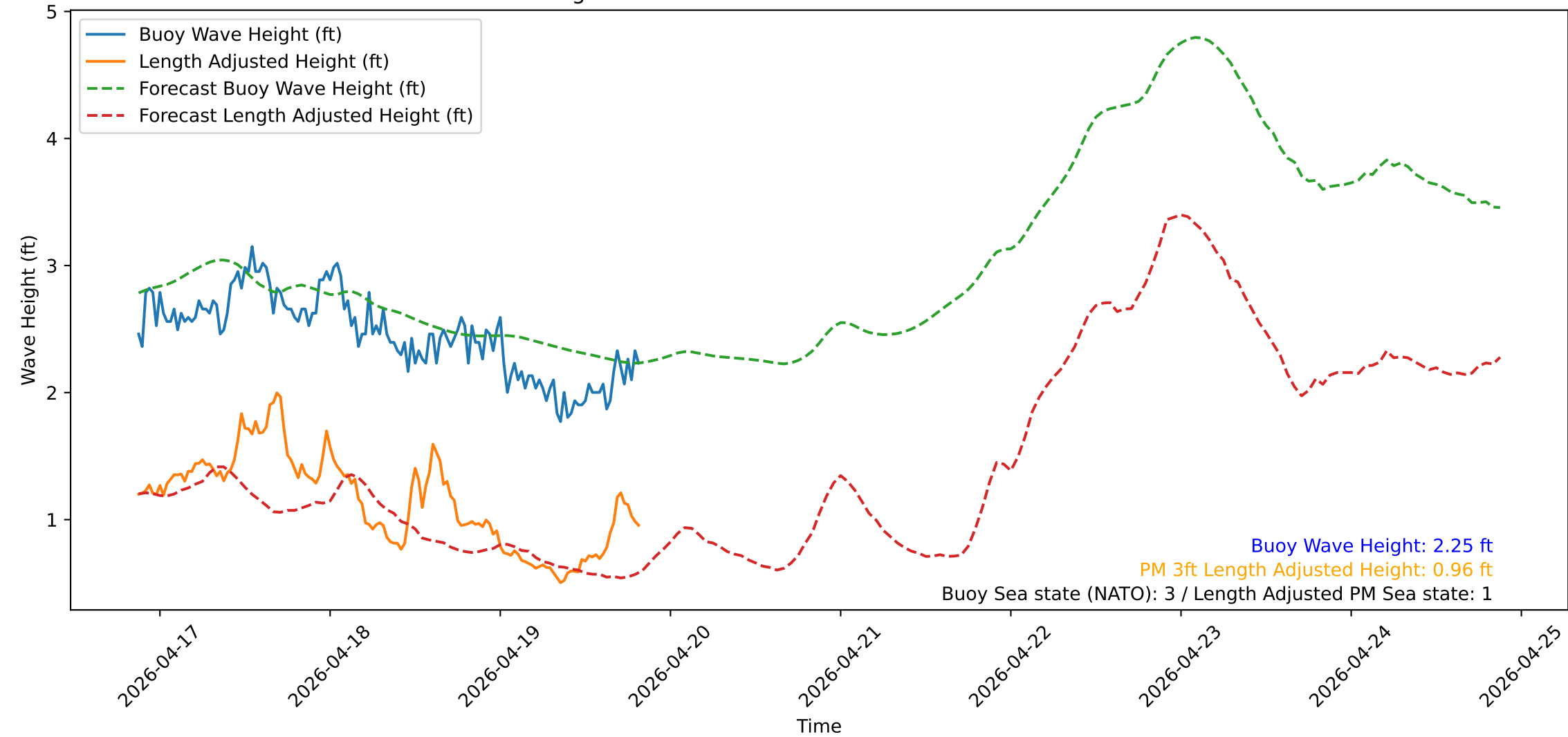
Wave Heights over Time for Red Beach at 2026-04-19 20:40:50
