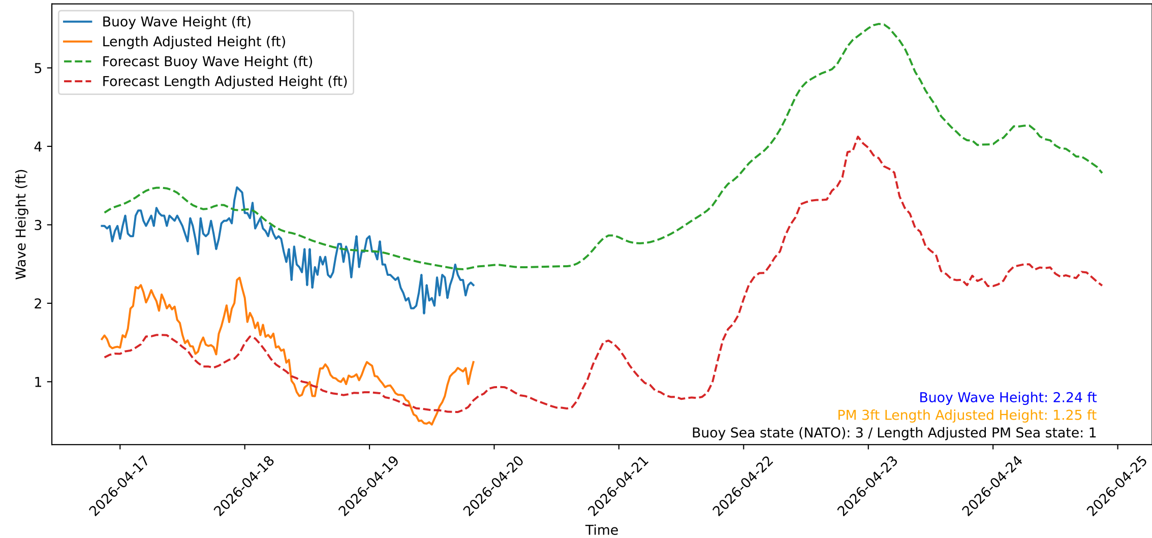
Wave Heights over Time for Green Beach at 2026-04-19 20:41:13
