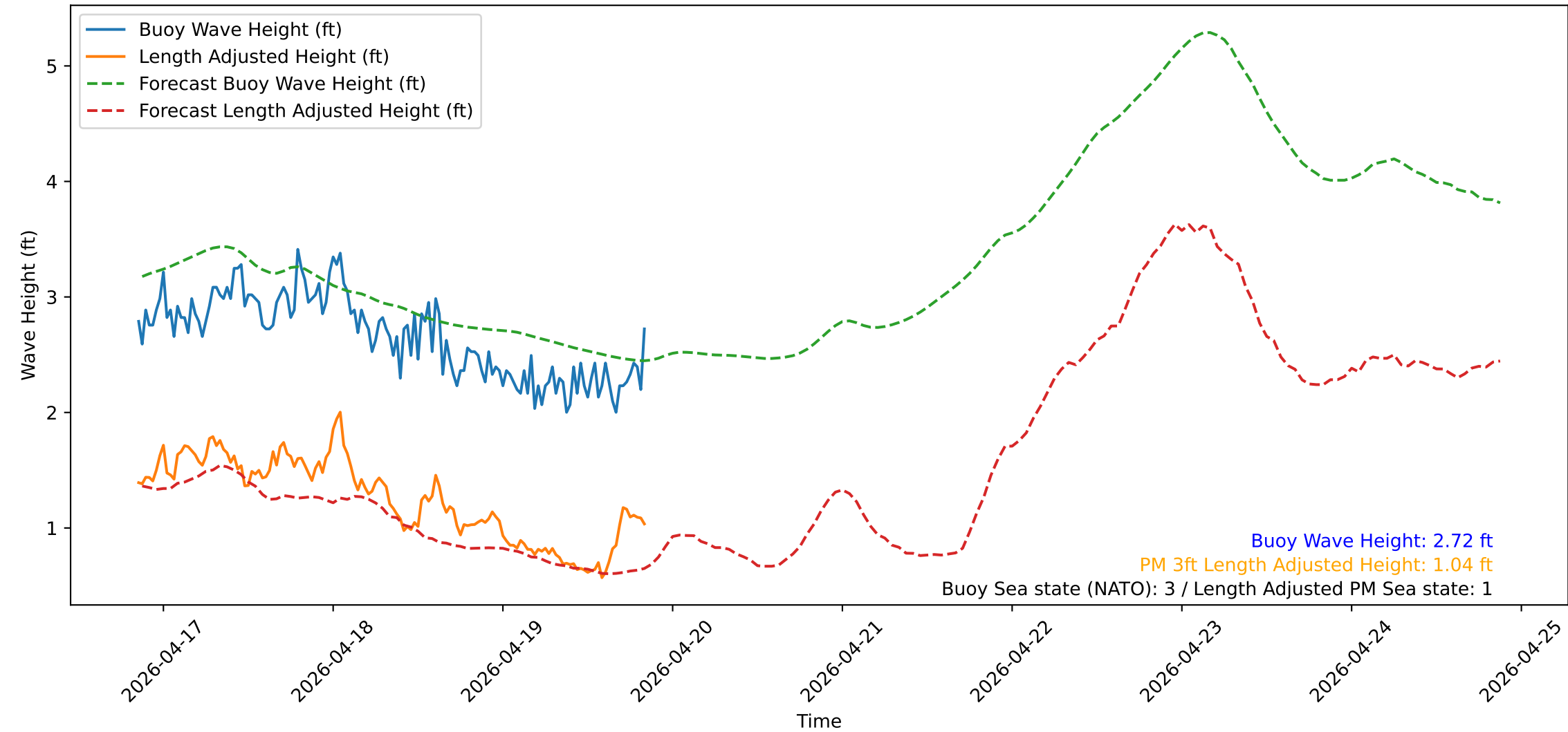
Wave Heights over Time for Oceanside Harbor at 2026-04-19 20:40:31
