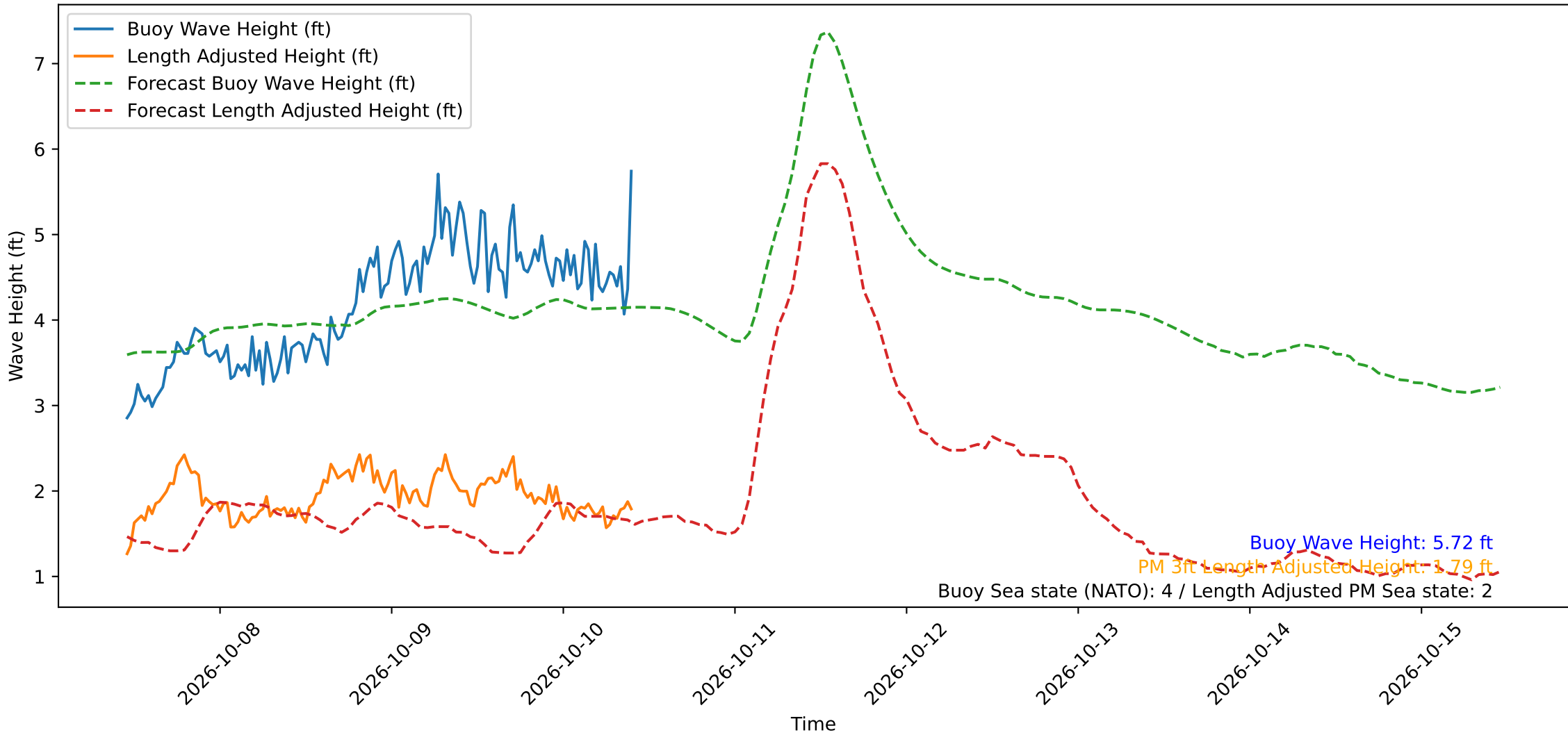
Wave Heights over Time for Red Beach at 2026-10-10 10:30:49
