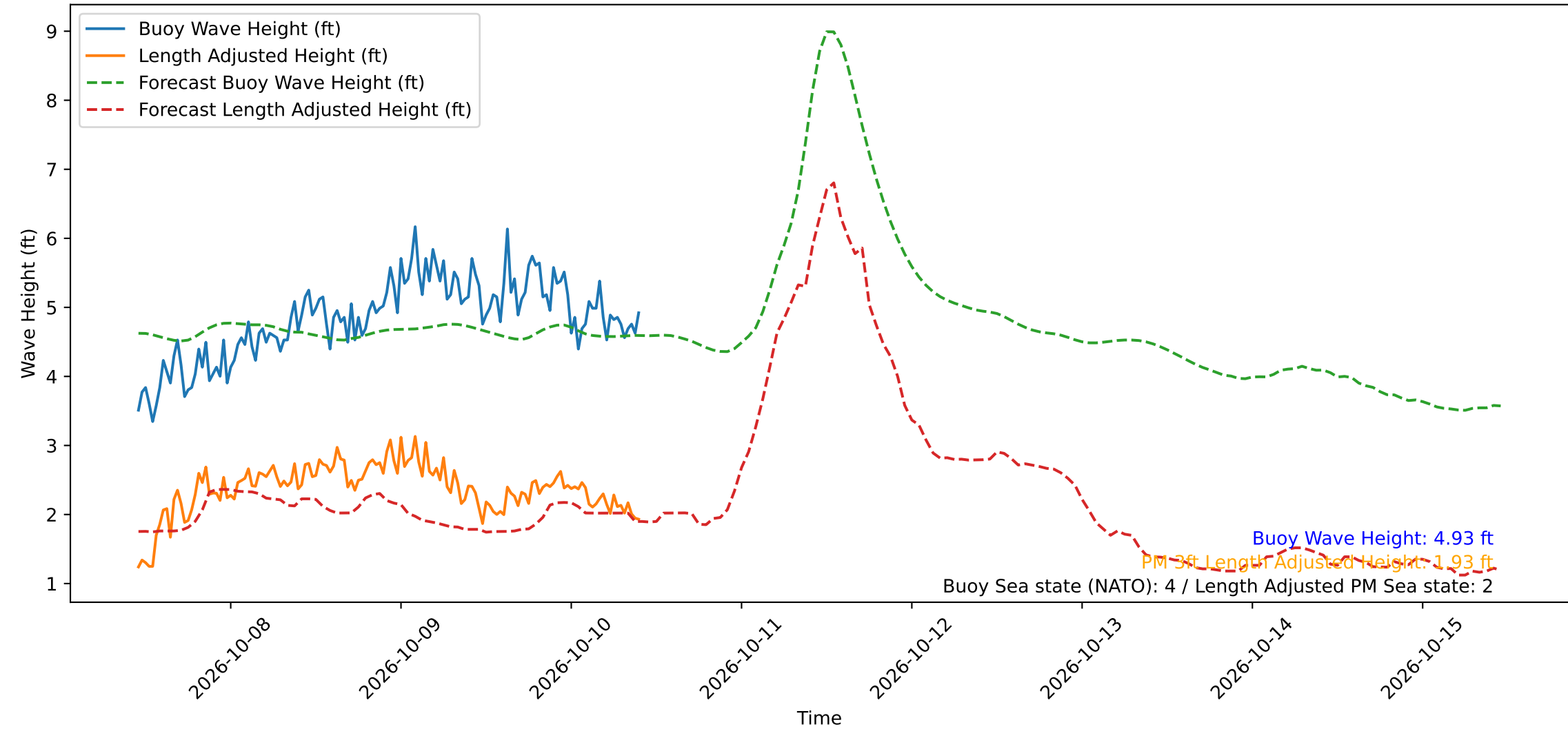
Wave Heights over Time for Green Beach at 2026-10-10 10:31:11
