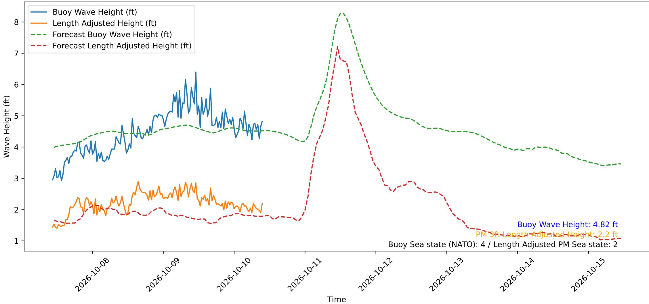
Wave Heights over Time for Oceanside Harbor at 2026-10-10 10:30:29
