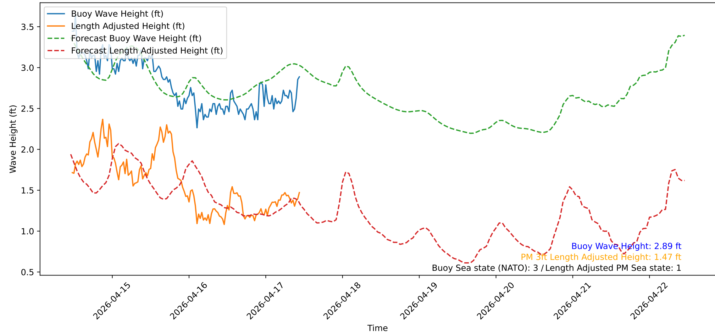
Wave Heights over Time for Red Beach at 2026-04-17 11:10:51
