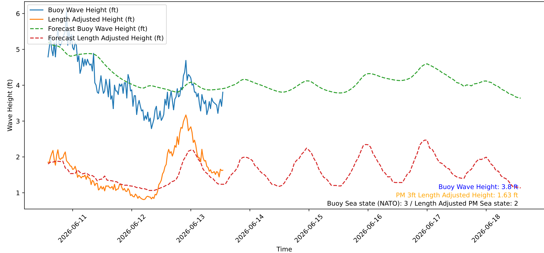
Wave Heights over Time for Oceanside Harbor at 2026-06-13 14:00:27
