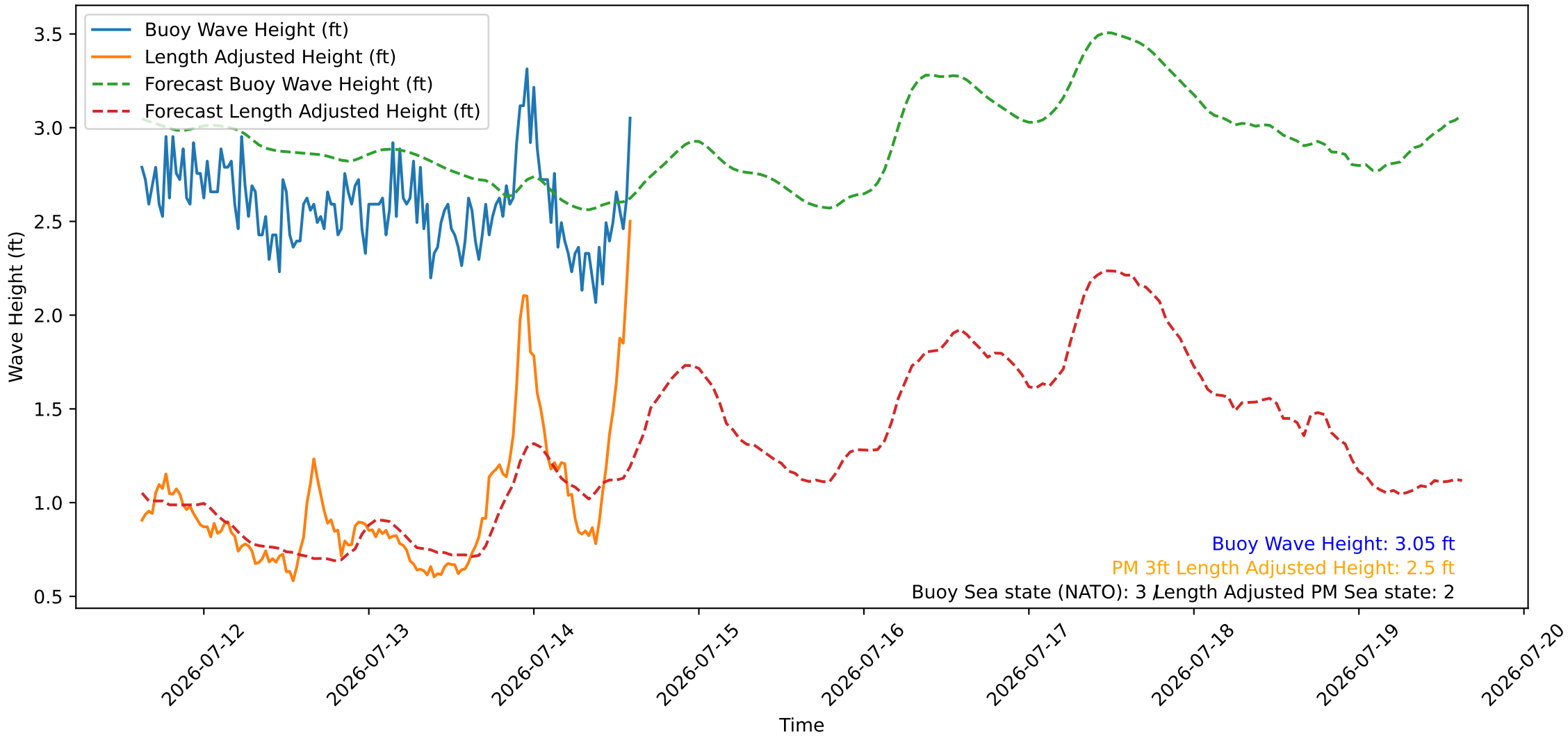
Wave Heights over Time for Green Beach at 2026-07-14 14:51:10
