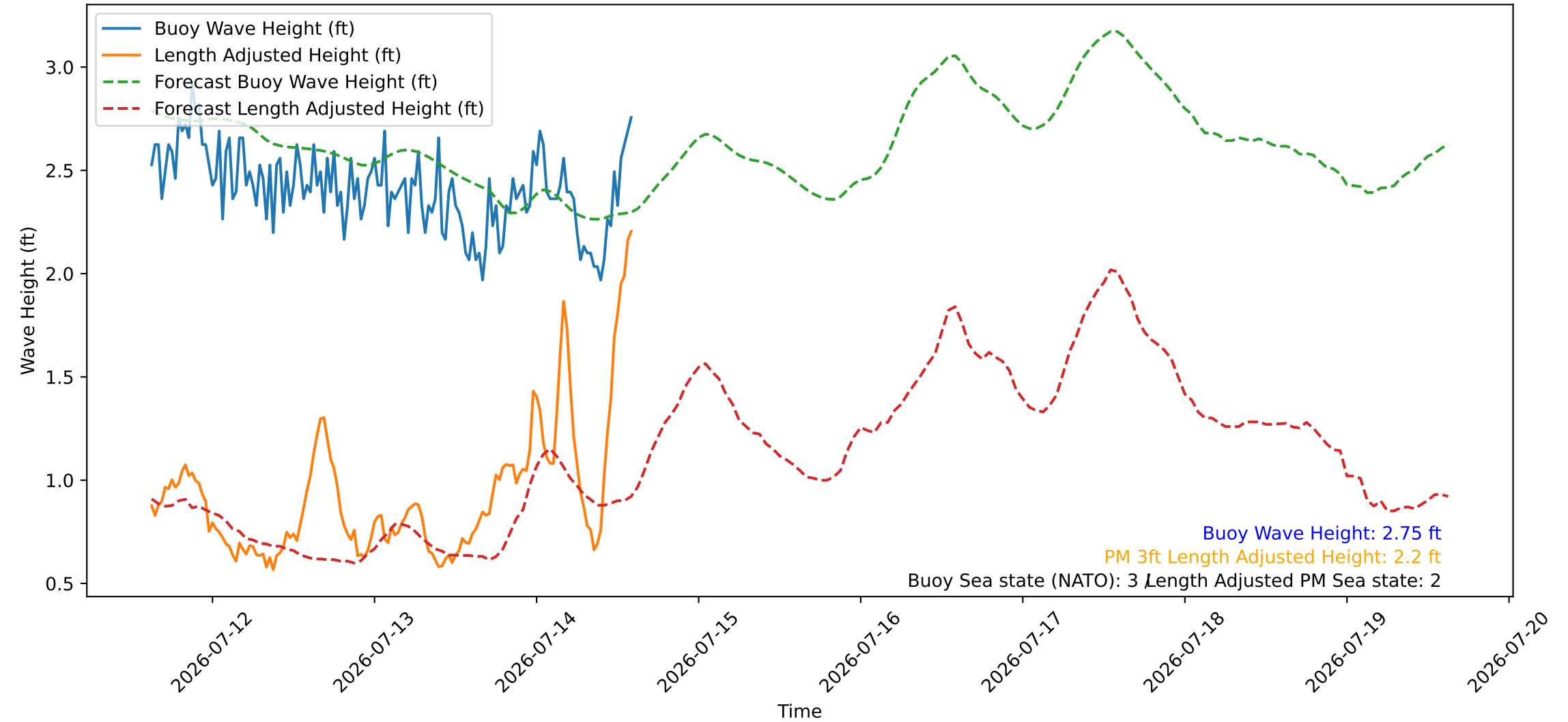
Wave Heights over Time for Red Beach at 2026-07-14 14:50:48
