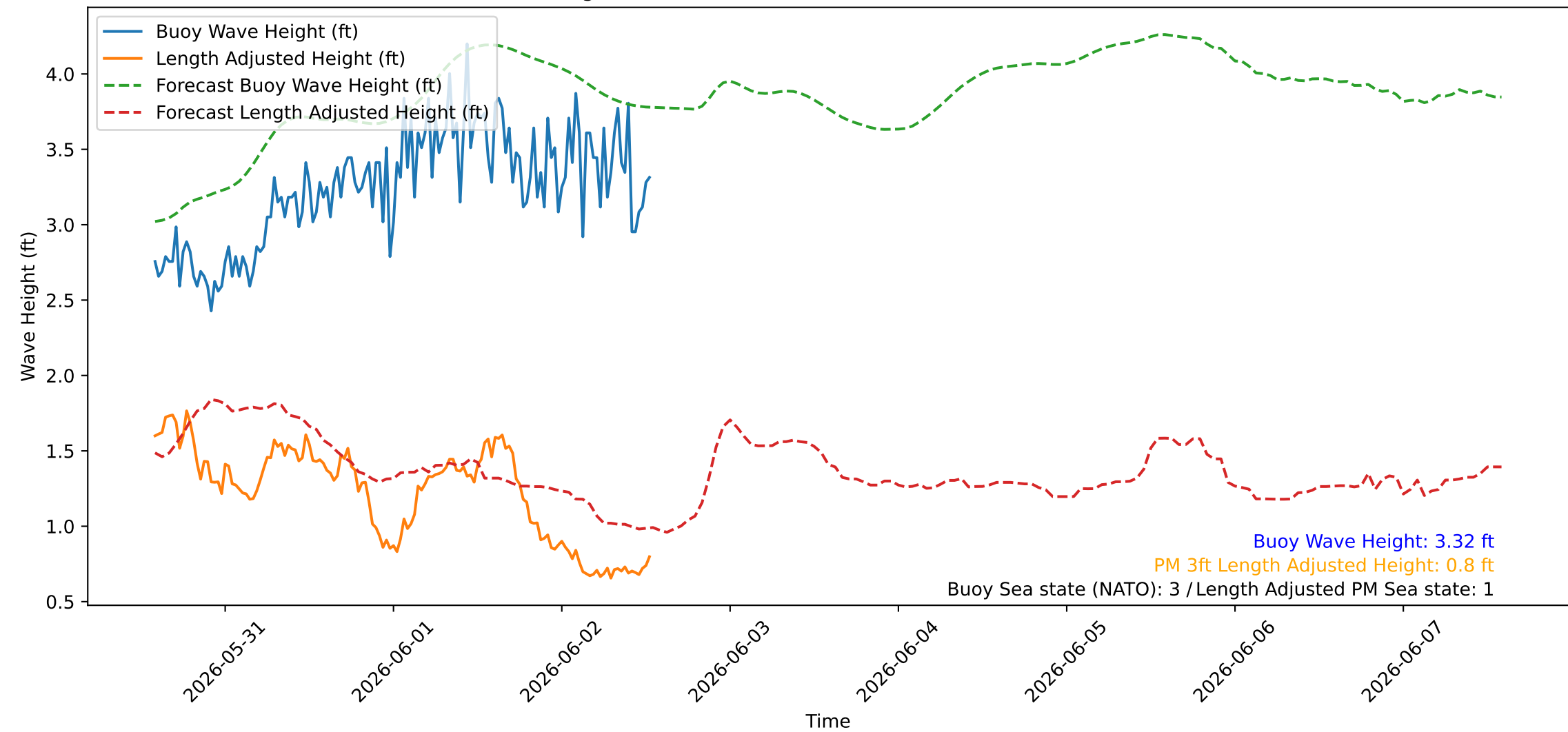
Wave Heights over Time for Red Beach at 2026-06-02 13:30:45
