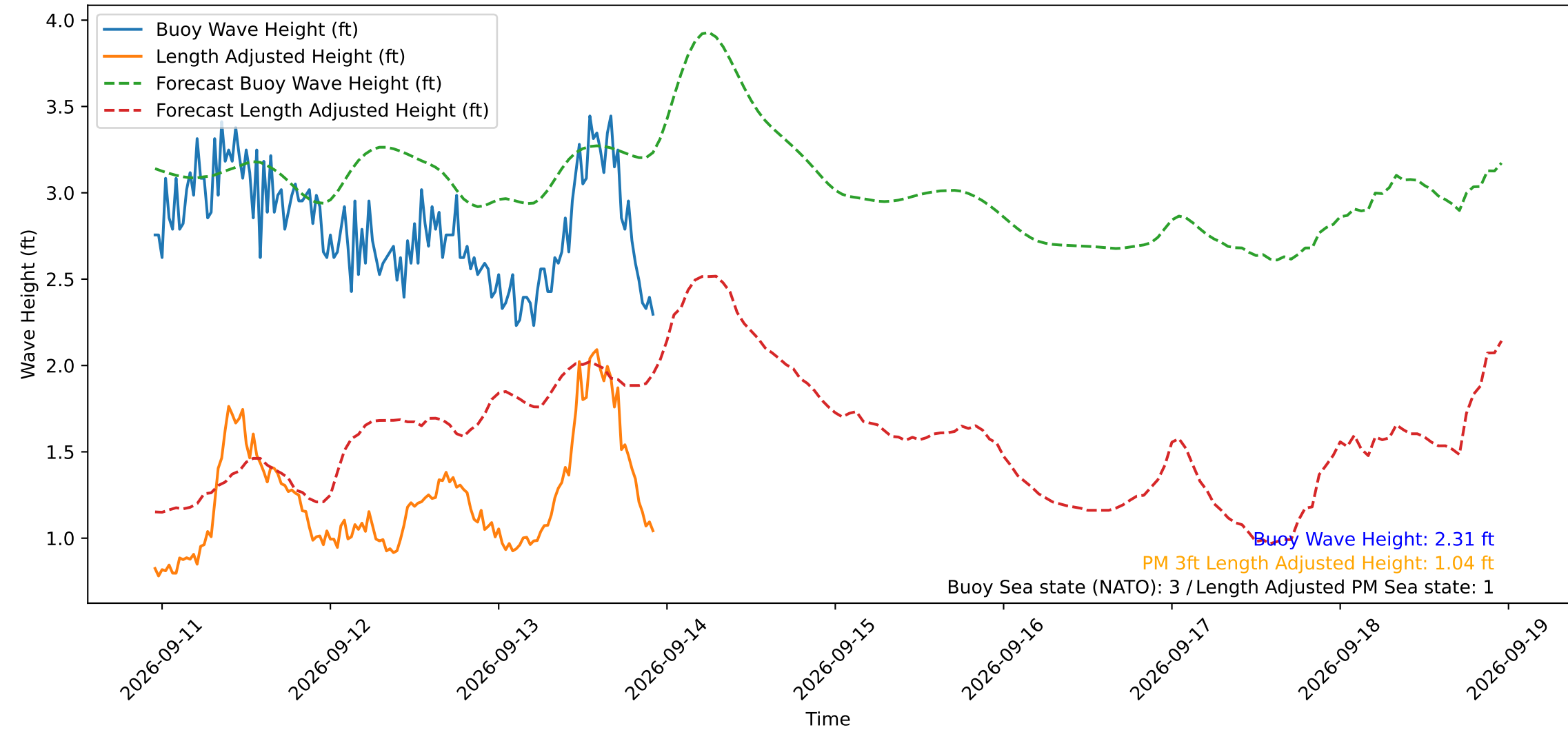
Wave Heights over Time for Red Beach at 2026-09-13 22:40:49
