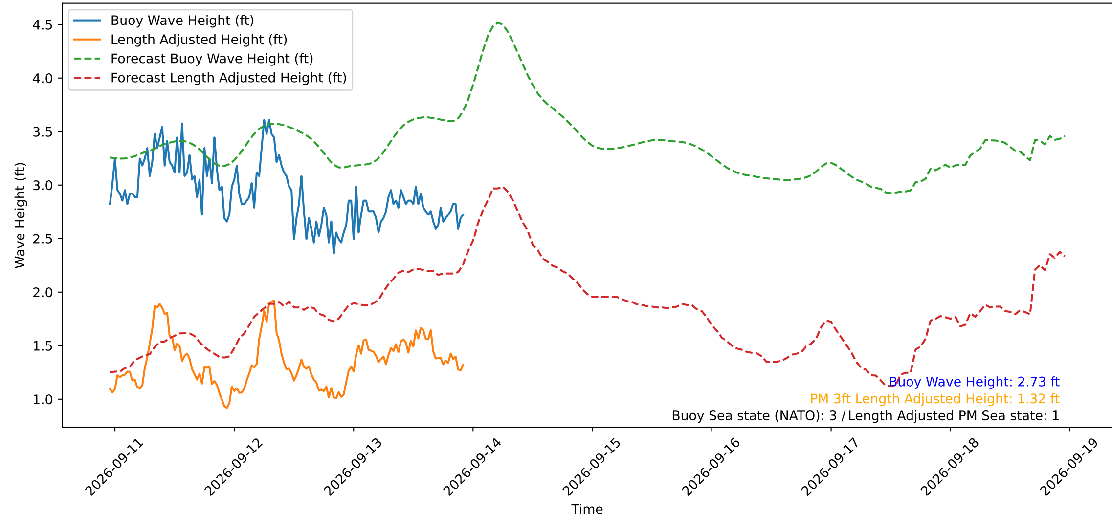
Wave Heights over Time for Green Beach at 2026-09-13 22:41:11
