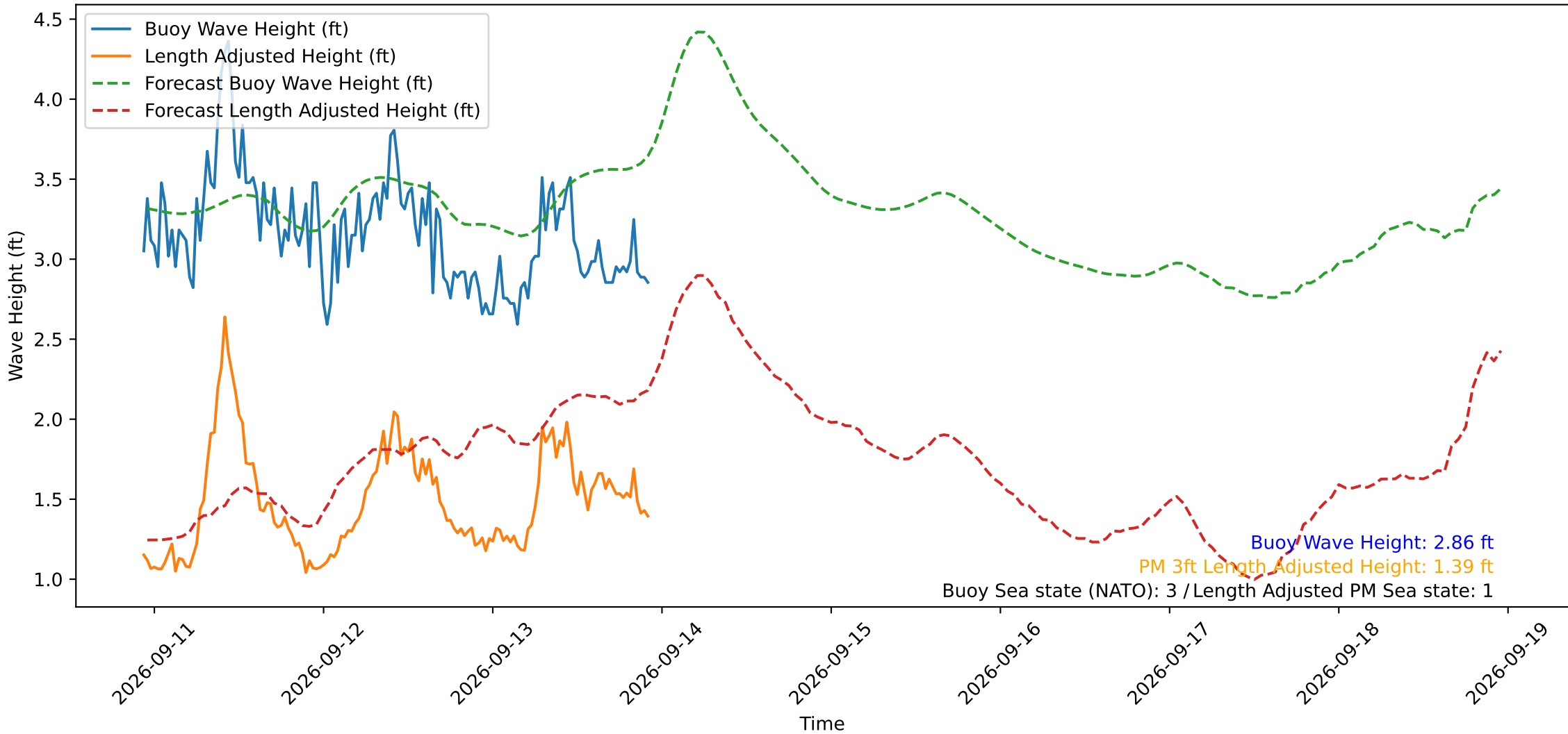
Wave Heights over Time for Oceanside Harbor at 2026-09-13 22:40:29
