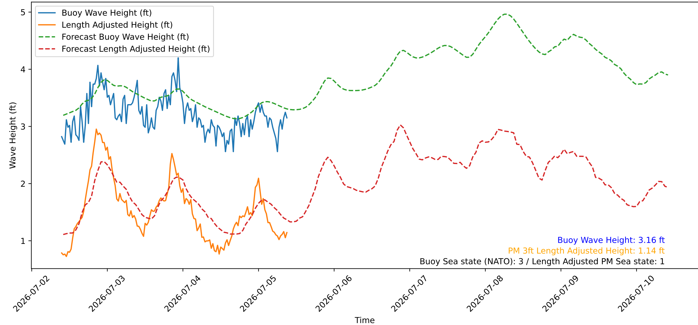
Wave Heights over Time for Green Beach at 2026-07-05 09:41:10
