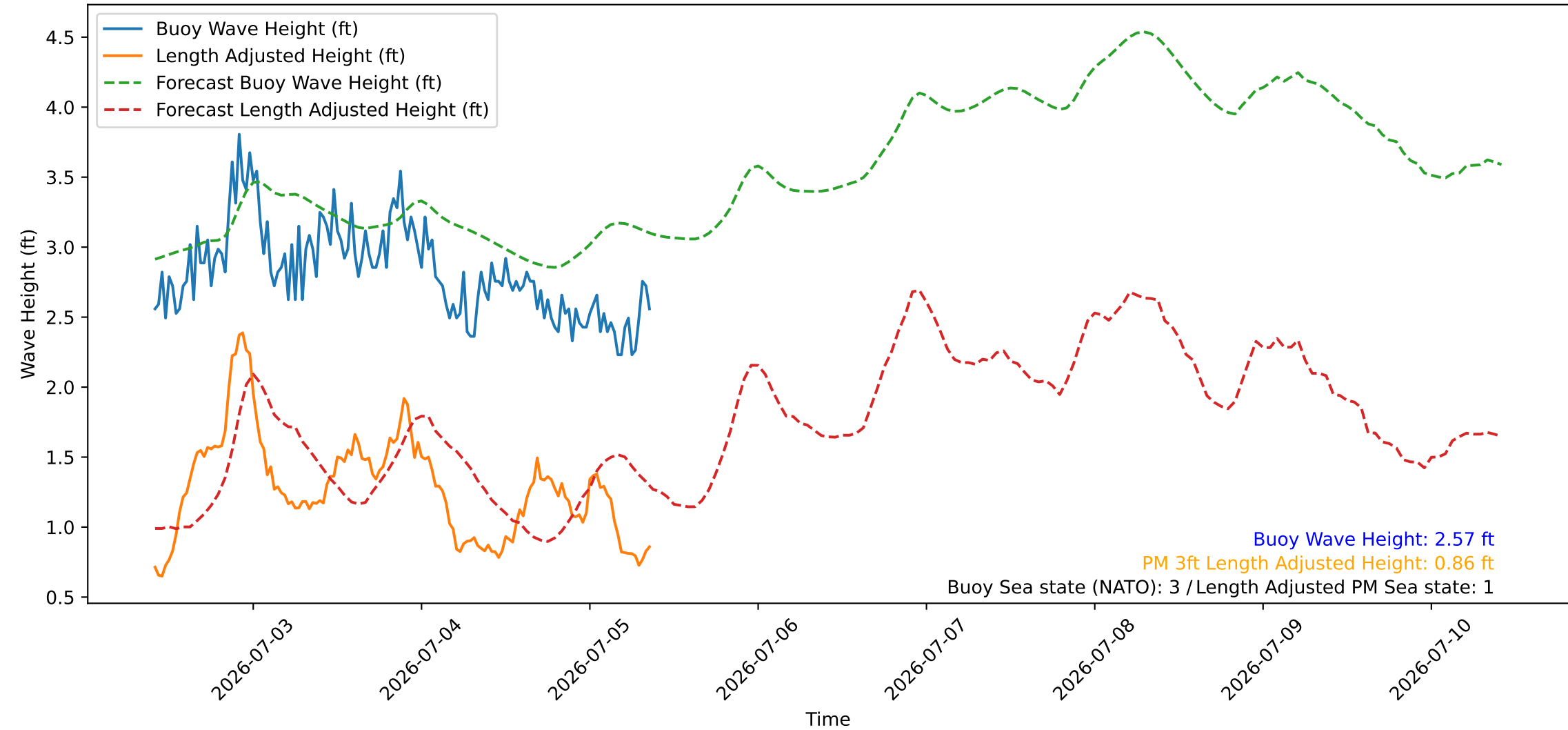
Wave Heights over Time for Red Beach at 2026-07-05 09:40:47
