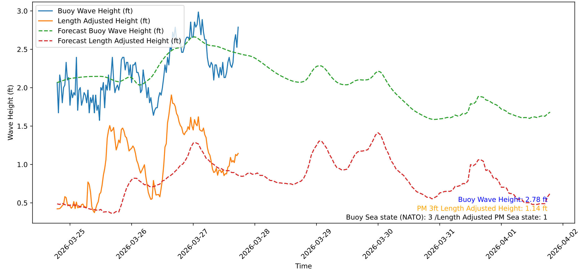
Wave Heights over Time for Red Beach at 2026-03-27 18:30:47
