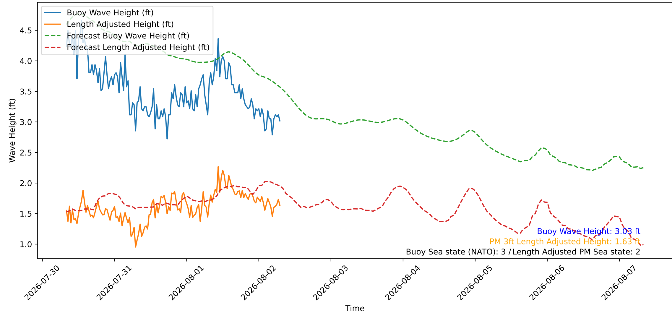
Wave Heights over Time for Oceanside Harbor at 2026-08-02 07:50:26
