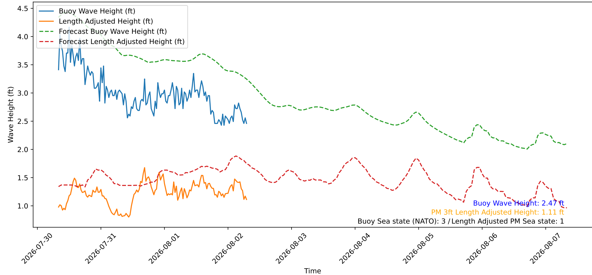
Wave Heights over Time for Red Beach at 2026-08-02 07:50:47
