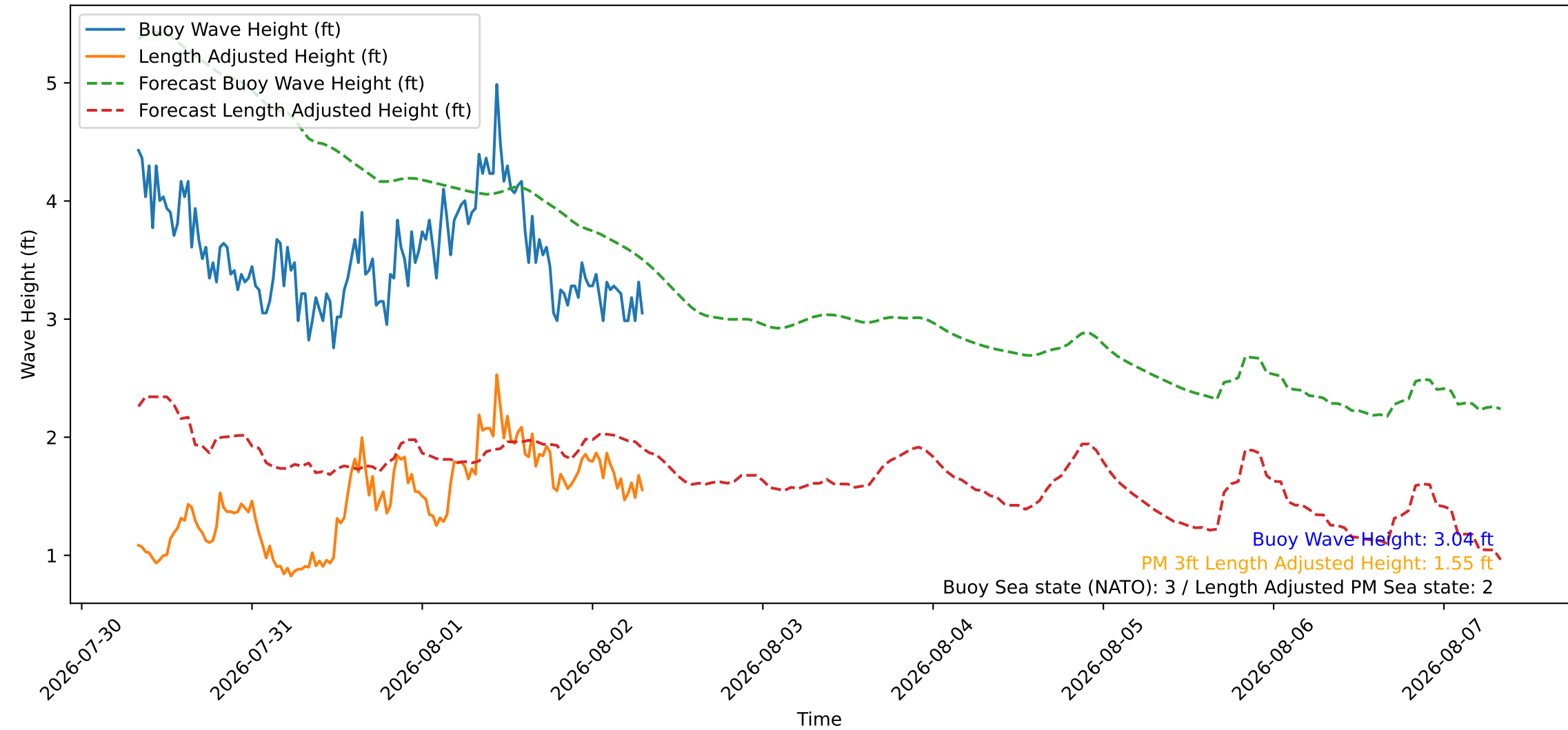
Wave Heights over Time for Green Beach at 2026-08-02 07:51:10
