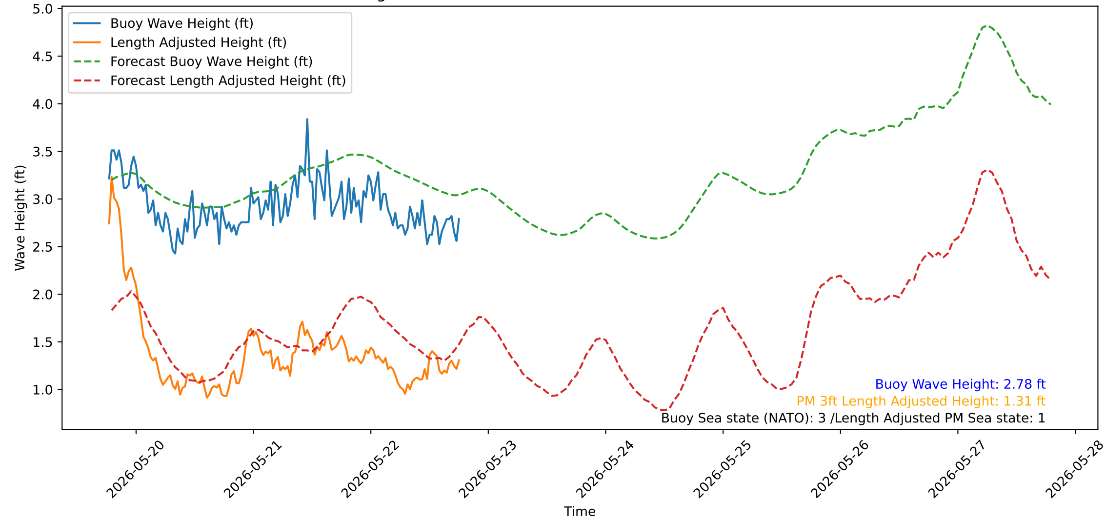
Wave Heights over Time for Oceanside Harbor at 2026-05-22 18:30:31
