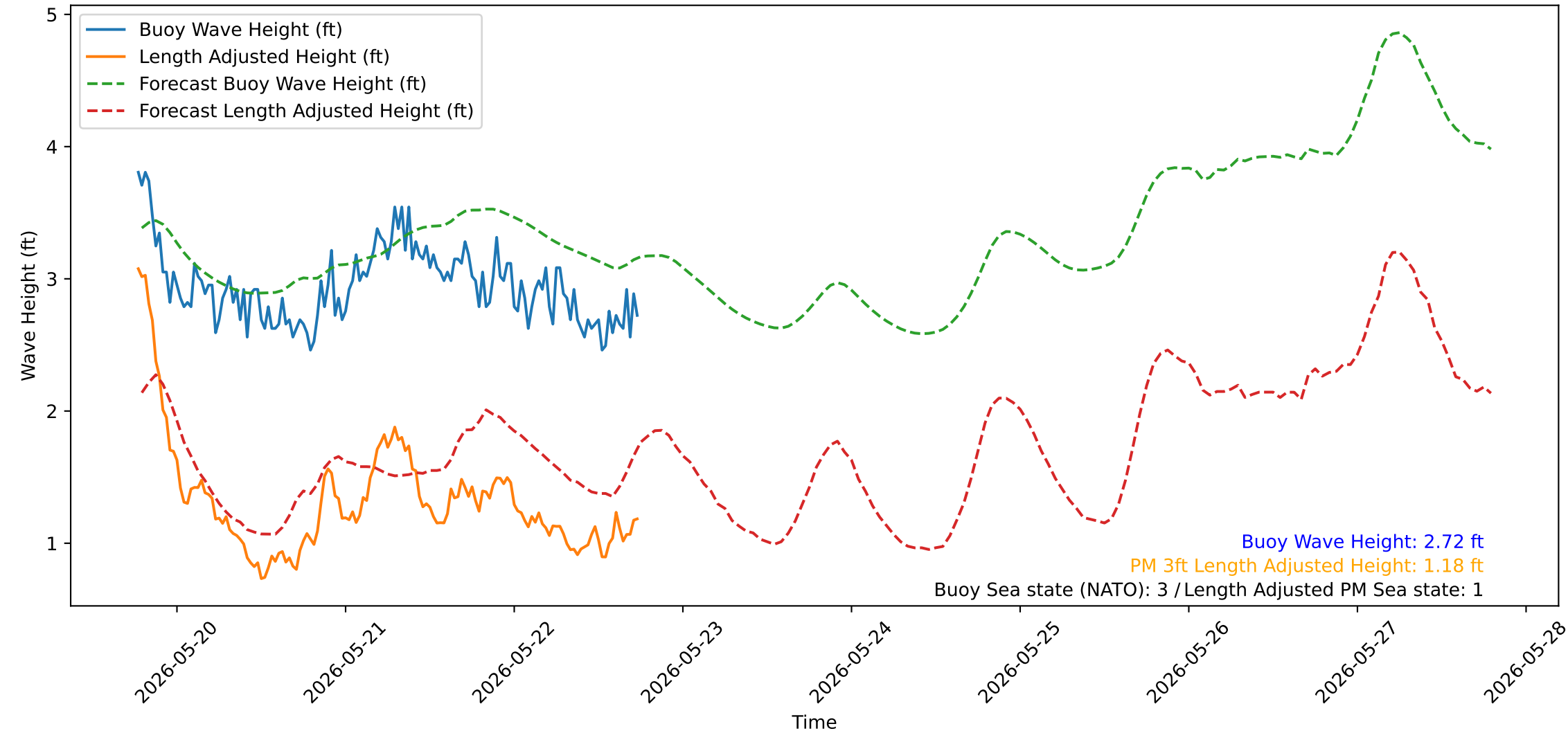
Wave Heights over Time for Green Beach at 2026-05-22 18:31:13
