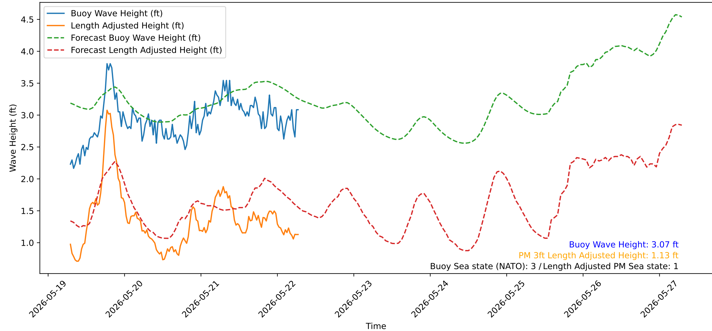
Wave Heights over Time for Green Beach at 2026-05-22 07:11:13
