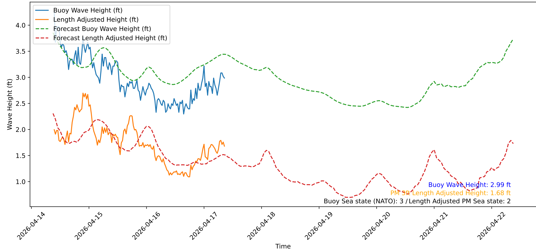
Wave Heights over Time for Oceanside Harbor at 2026-04-17 09:20:33
