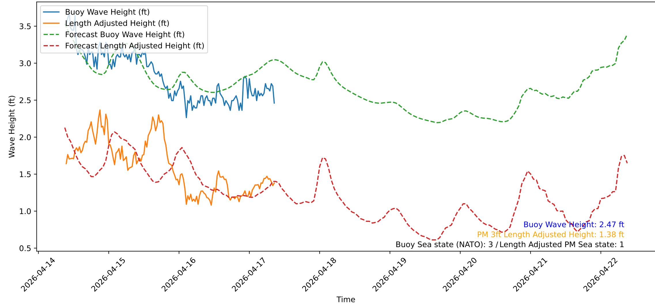
Wave Heights over Time for Red Beach at 2026-04-17 09:20:55
