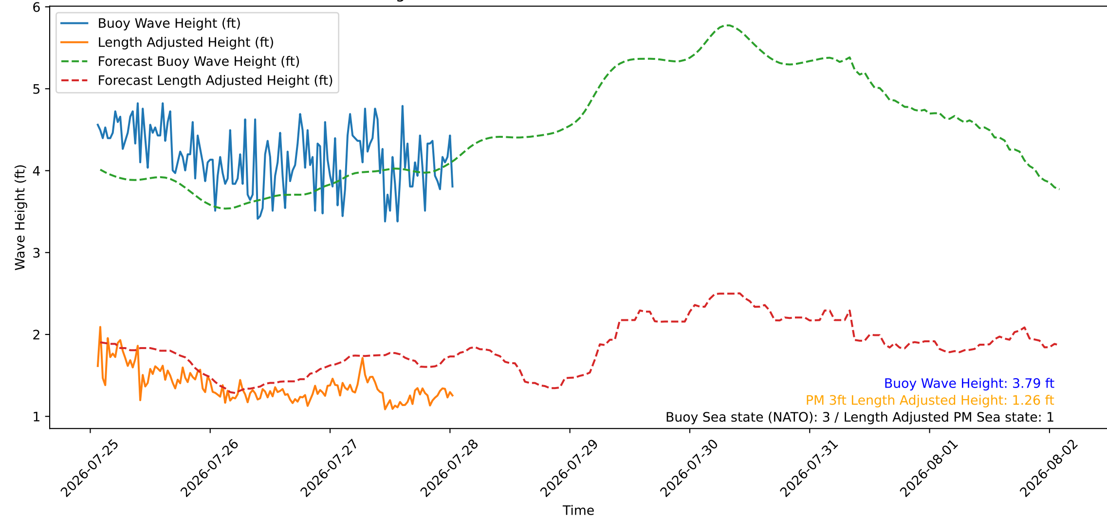
Wave Heights over Time for Green Beach at 2026-07-28 01:31:08
