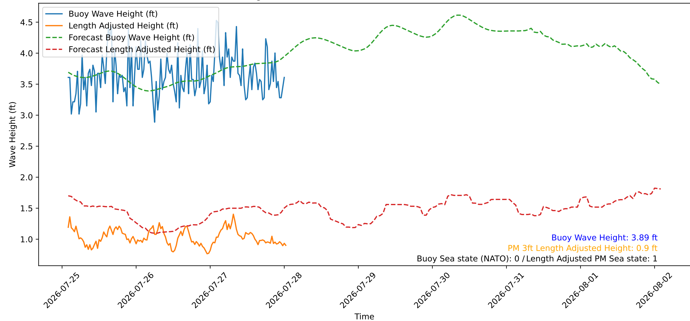
Wave Heights over Time for Red Beach at 2026-07-28 01:30:46
