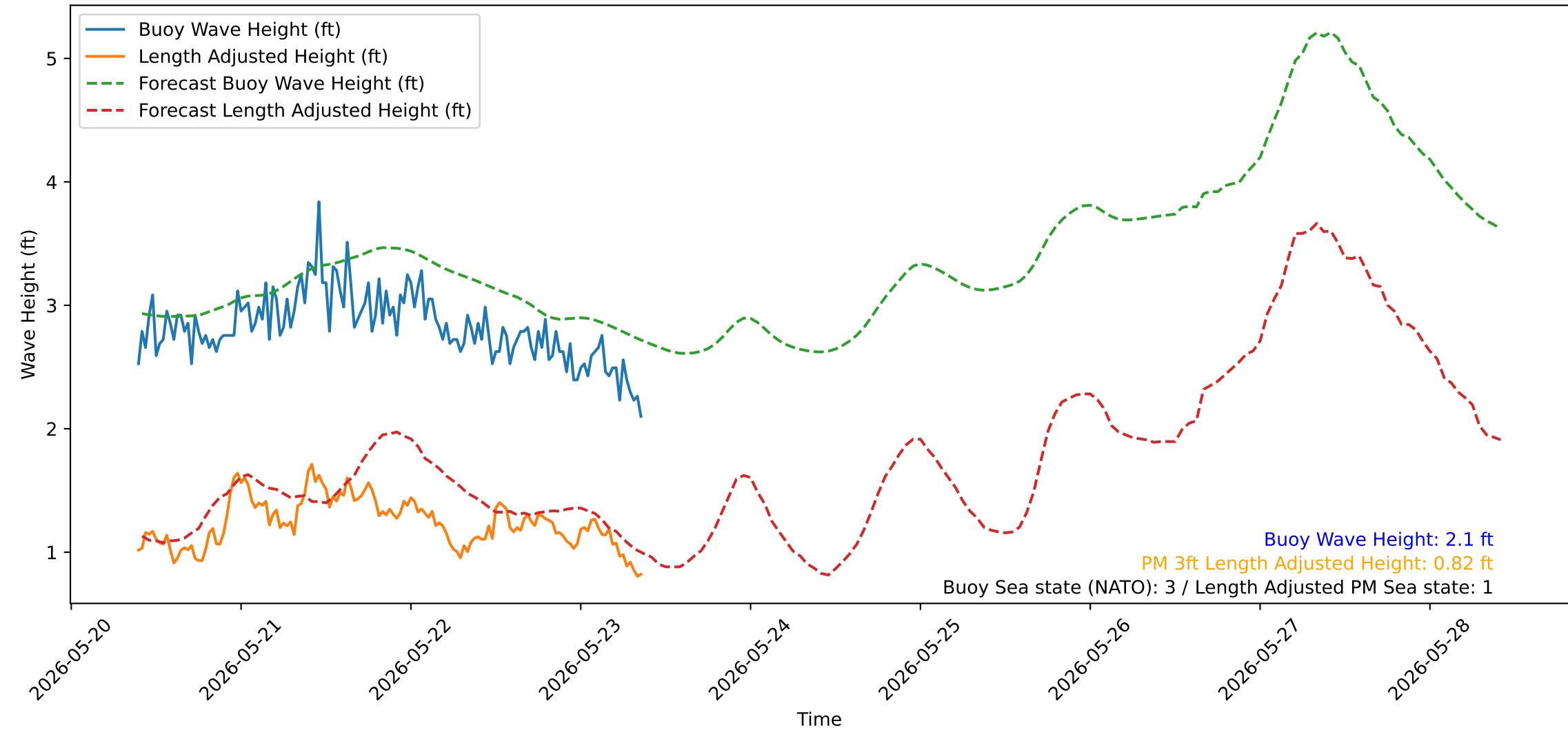
Wave Heights over Time for Oceanside Harbor at 2026-05-23 09:30:32
