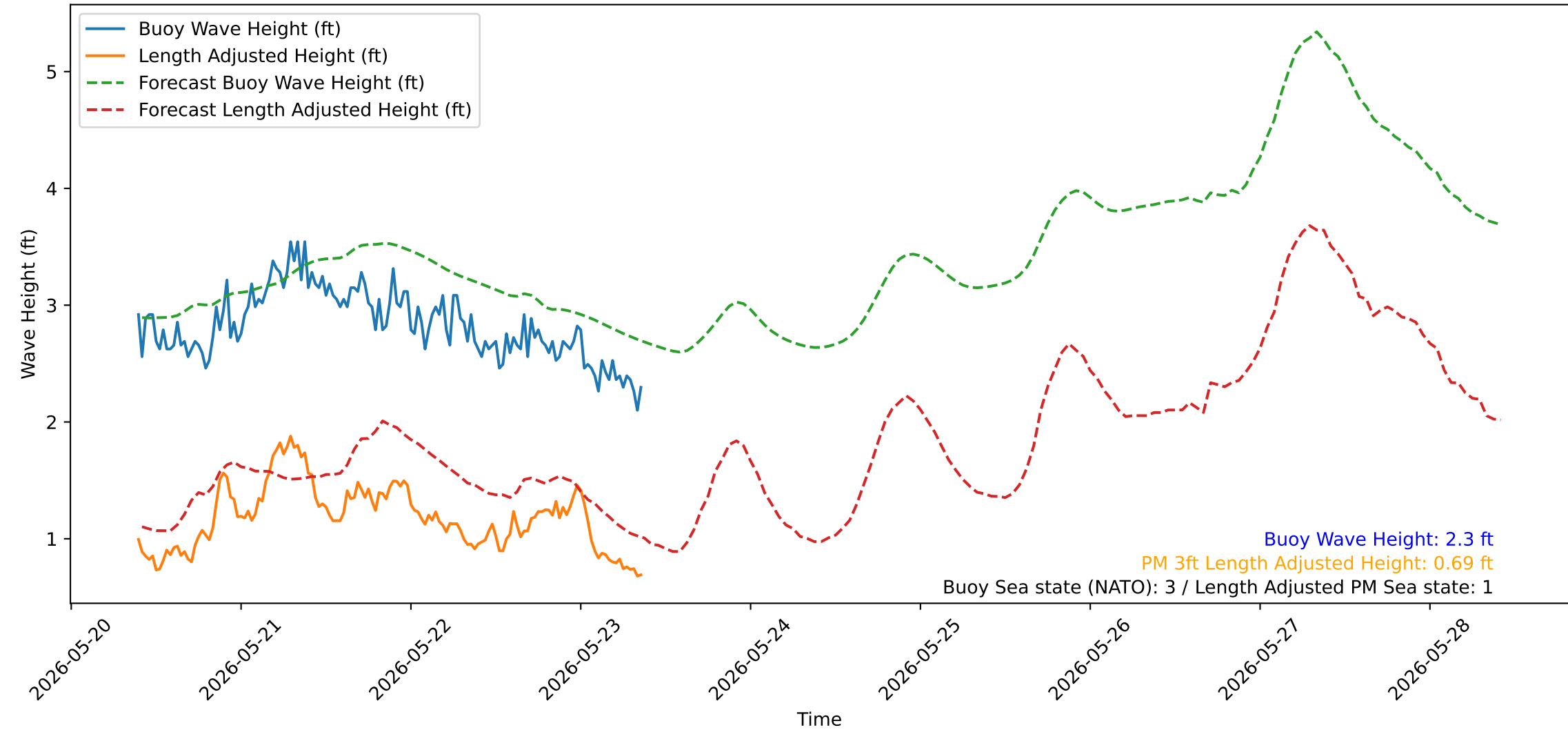
Wave Heights over Time for Green Beach at 2026-05-23 09:31:14
