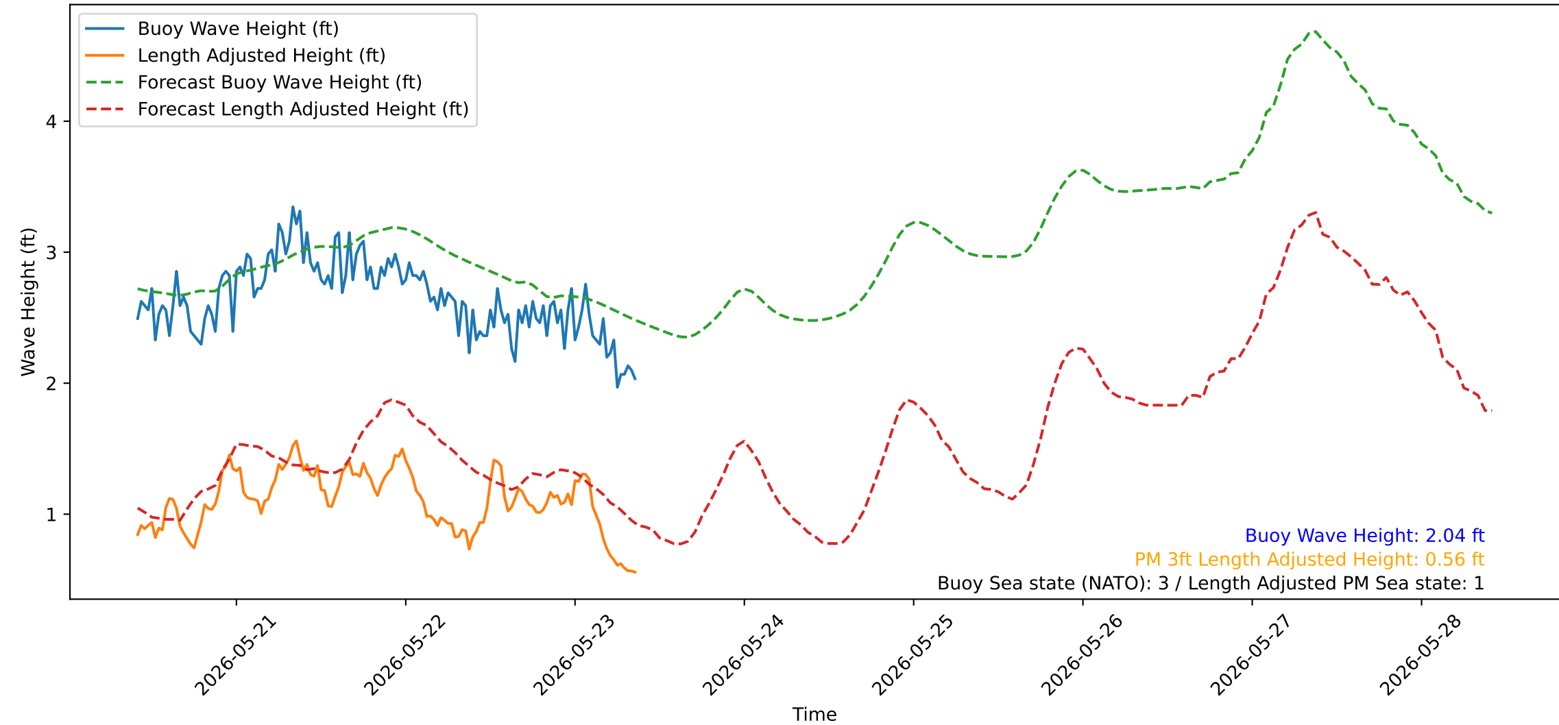
Wave Heights over Time for Red Beach at 2026-05-23 09:30:51
