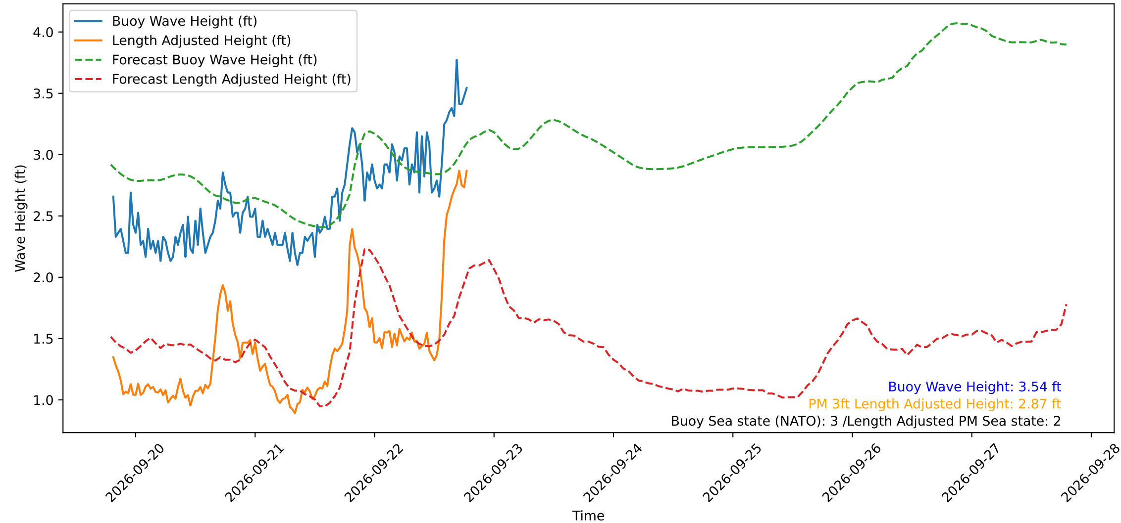
Wave Heights over Time for Oceanside Harbor at 2026-09-22 19:20:30
