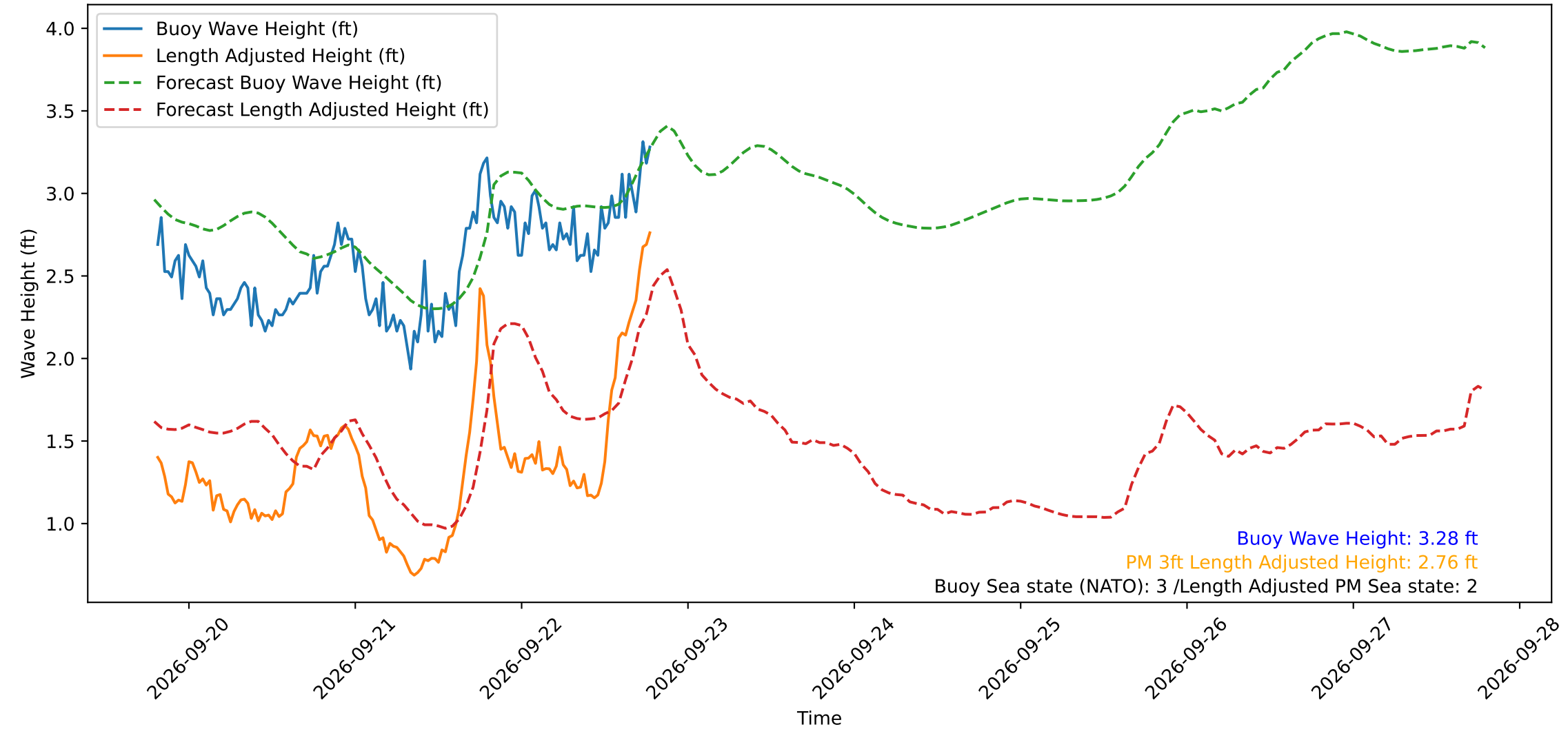
Wave Heights over Time for Green Beach at 2026-09-22 19:21:14
