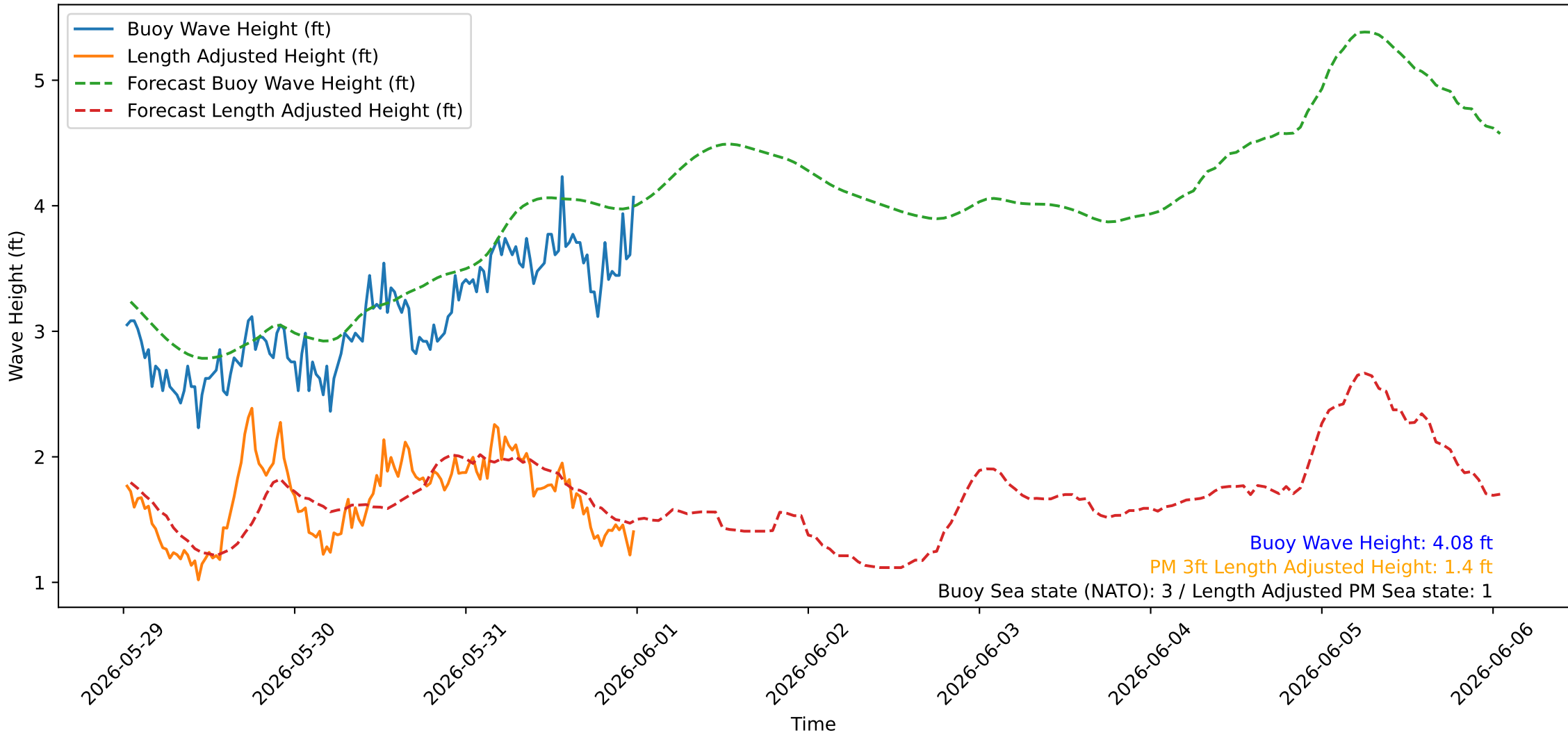
Wave Heights over Time for Oceanside Harbor at 2026-06-01 00:30:26
