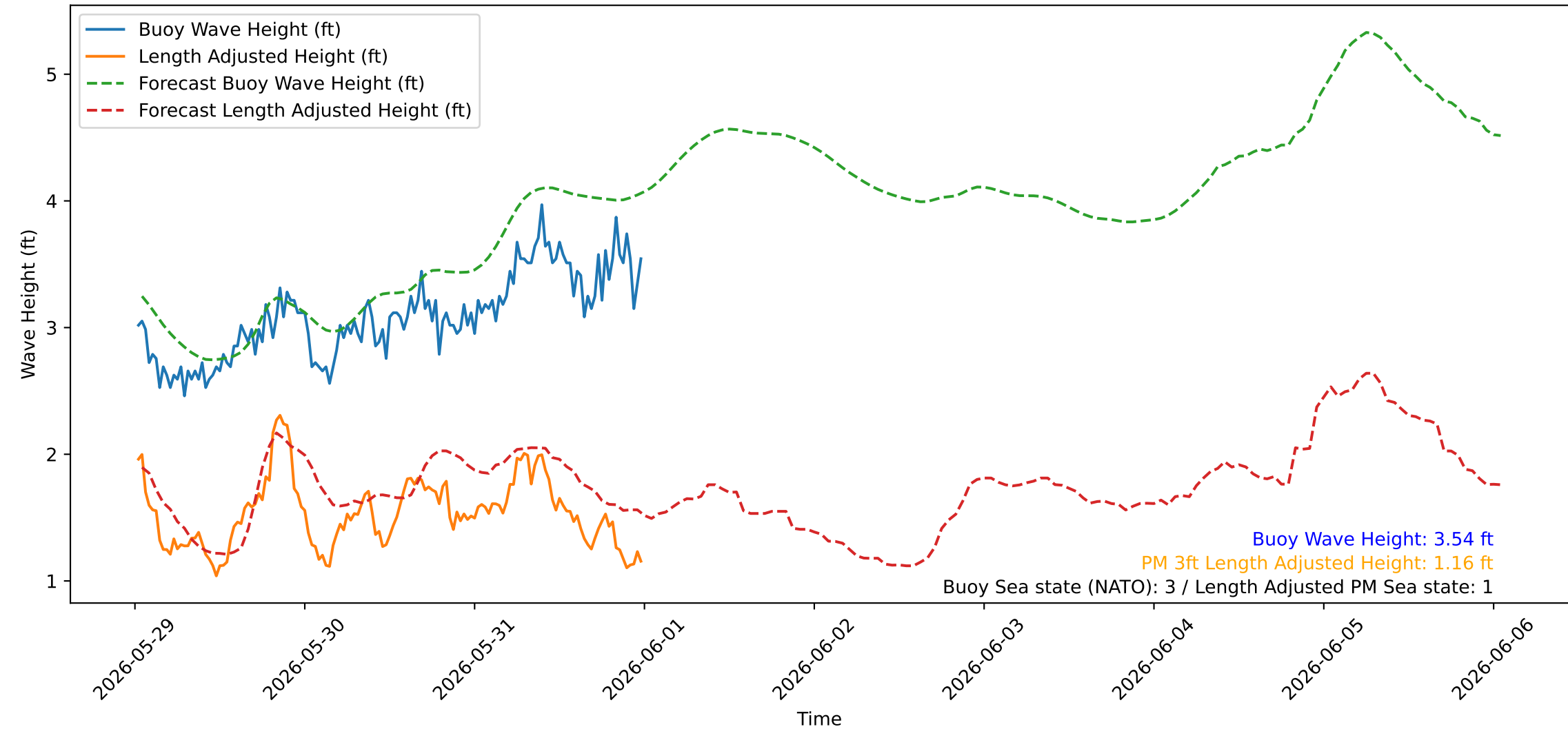
Wave Heights over Time for Green Beach at 2026-06-01 00:31:07
