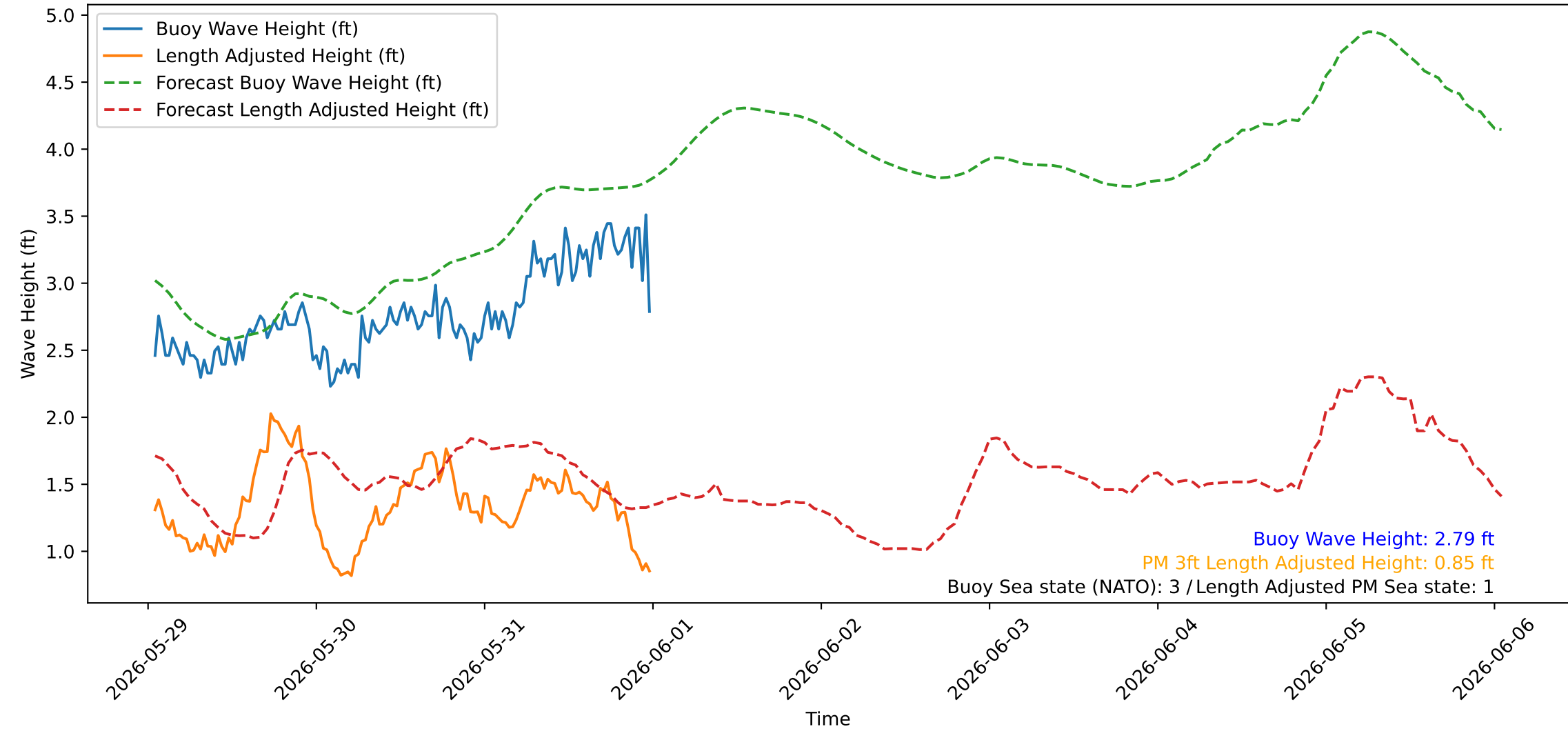
Wave Heights over Time for Red Beach at 2026-06-01 00:30:45
