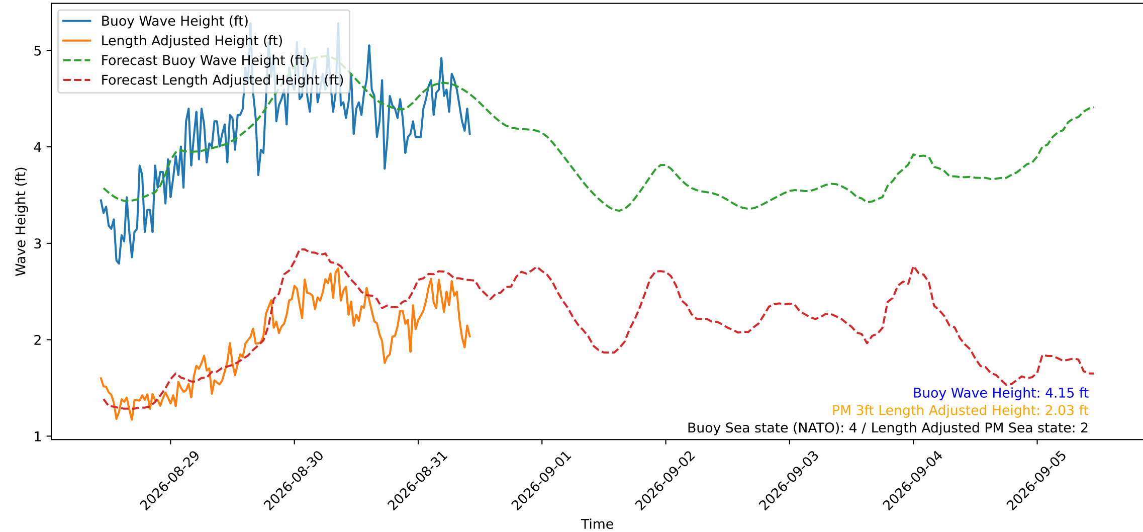
Wave Heights over Time for Oceanside Harbor at 2026-08-31 10:40:29
