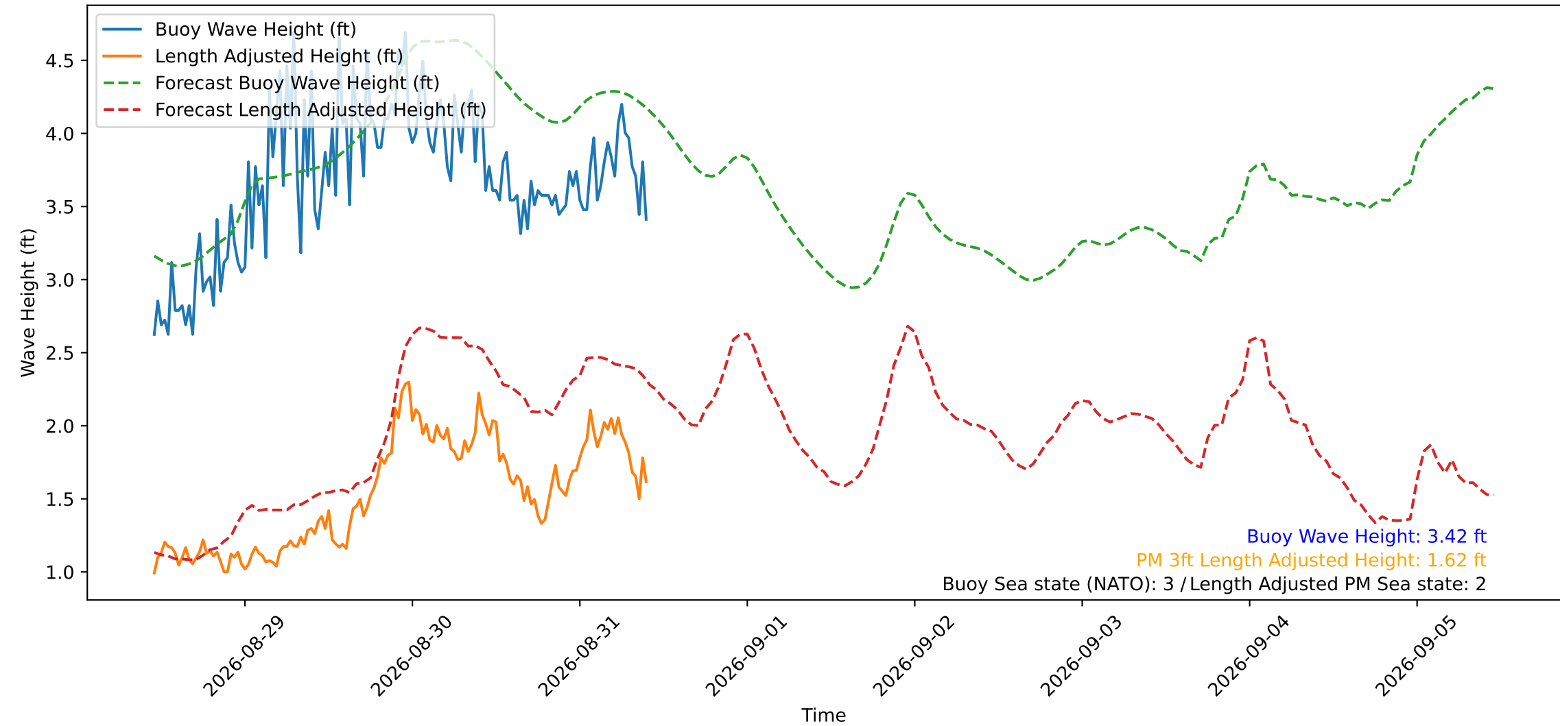
Wave Heights over Time for Red Beach at 2026-08-31 10:40:49
