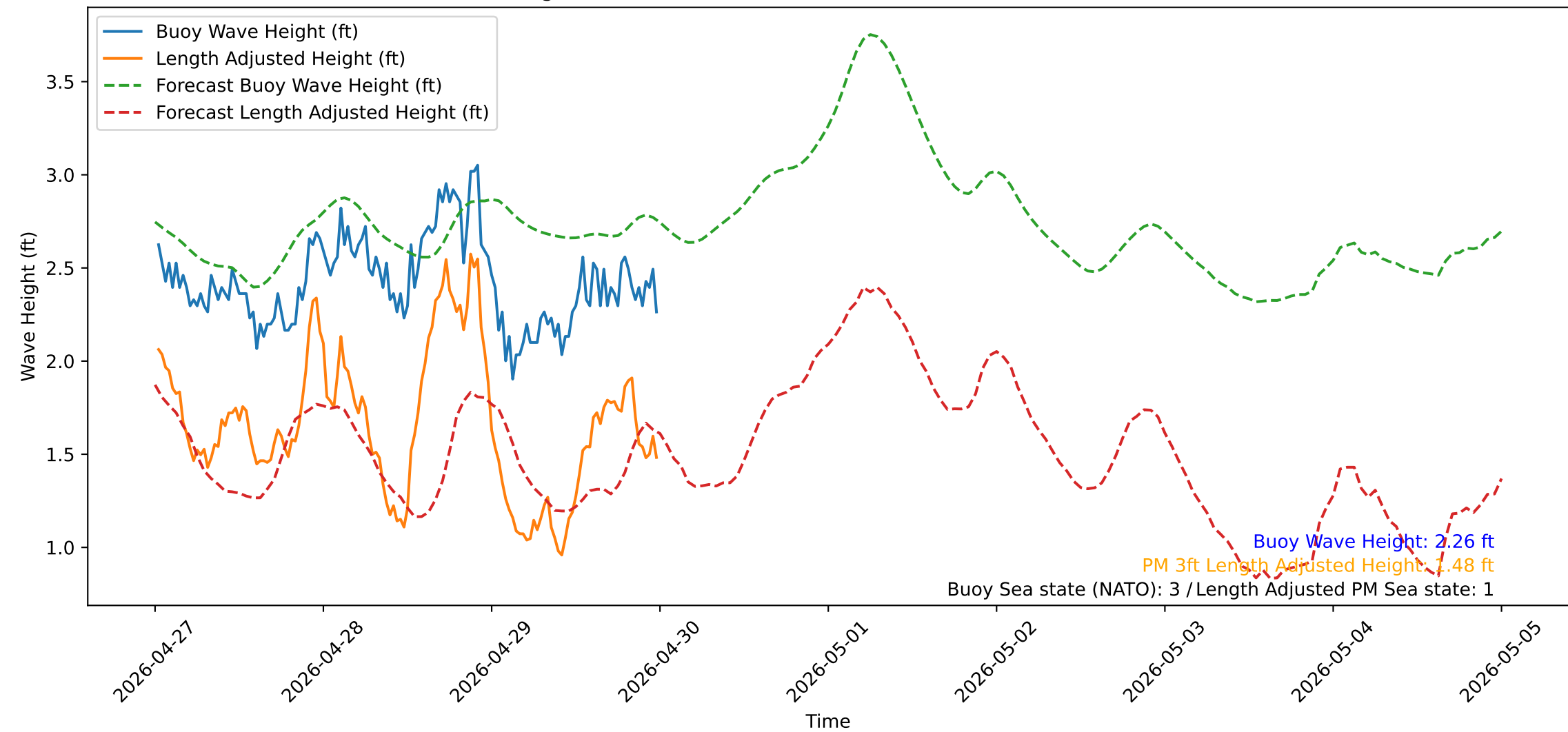
Wave Heights over Time for Oceanside Harbor at 2026-04-30 00:20:31
