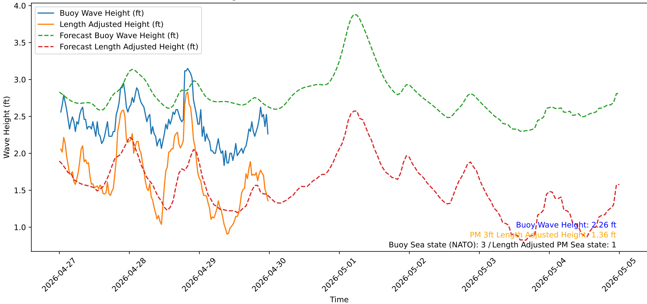
Wave Heights over Time for Green Beach at 2026-04-30 00:21:13
