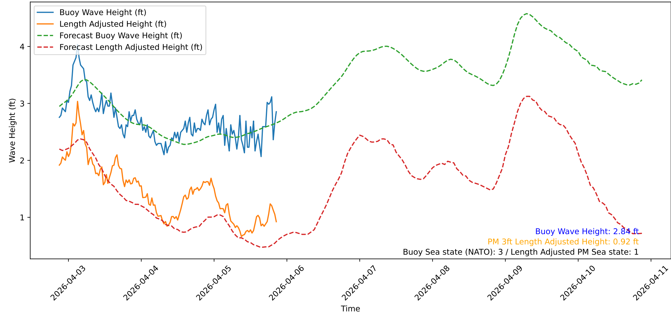
Wave Heights over Time for Oceanside Harbor at 2026-04-05 21:10:35
