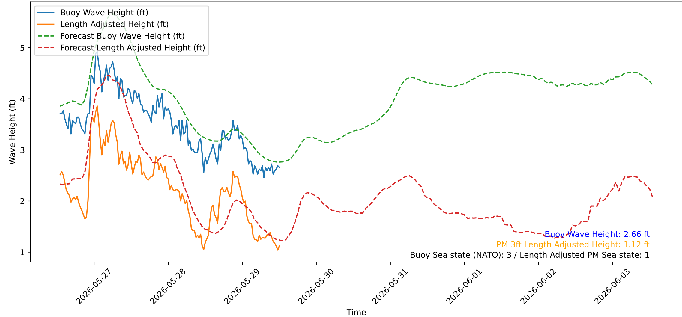
Wave Heights over Time for Green Beach at 2026-05-29 12:51:05
