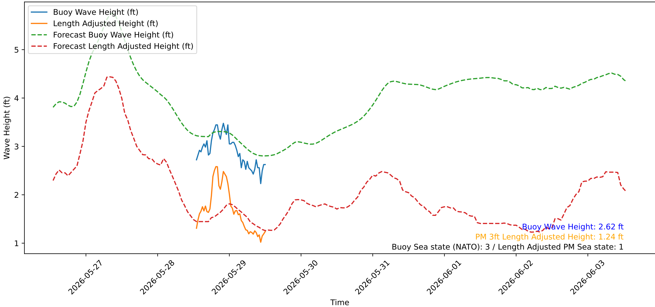
Wave Heights over Time for Oceanside Harbor at 2026-05-29 12:50:22
