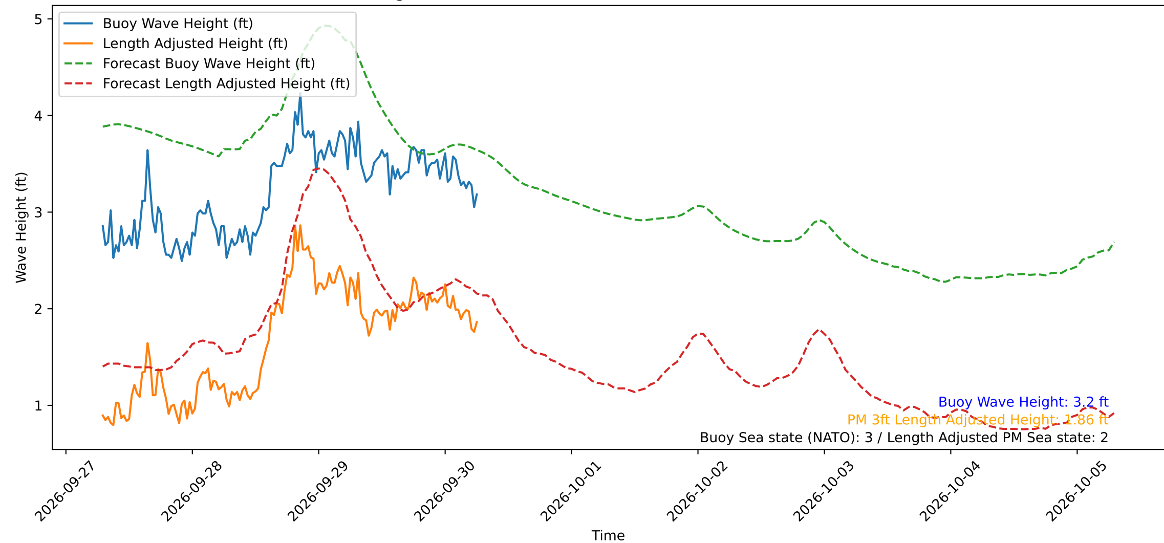
Wave Heights over Time for Oceanside Harbor at 2026-09-30 06:50:29
