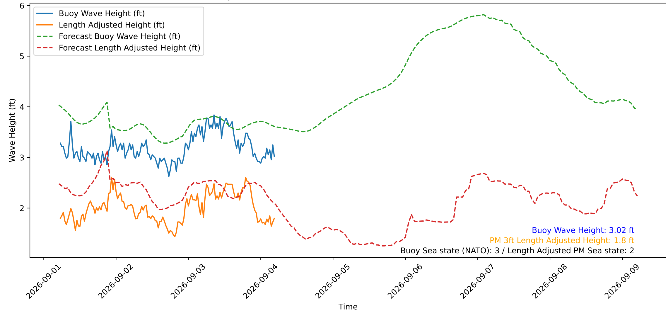
Wave Heights over Time for Oceanside Harbor at 2026-09-04 05:20:30
