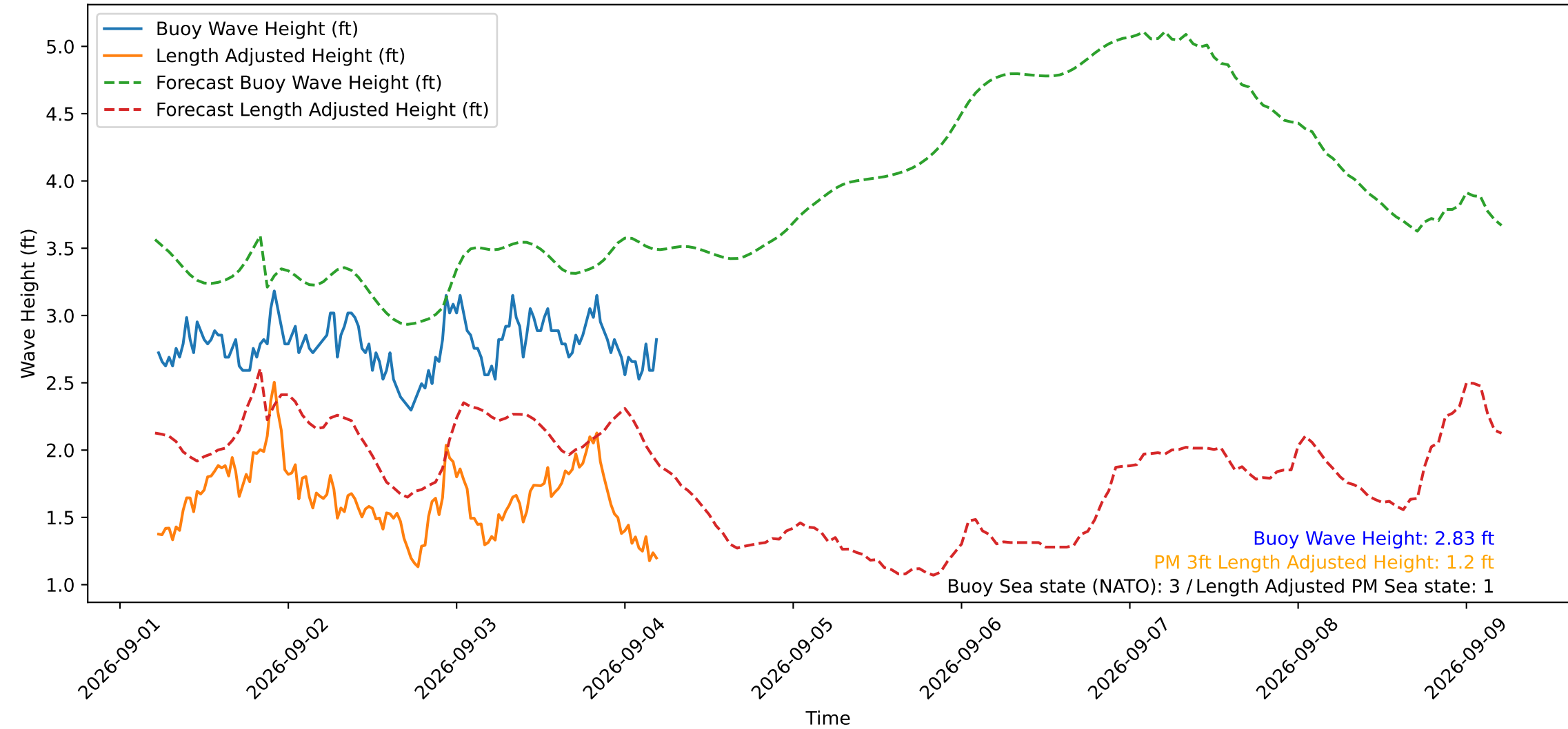
Wave Heights over Time for Red Beach at 2026-09-04 05:20:51
