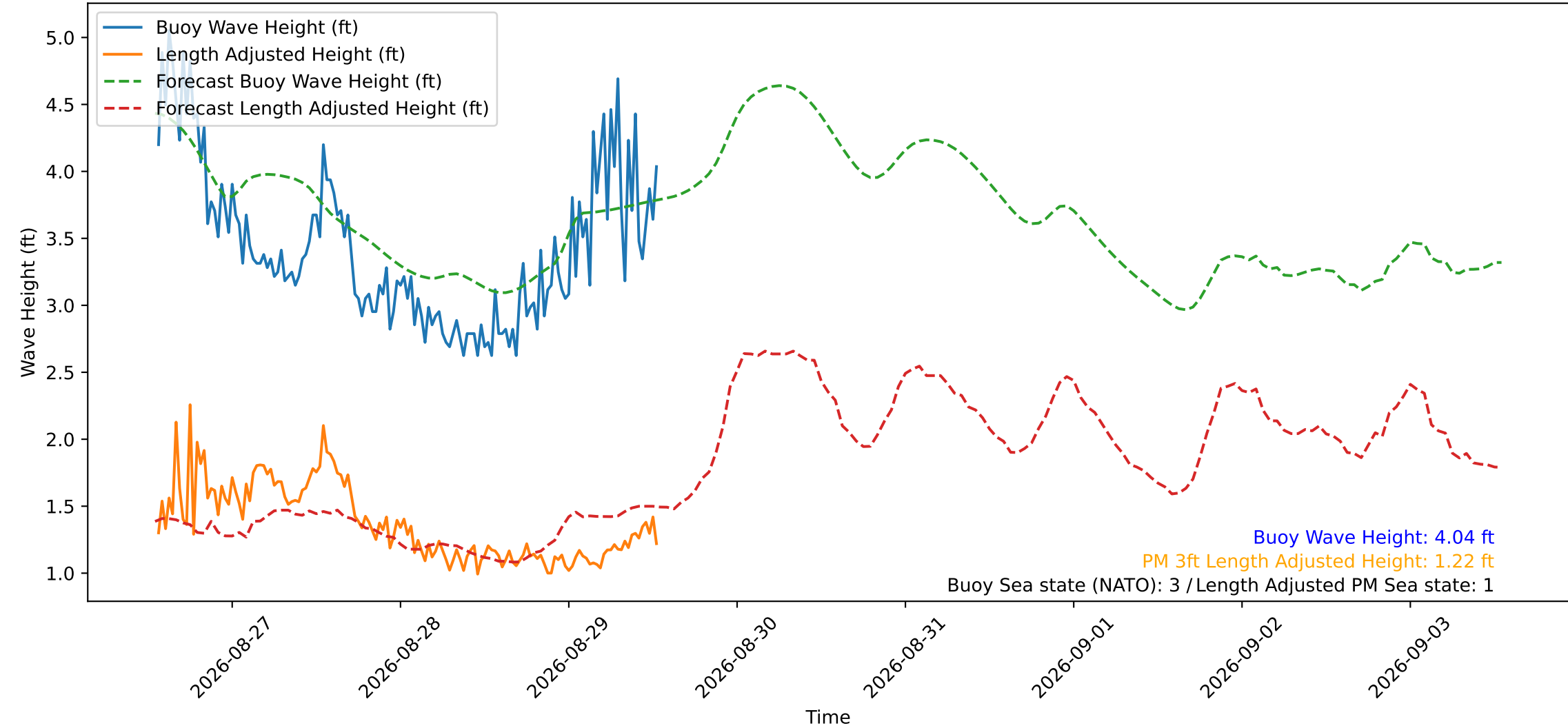
Wave Heights over Time for Red Beach at 2026-08-29 13:20:50
