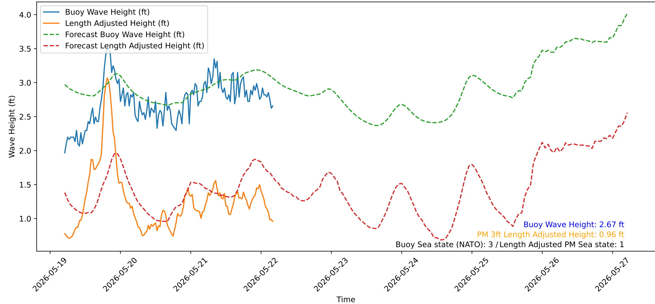
Wave Heights over Time for Red Beach at 2026-05-22 04:50:51
