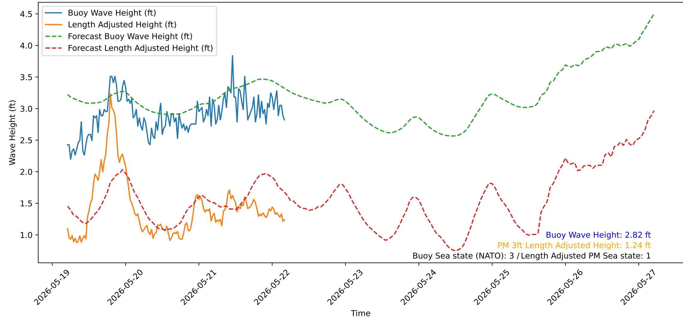
Wave Heights over Time for Oceanside Harbor at 2026-05-22 04:50:31
