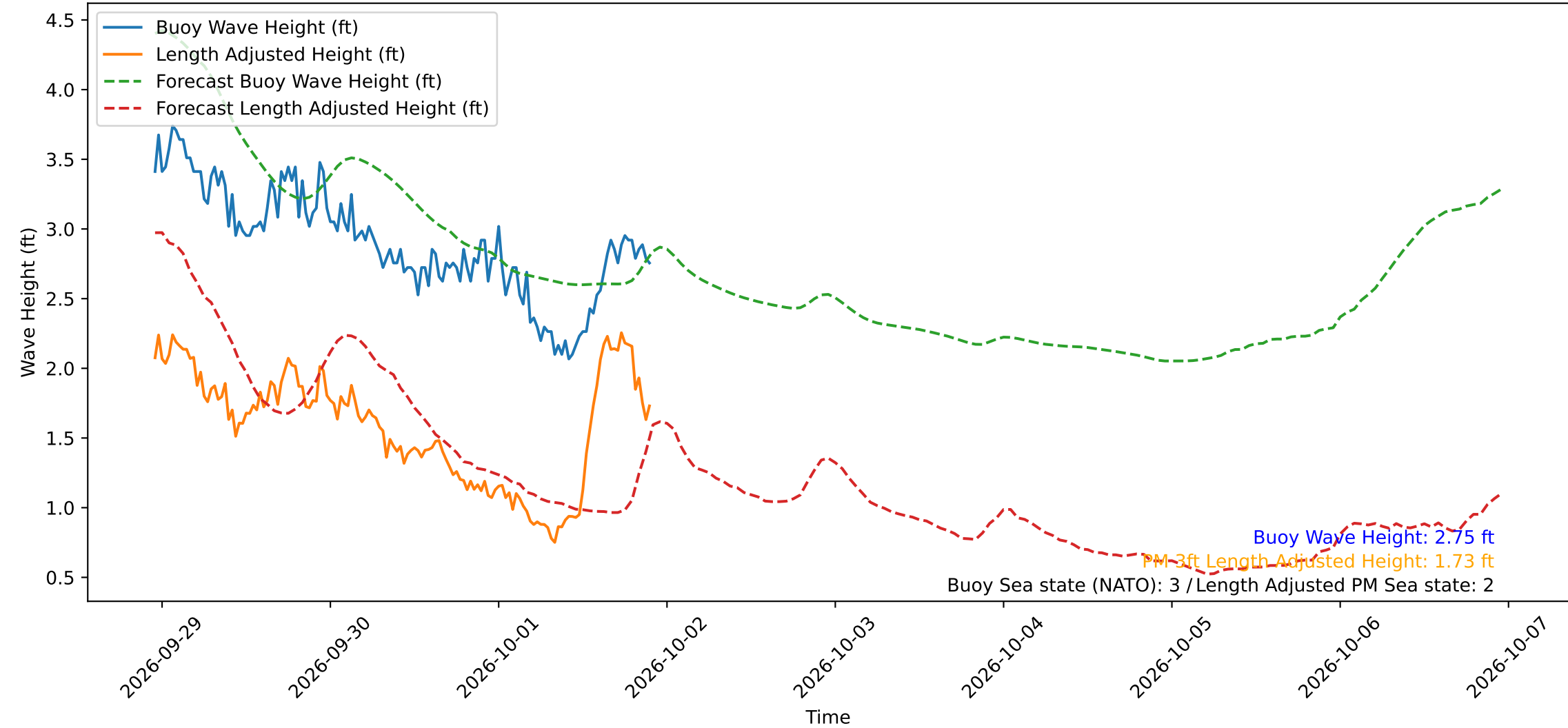
Wave Heights over Time for Red Beach at 2026-10-01 22:30:49
