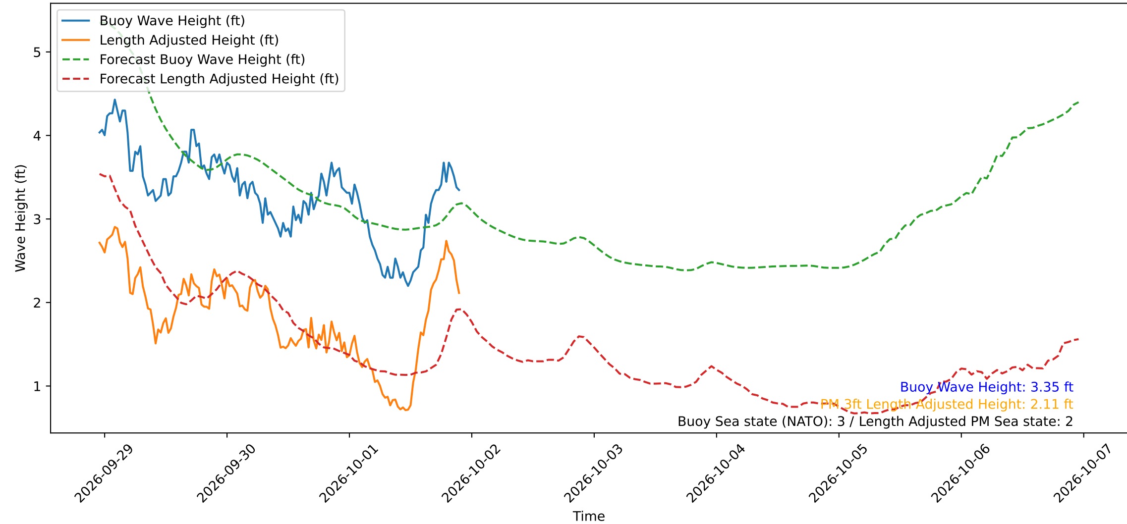
Wave Heights over Time for Green Beach at 2026-10-01 22:31:11
