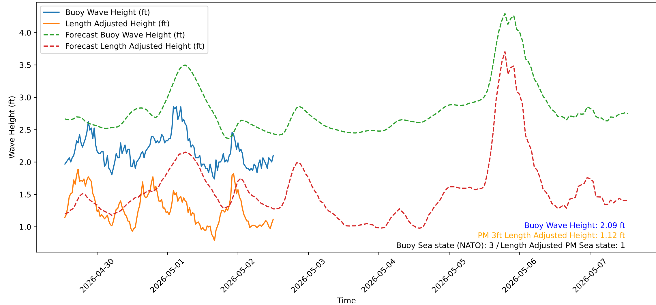
Wave Heights over Time for Green Beach at 2026-05-02 13:01:13
