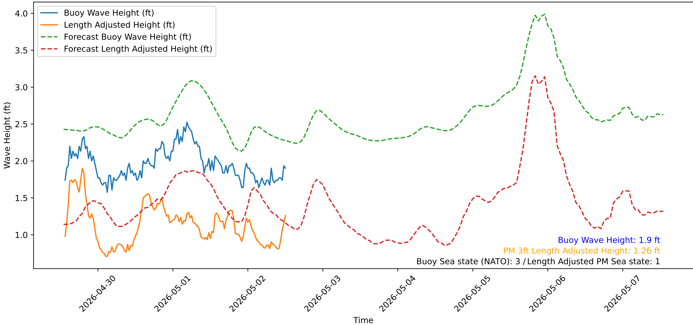
Wave Heights over Time for Red Beach at 2026-05-02 13:00:51
