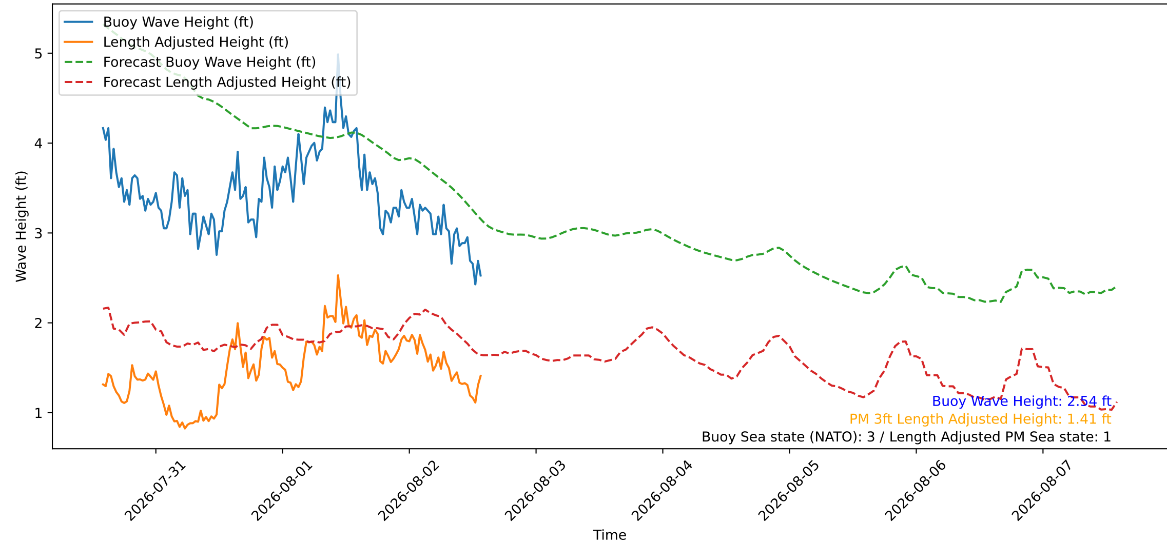
Wave Heights over Time for Green Beach at 2026-08-02 14:11:08
