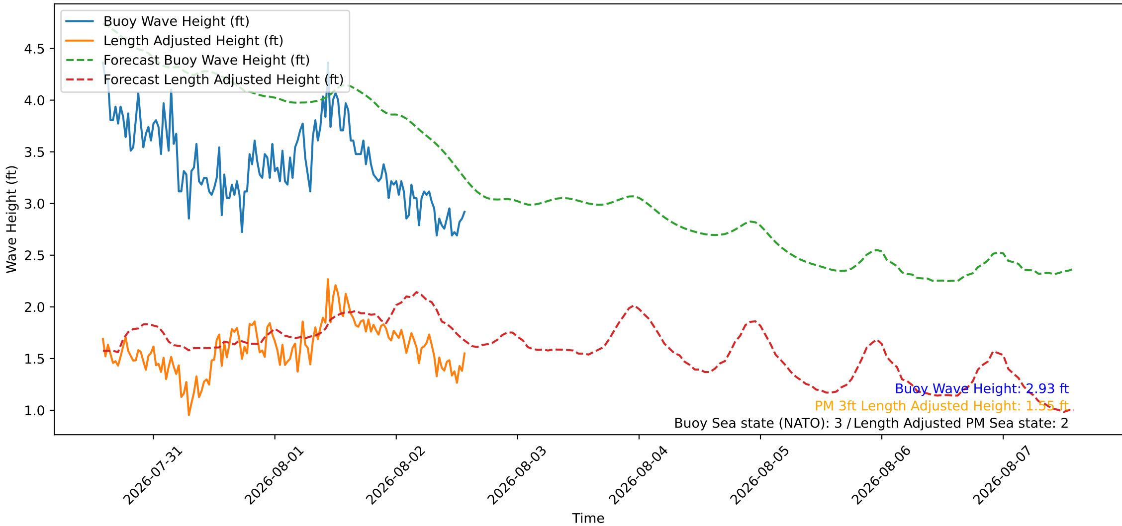
Wave Heights over Time for Oceanside Harbor at 2026-08-02 14:10:26
