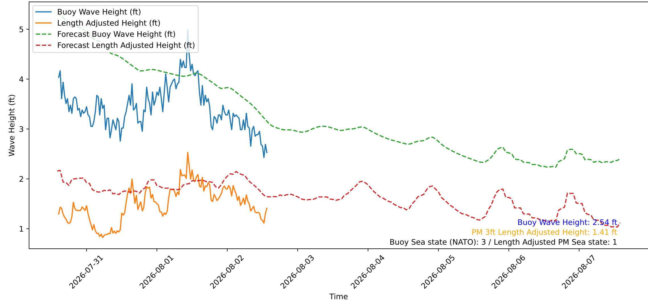
Wave Heights over Time for Green Beach at 2026-08-02 14:21:11
