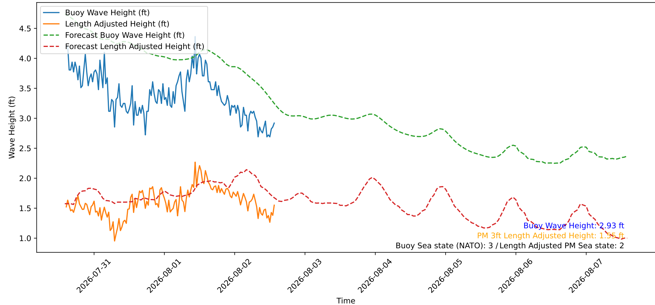
Wave Heights over Time for Oceanside Harbor at 2026-08-02 14:20:27
