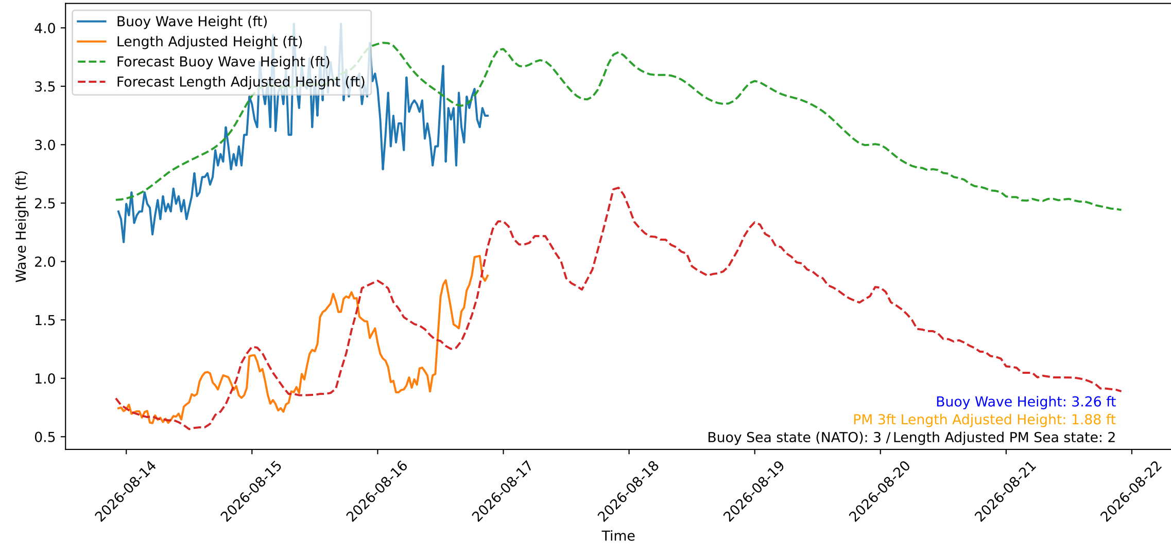
Wave Heights over Time for Red Beach at 2026-08-16 22:00:46
