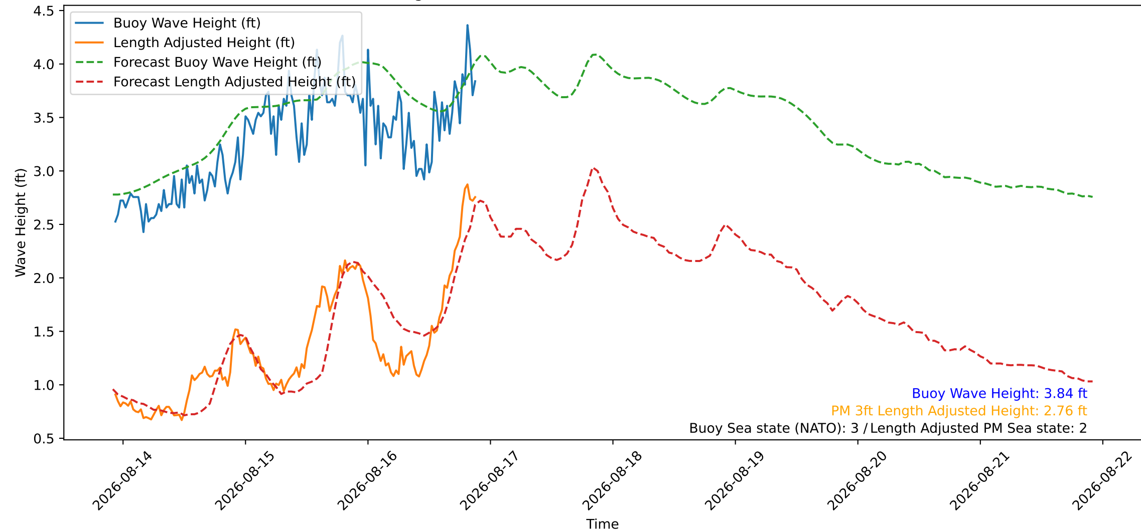
Wave Heights over Time for Green Beach at 2026-08-16 22:01:08
