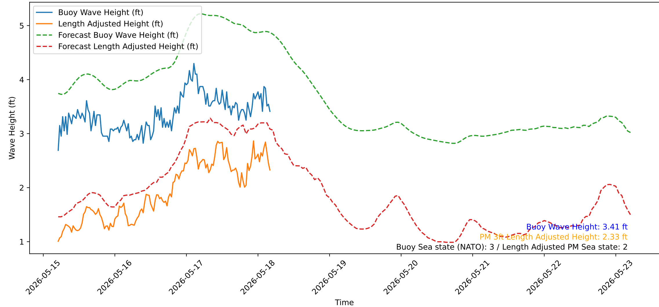
Wave Heights over Time for Oceanside Harbor at 2026-05-18 05:00:30
