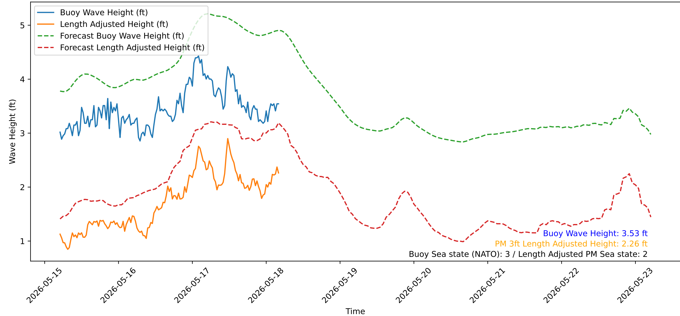
Wave Heights over Time for Green Beach at 2026-05-18 05:01:12
