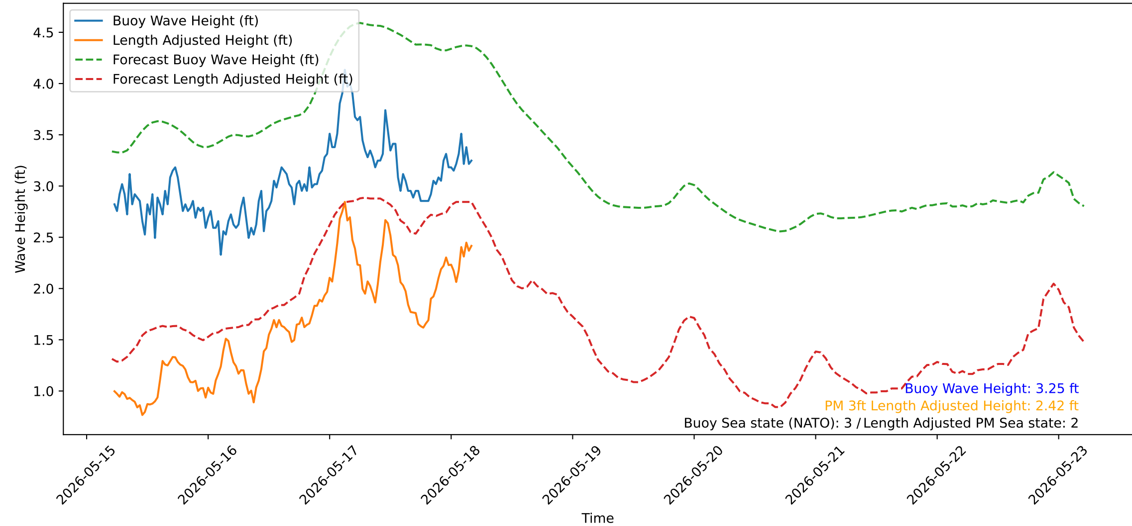
Wave Heights over Time for Red Beach at 2026-05-18 05:00:50
