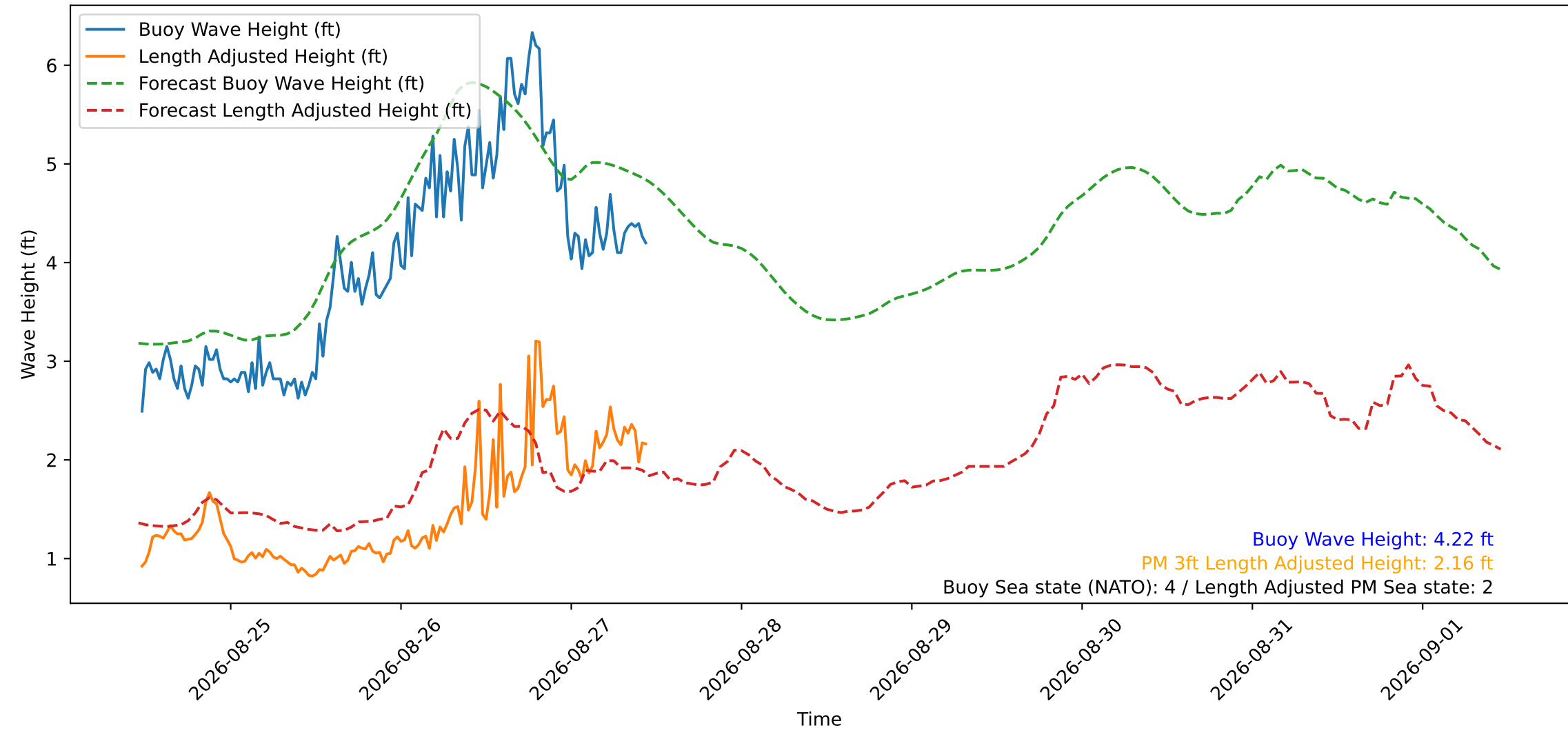
Wave Heights over Time for Green Beach at 2026-08-27 11:21:15
