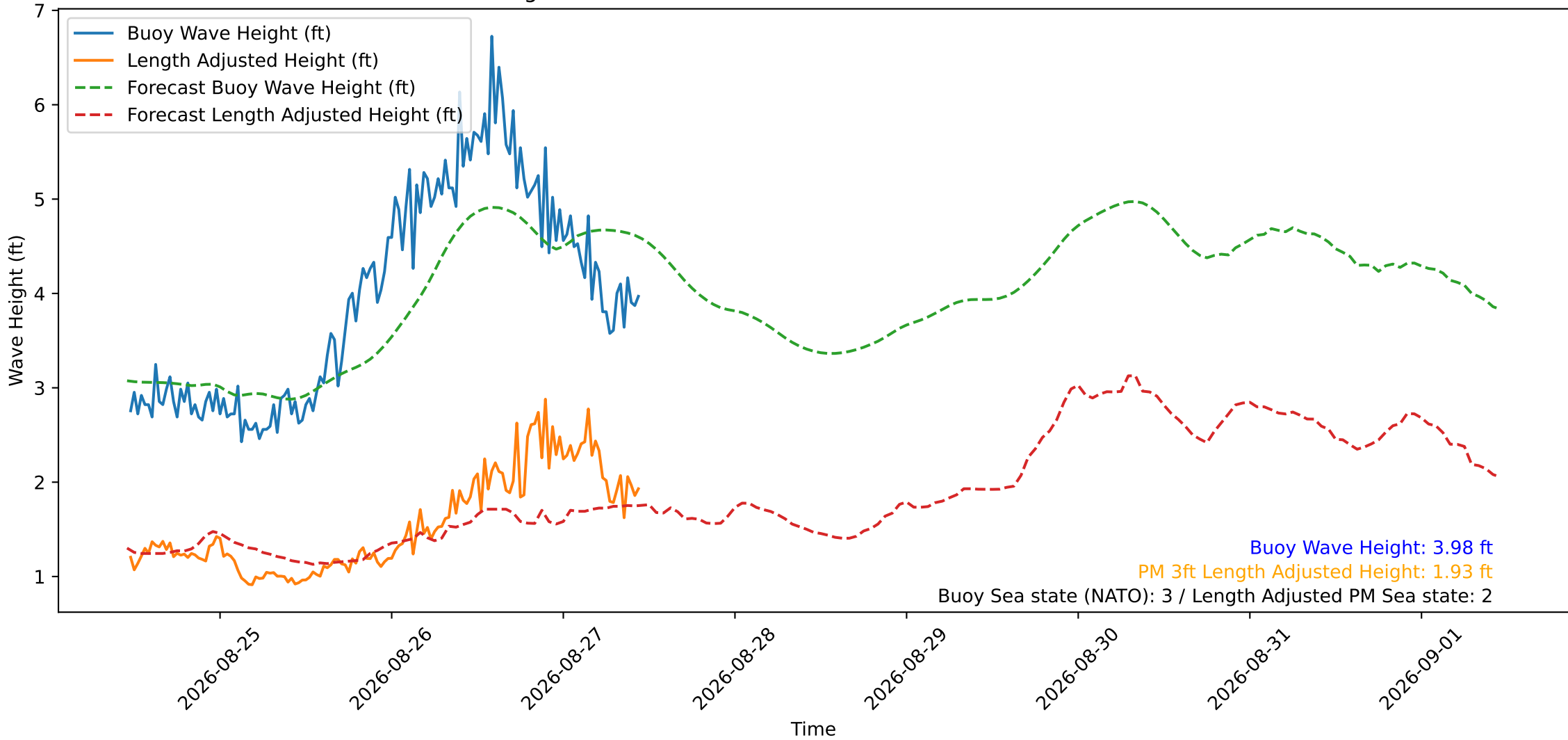
Wave Heights over Time for Oceanside Harbor at 2026-08-27 11:20:30
