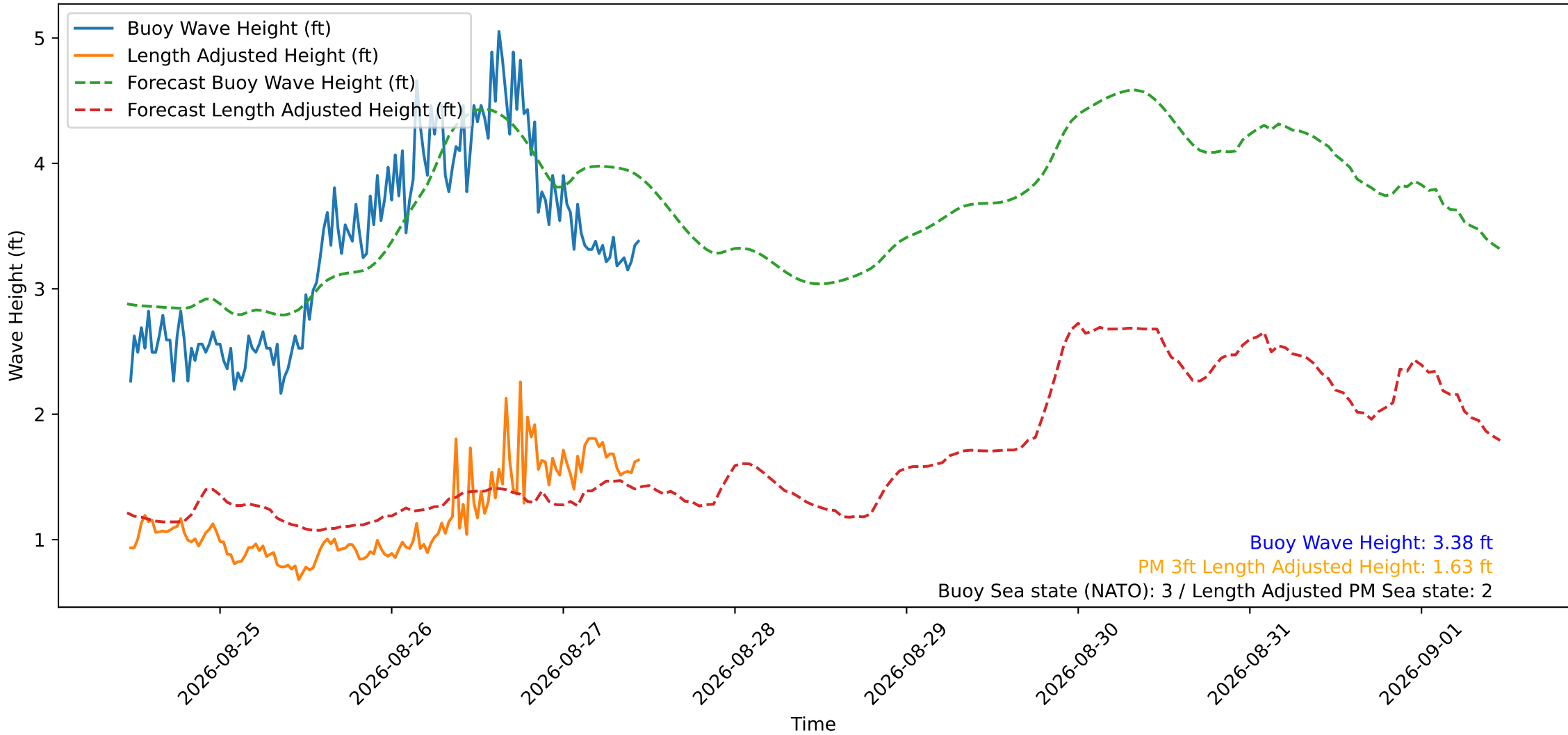
Wave Heights over Time for Red Beach at 2026-08-27 11:20:51
