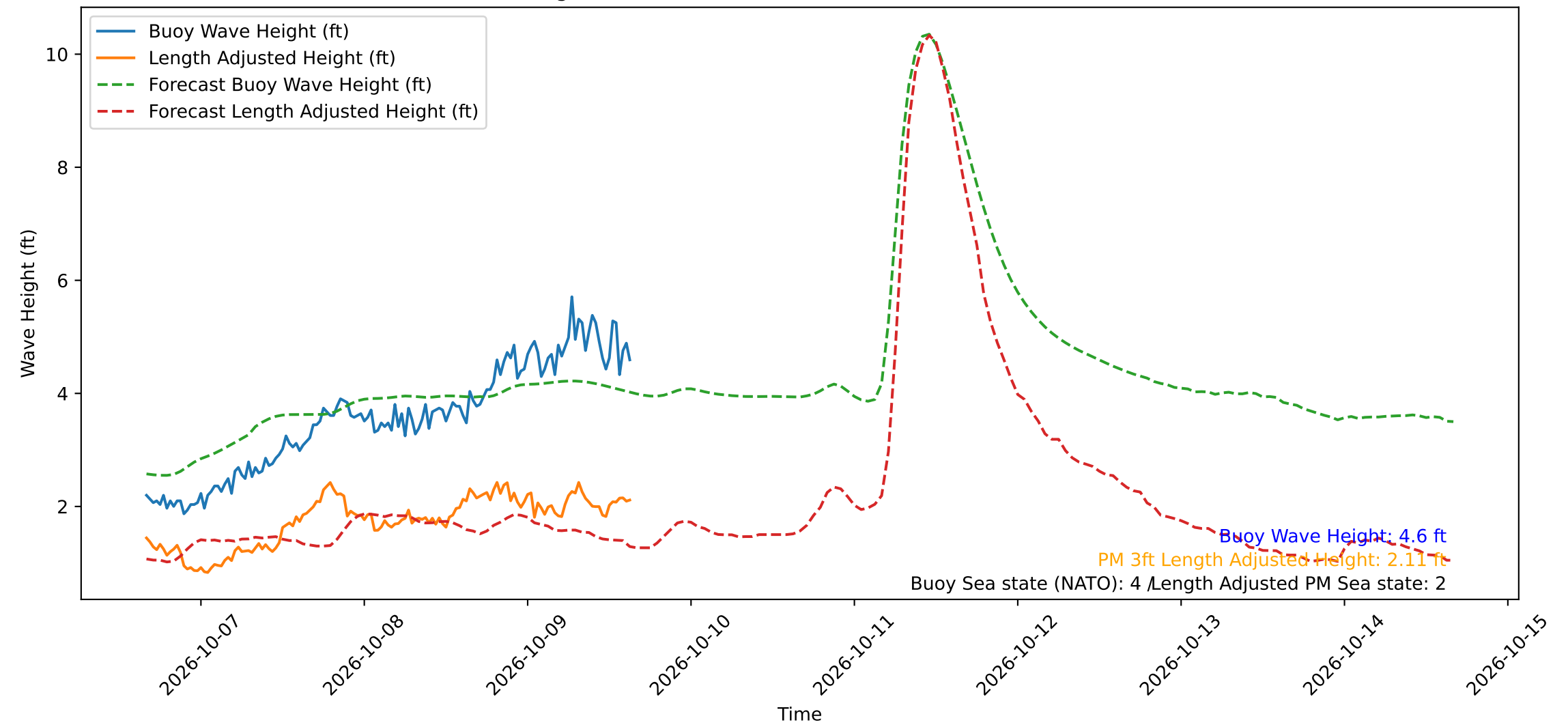
Wave Heights over Time for Red Beach at 2026-10-09 15:40:49
