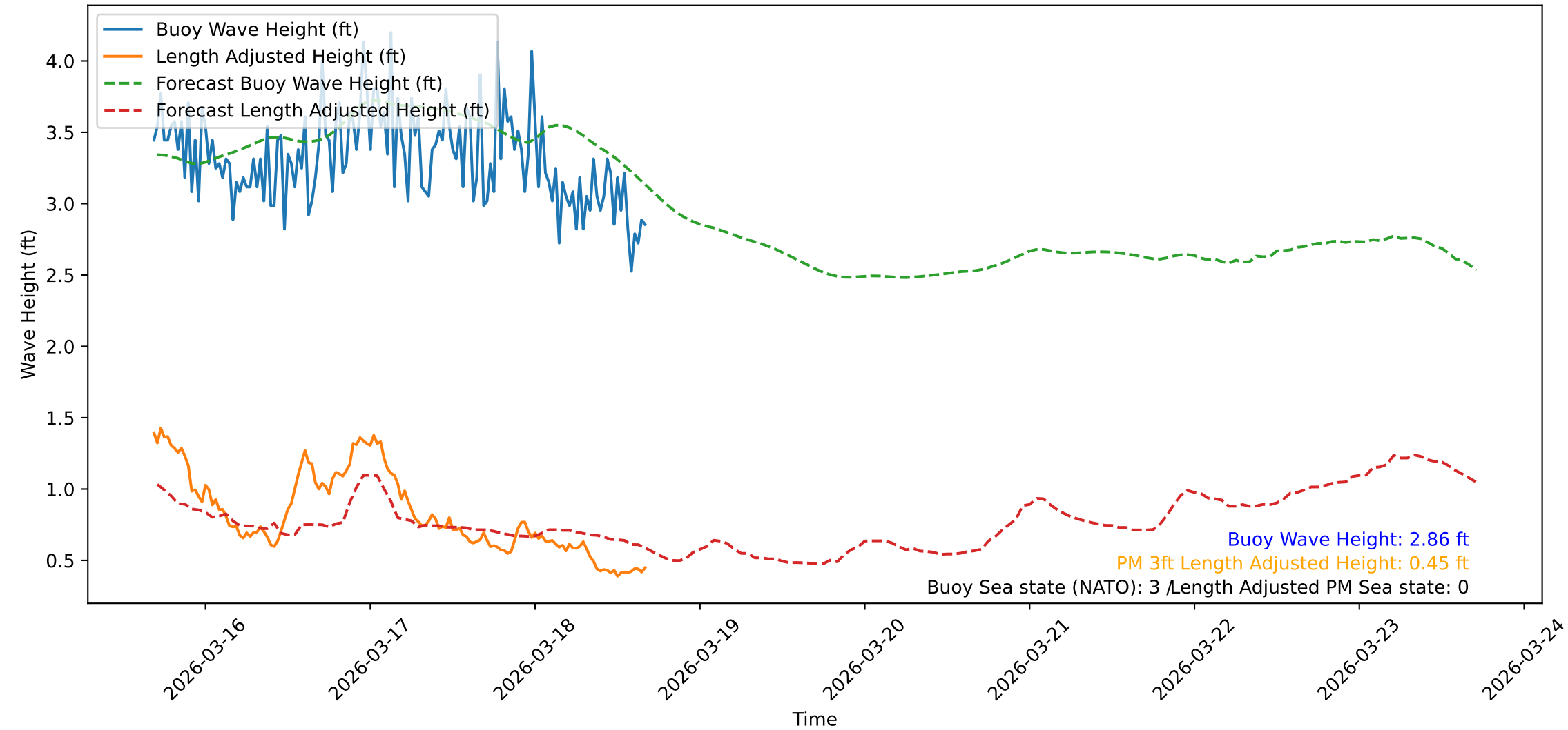
Wave Heights over Time for Green Beach at 2026-03-18 16:41:10
