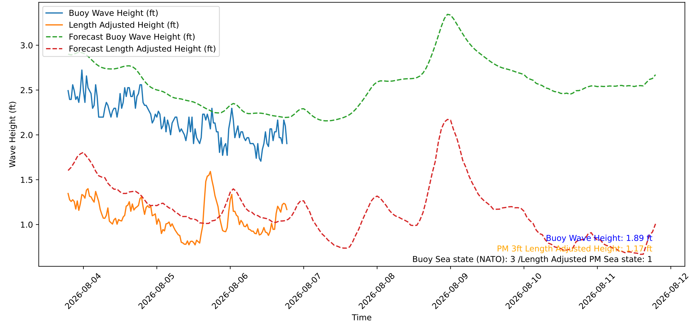
Wave Heights over Time for Oceanside Harbor at 2026-08-06 19:10:26
