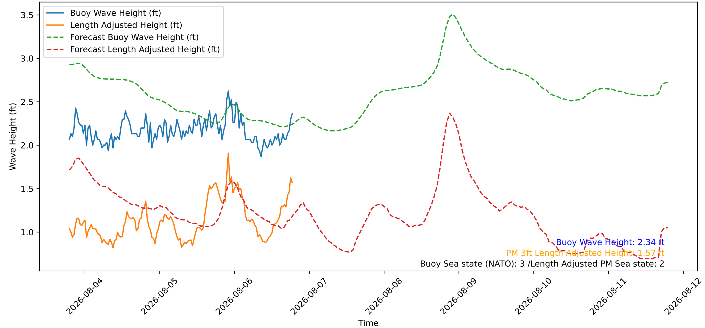
Wave Heights over Time for Green Beach at 2026-08-06 19:11:08
