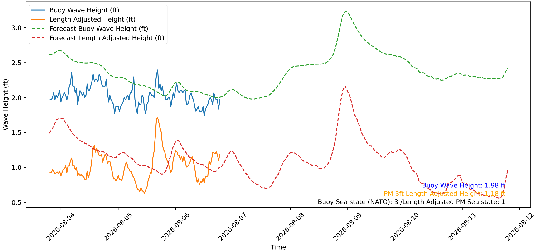
Wave Heights over Time for Red Beach at 2026-08-06 19:10:45
