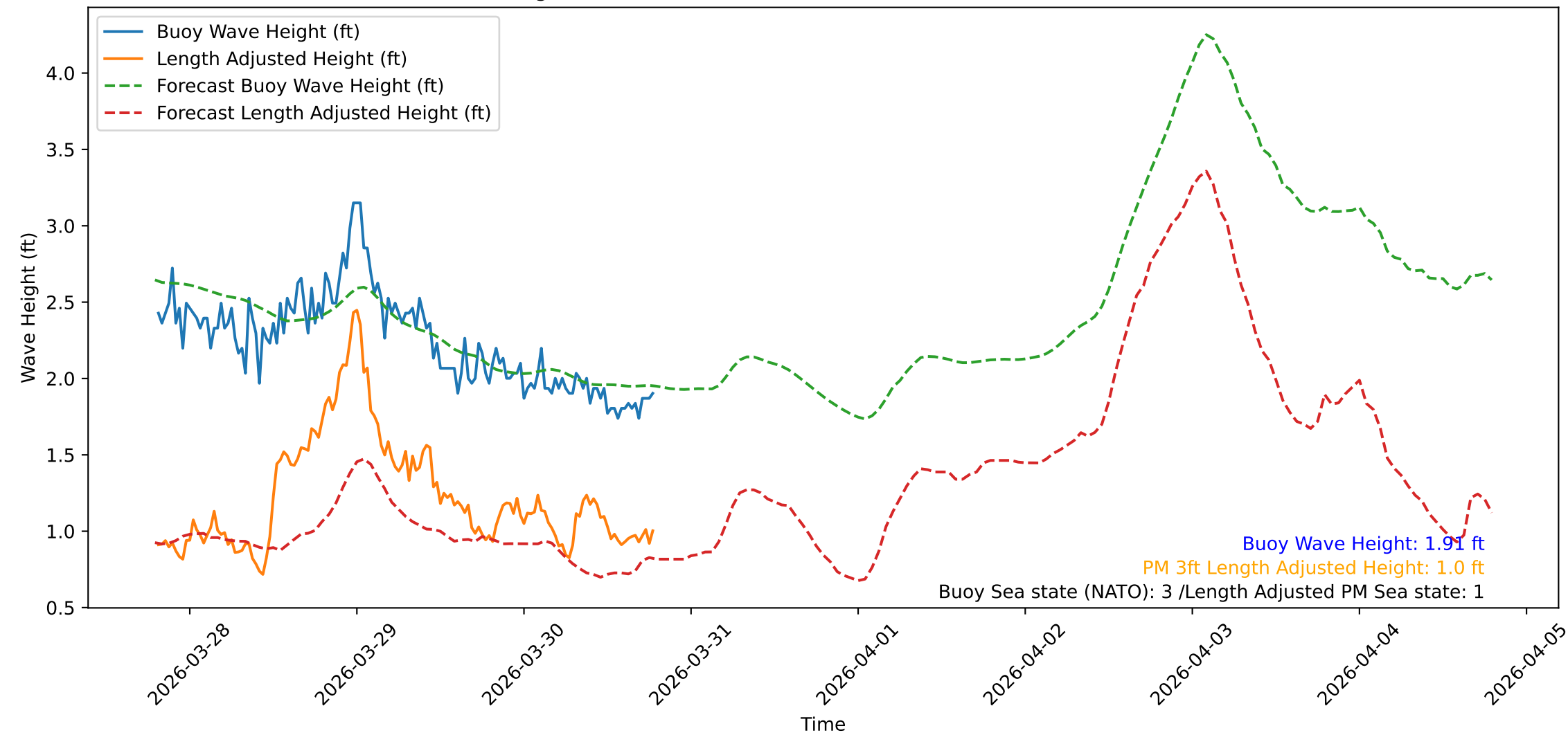
Wave Heights over Time for Oceanside Harbor at 2026-03-30 19:20:31
