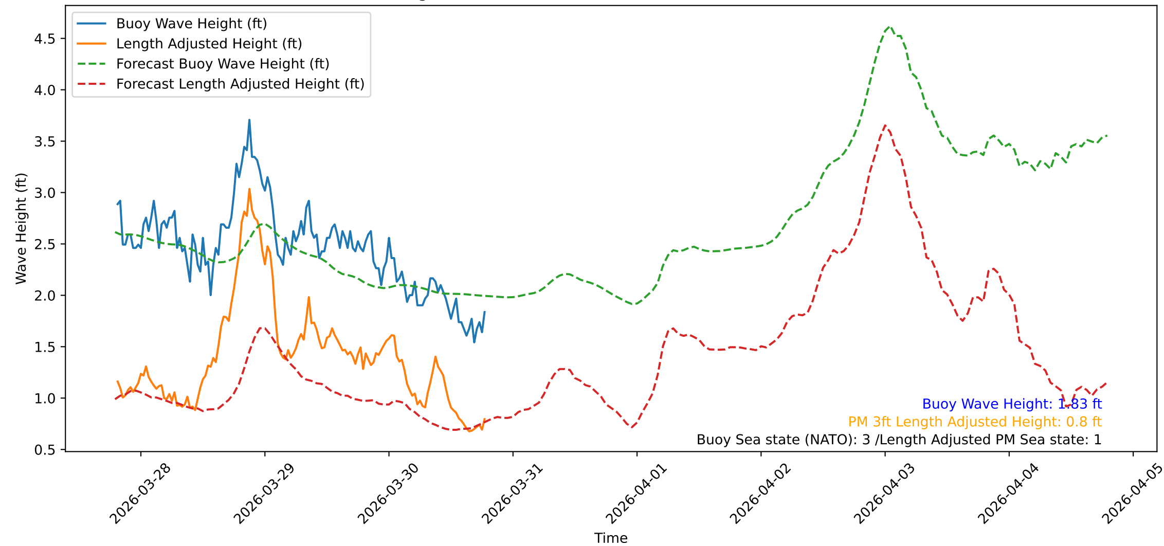
Wave Heights over Time for Green Beach at 2026-03-30 19:21:10
