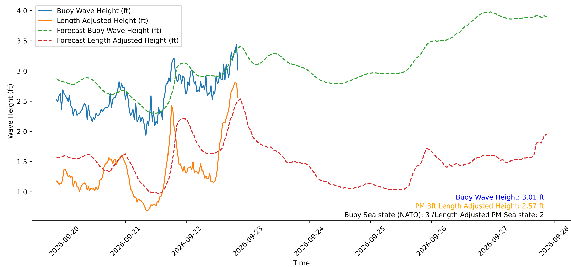
Wave Heights over Time for Green Beach at 2026-09-22 20:51:13
