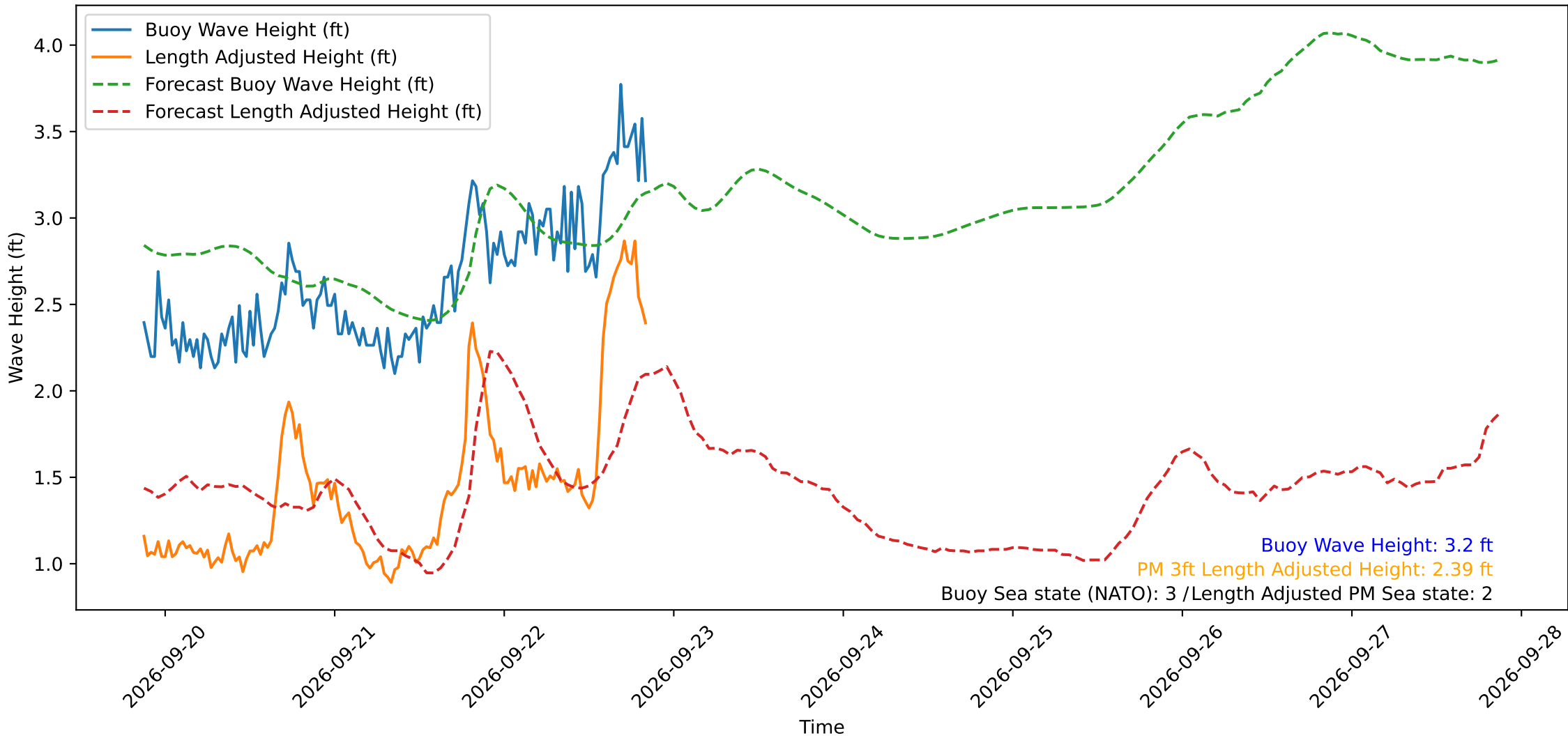
Wave Heights over Time for Oceanside Harbor at 2026-09-22 20:50:29
