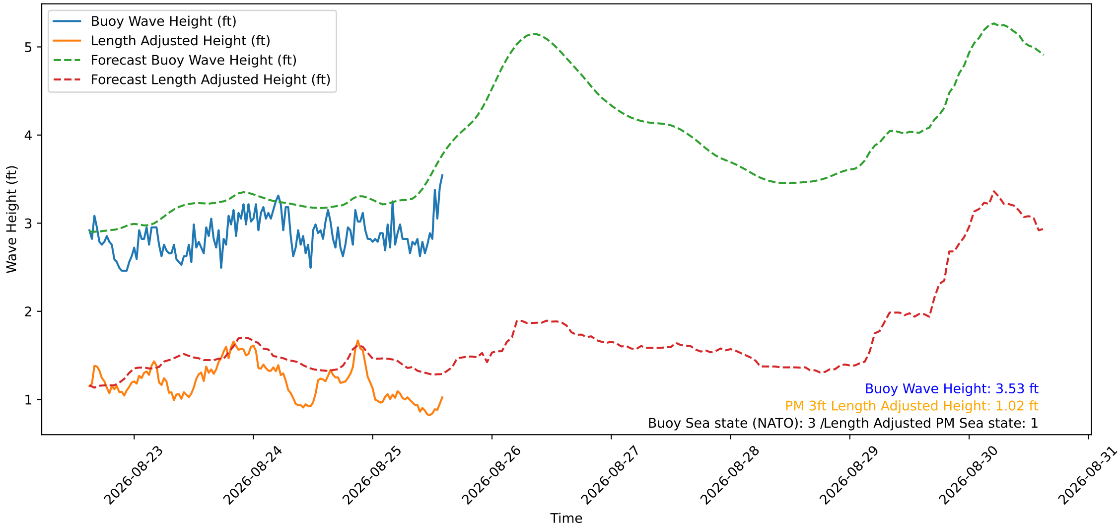
Wave Heights over Time for Green Beach at 2026-08-25 14:41:12
