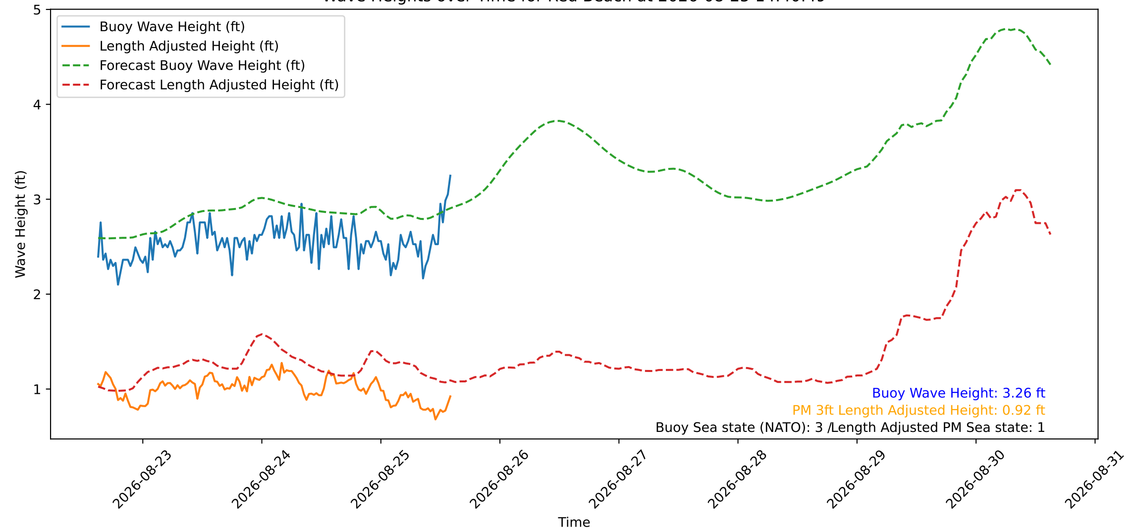
Wave Heights over Time for Red Beach at 2026-08-25 14:40:49
