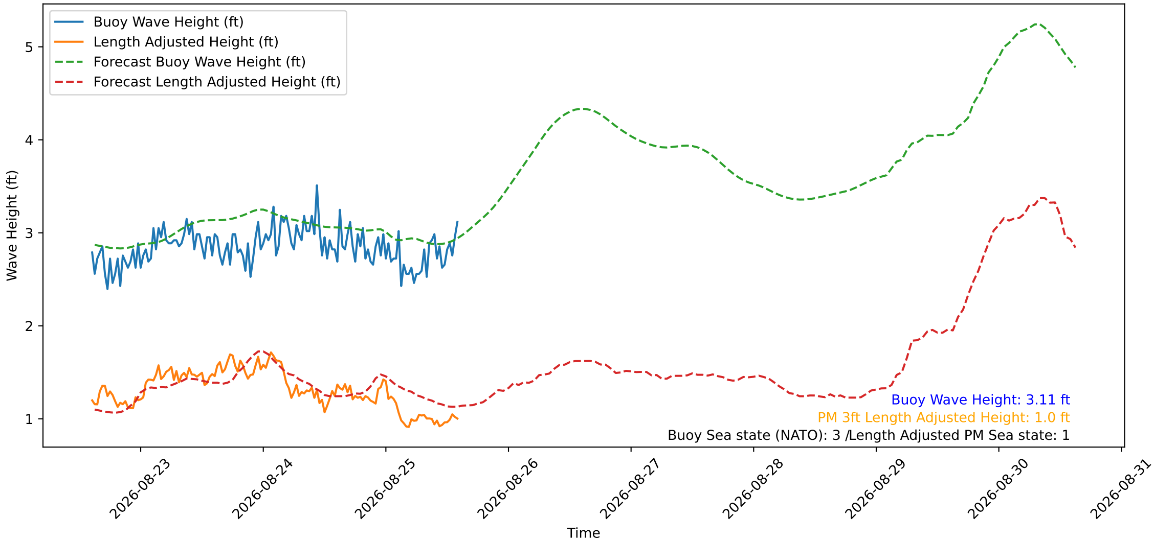
Wave Heights over Time for Oceanside Harbor at 2026-08-25 14:40:29
