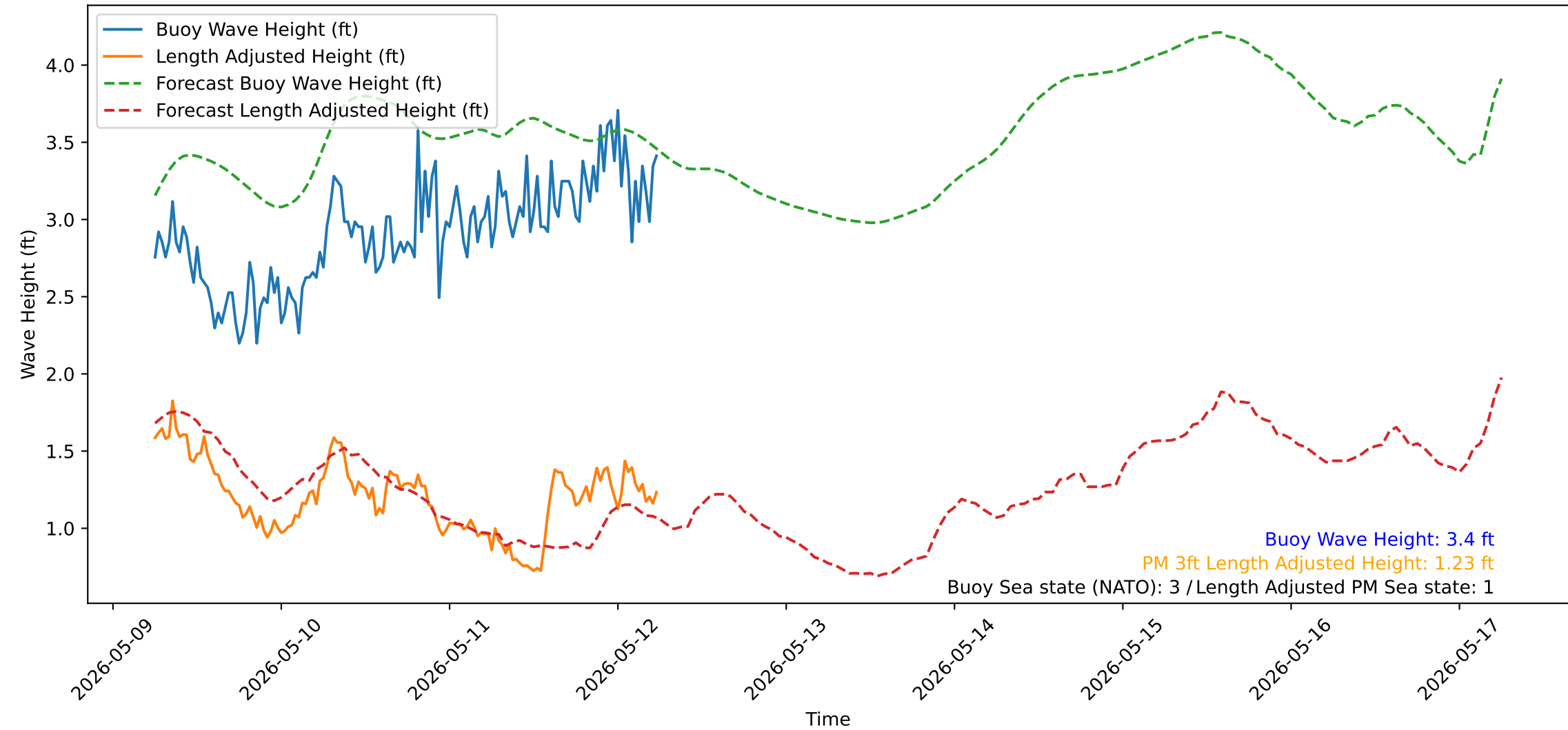
Wave Heights over Time for Oceanside Harbor at 2026-05-12 06:10:31
