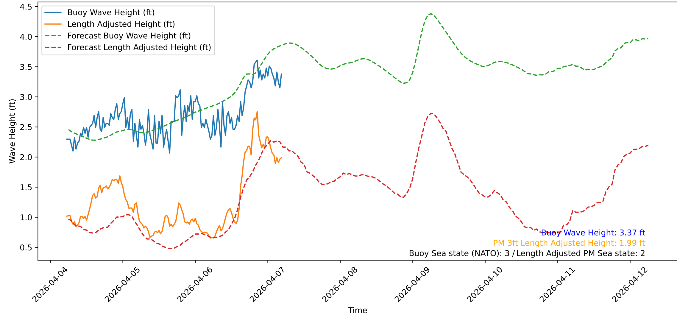
Wave Heights over Time for Oceanside Harbor at 2026-04-07 05:30:31
