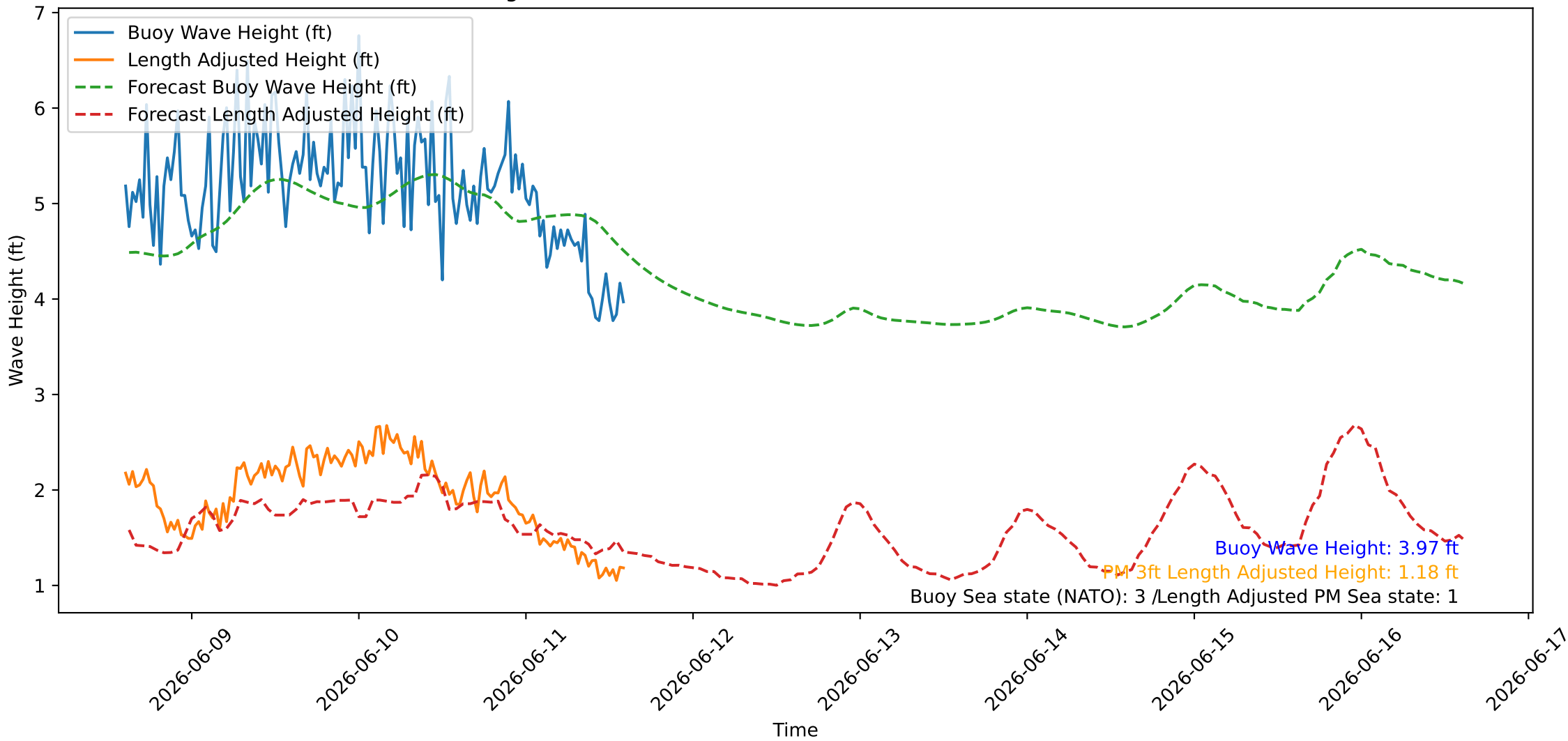
Wave Heights over Time for Oceanside Harbor at 2026-06-11 14:40:26
