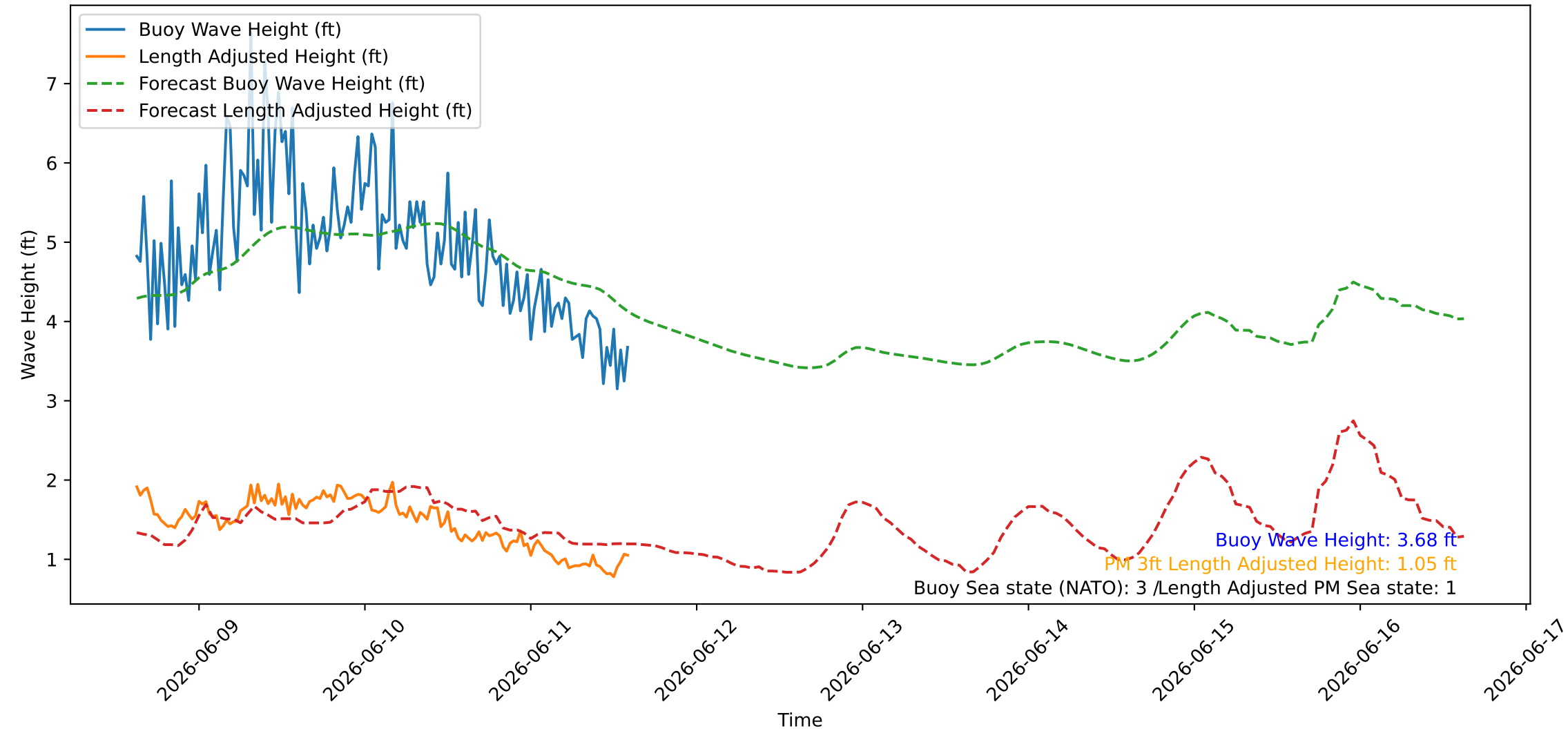
Wave Heights over Time for Red Beach at 2026-06-11 14:40:46
