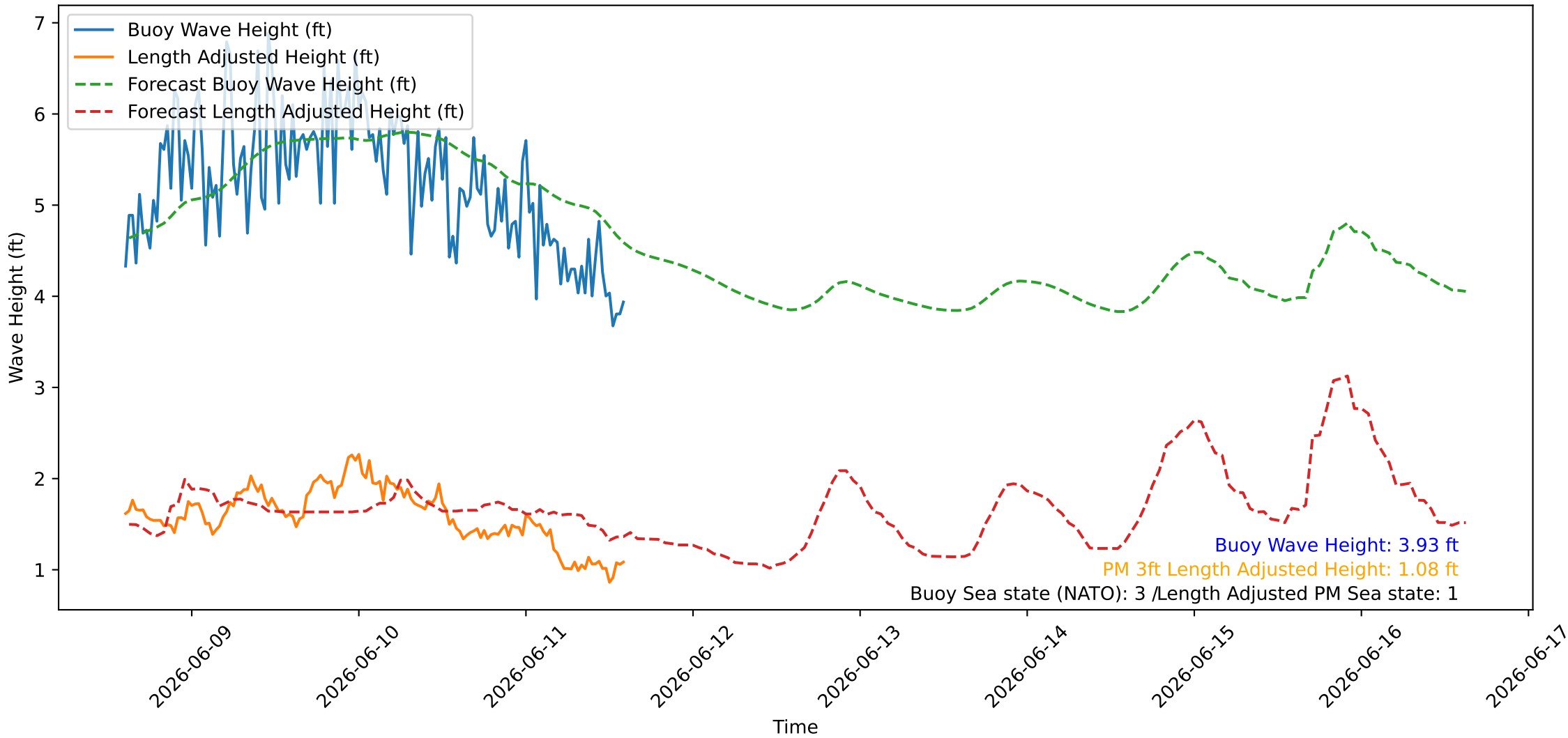
Wave Heights over Time for Green Beach at 2026-06-11 14:41:09
