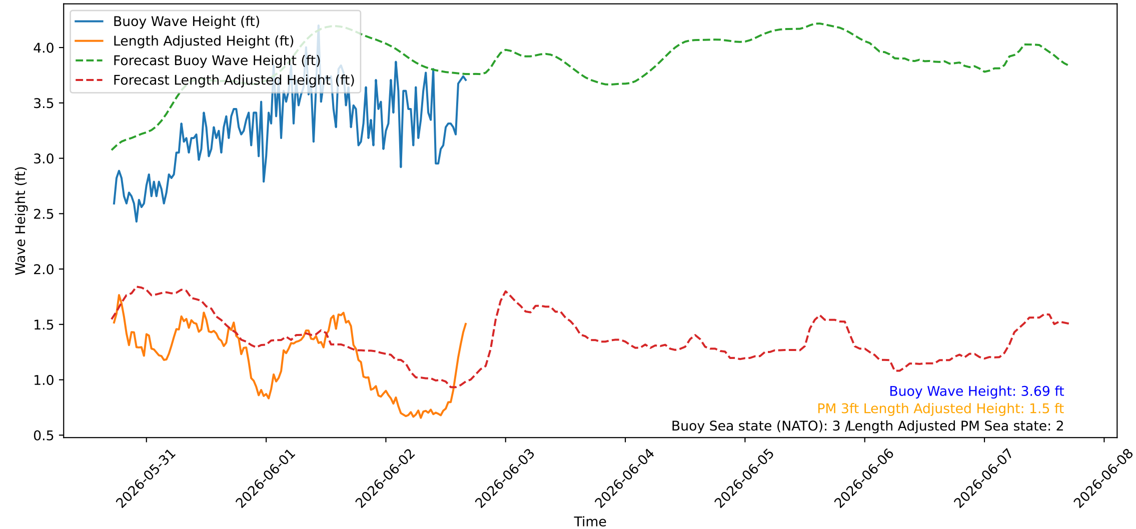
Wave Heights over Time for Red Beach at 2026-06-02 17:00:44
