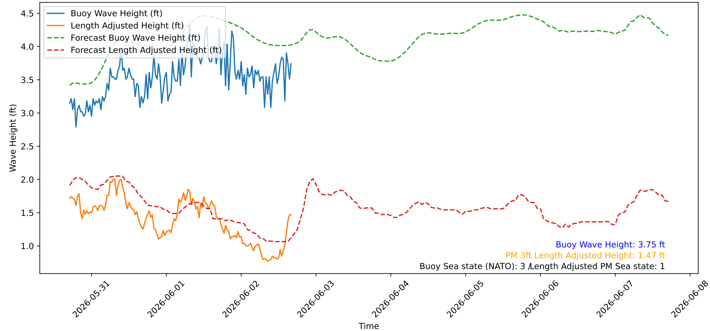
Wave Heights over Time for Green Beach at 2026-06-02 17:01:07
