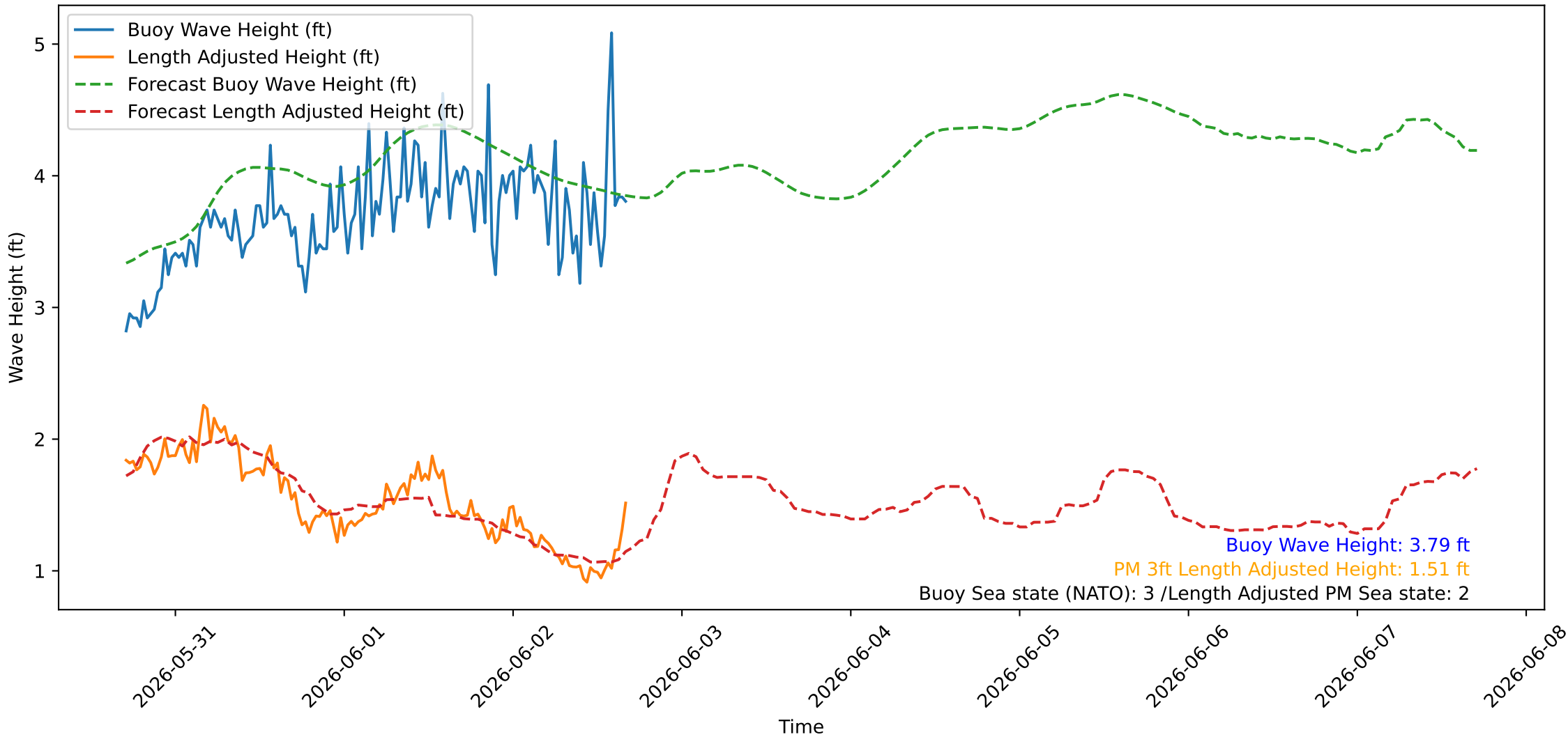
Wave Heights over Time for Oceanside Harbor at 2026-06-02 17:00:25
