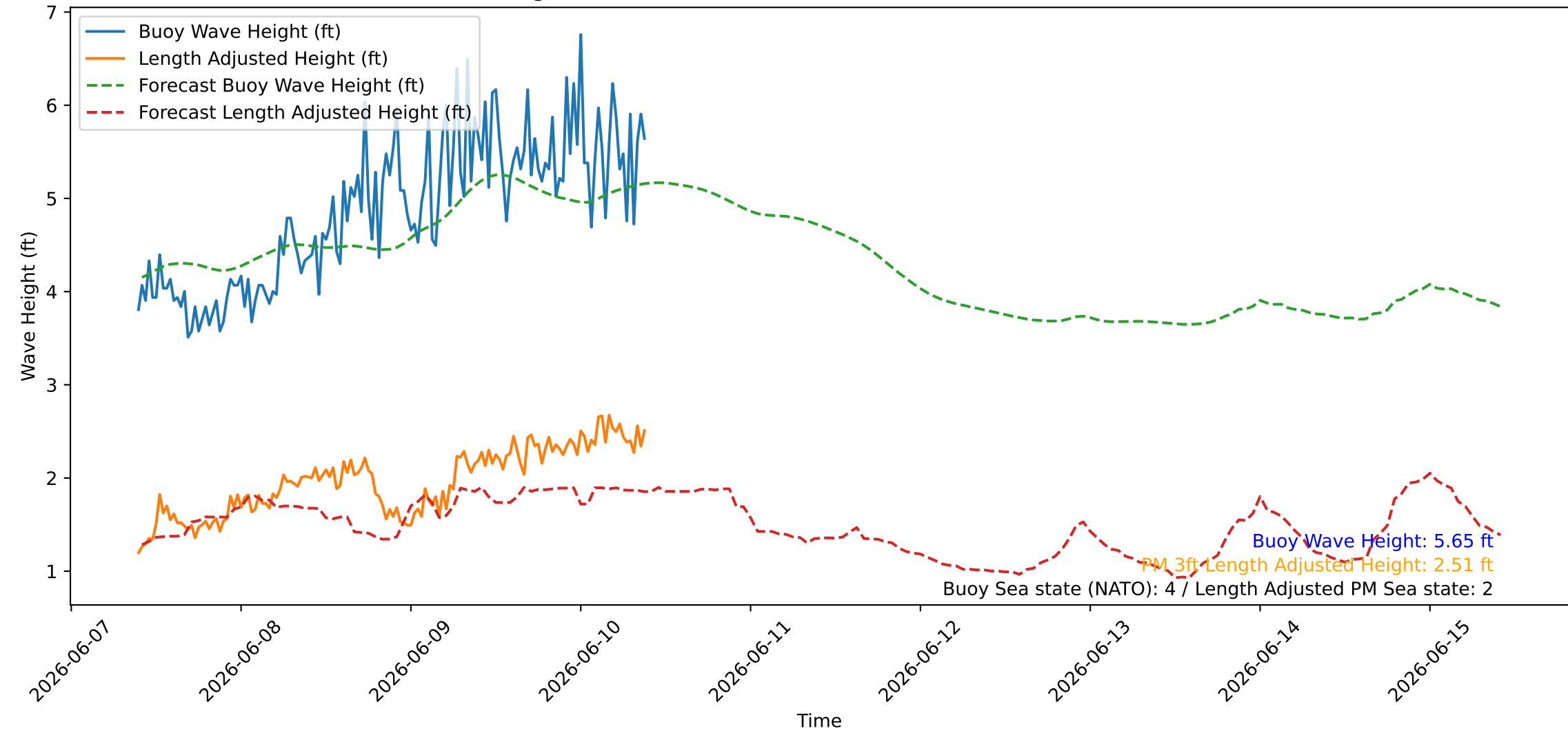
Wave Heights over Time for Oceanside Harbor at 2026-06-10 09:30:26
