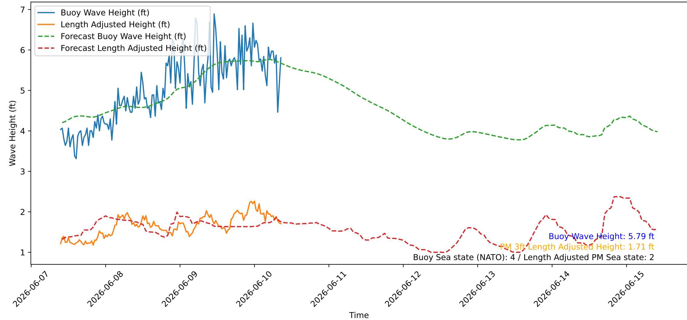
Wave Heights over Time for Green Beach at 2026-06-10 09:31:10
