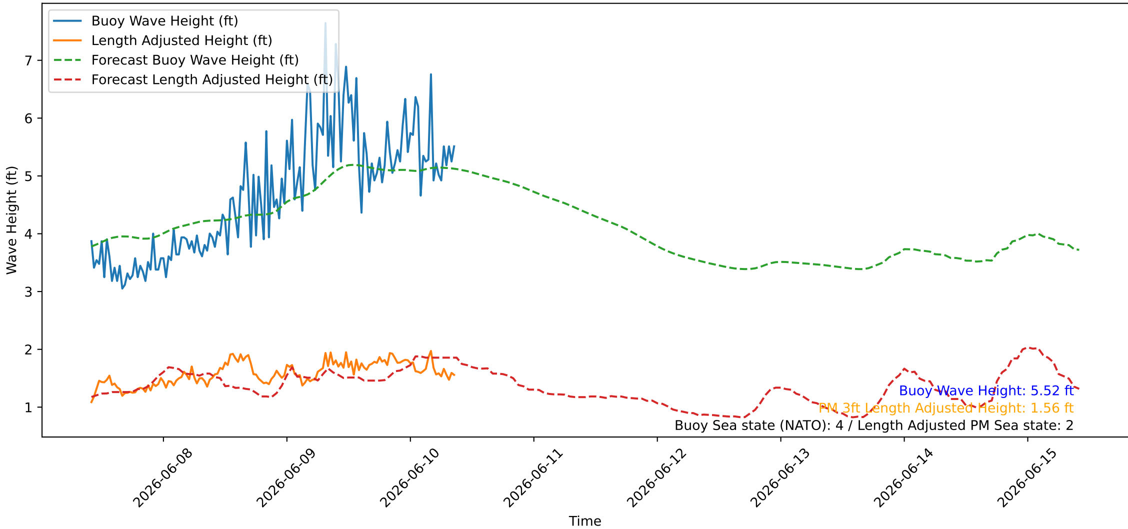
Wave Heights over Time for Red Beach at 2026-06-10 09:30:46
