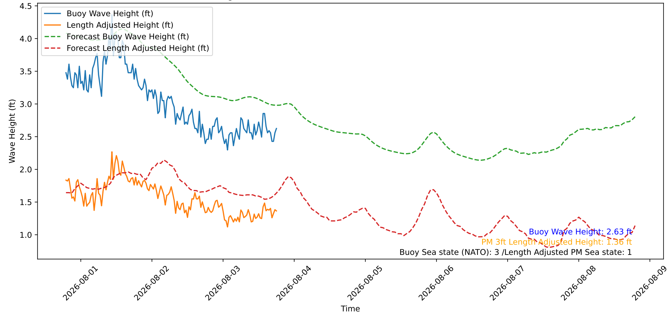
Wave Heights over Time for Oceanside Harbor at 2026-08-03 19:00:27
