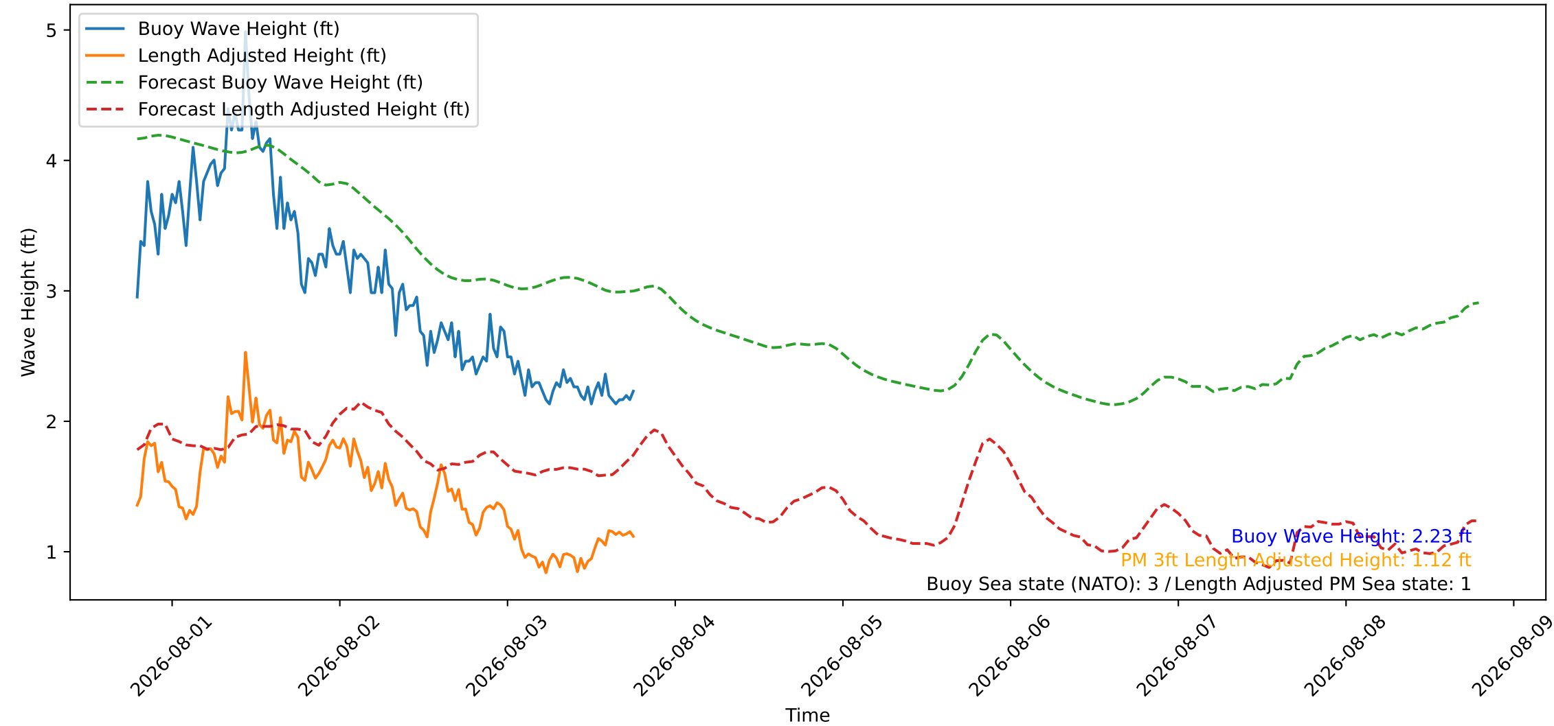
Wave Heights over Time for Green Beach at 2026-08-03 19:01:08
