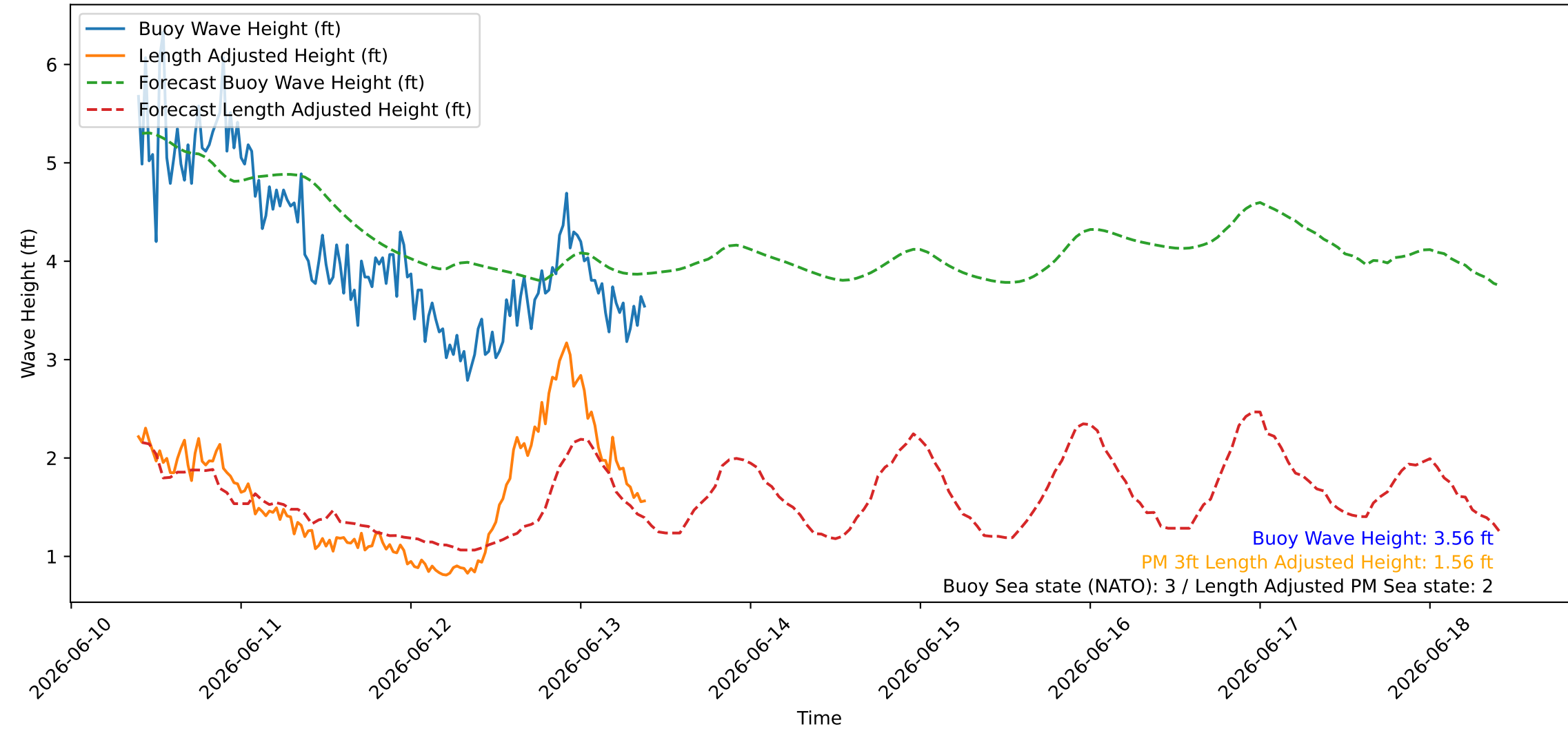
Wave Heights over Time for Oceanside Harbor at 2026-06-13 09:40:27
