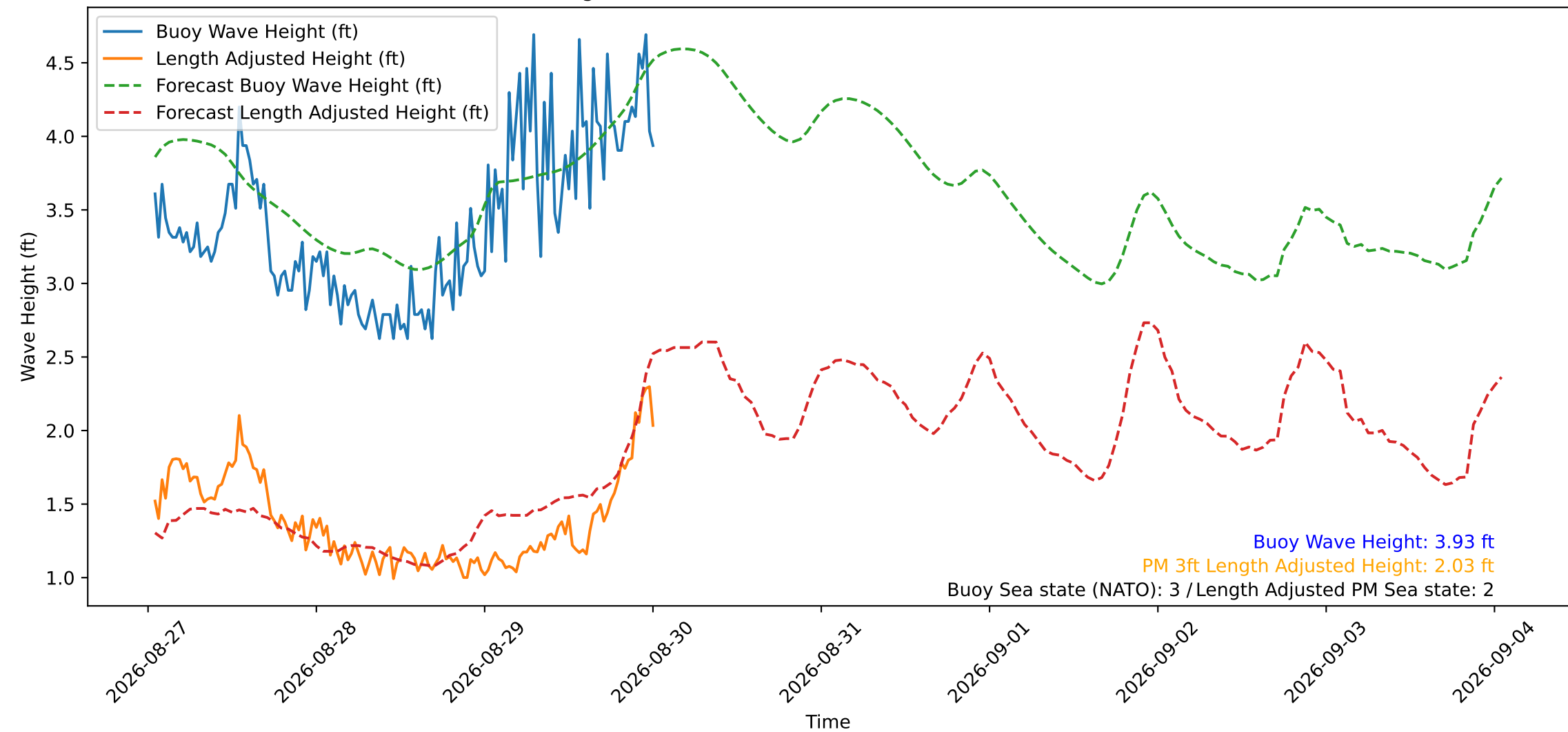
Wave Heights over Time for Red Beach at 2026-08-30 00:40:50
