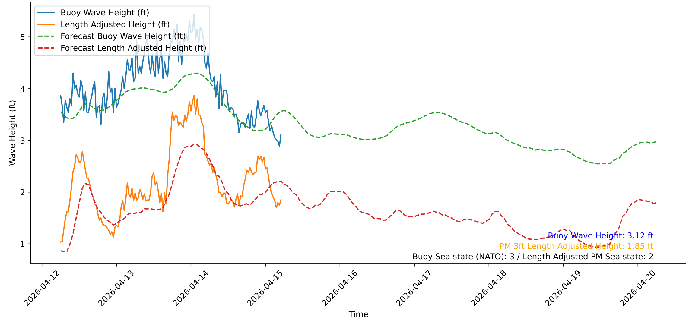
Wave Heights over Time for Oceanside Harbor at 2026-04-15 05:50:31
