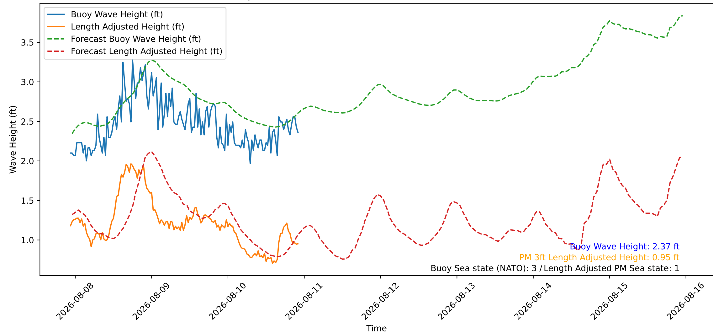
Wave Heights over Time for Oceanside Harbor at 2026-08-10 22:40:26
