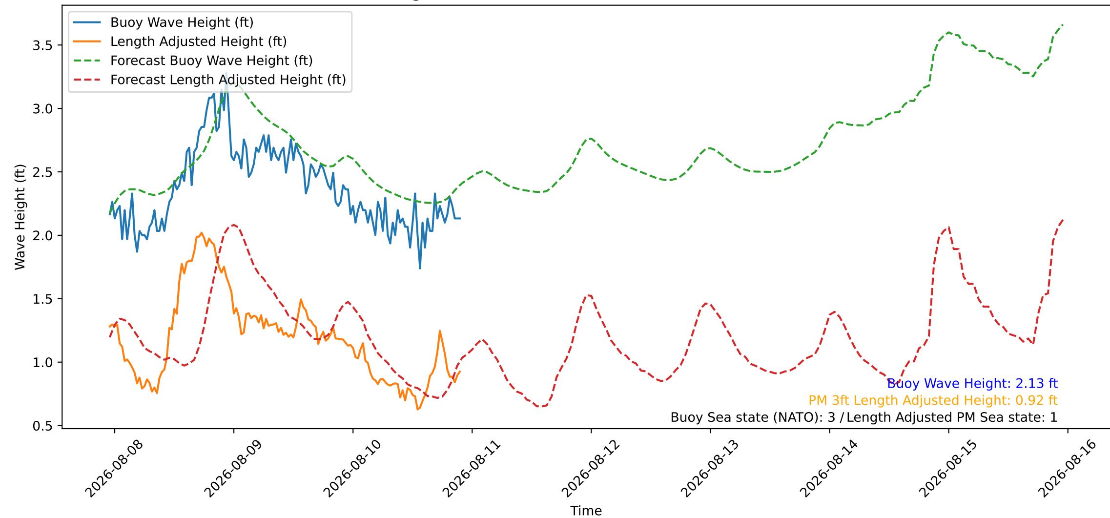
Wave Heights over Time for Red Beach at 2026-08-10 22:40:46
