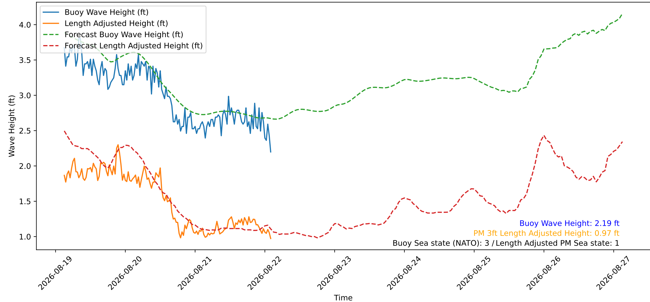
Wave Heights over Time for Oceanside Harbor at 2026-08-22 03:10:30
