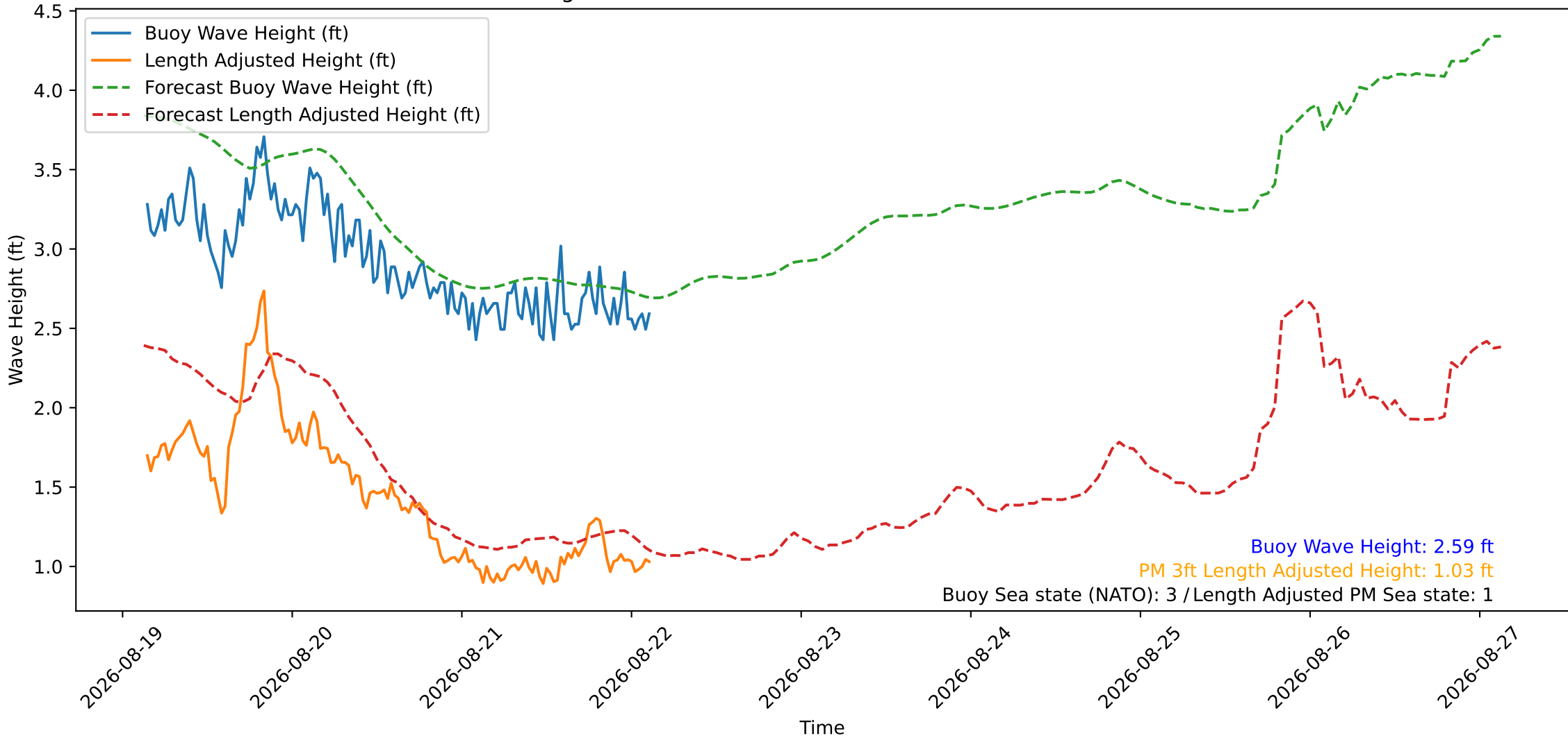
Wave Heights over Time for Green Beach at 2026-08-22 03:11:12
