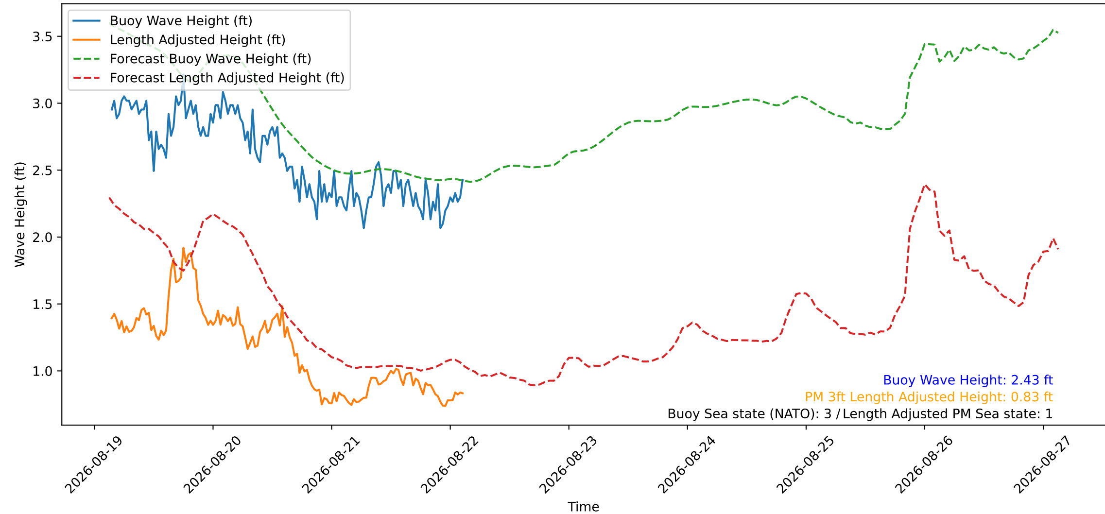
Wave Heights over Time for Red Beach at 2026-08-22 03:10:49
